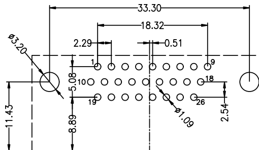
Recommended P.C.B Layout Top View Tolerance: ±0.05mm
