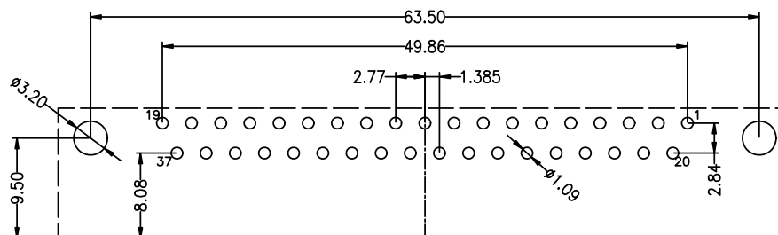
PCB LAYOUT
