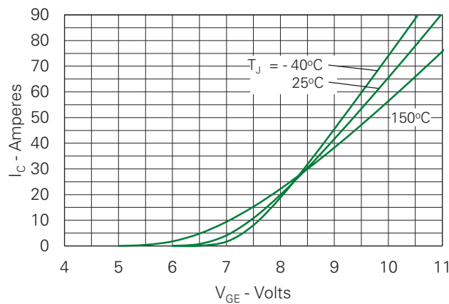
Fig. 6. Input Admittance
