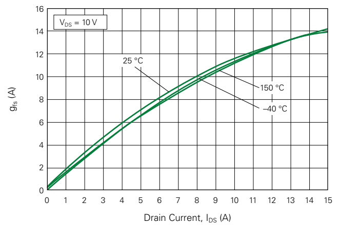
Fig. 2. Typical Transconductance
