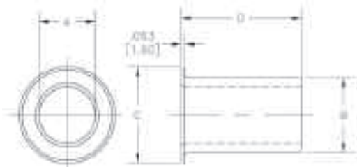
MS 3420-XX
