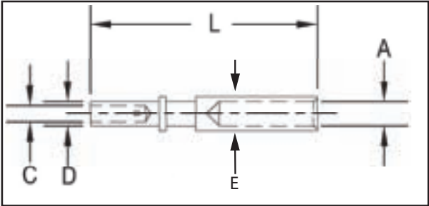
Female (Socket)
