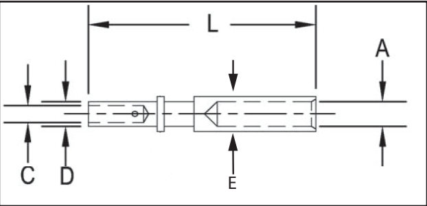
Female (Socket)
