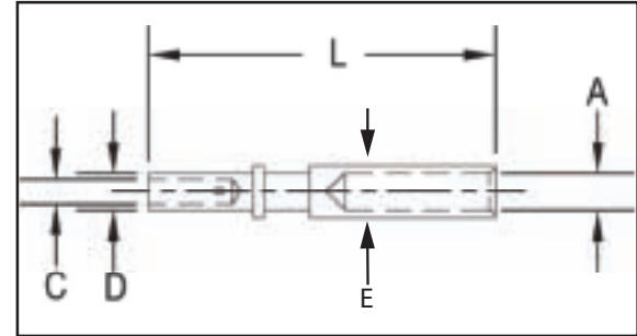
Female (Socket)
