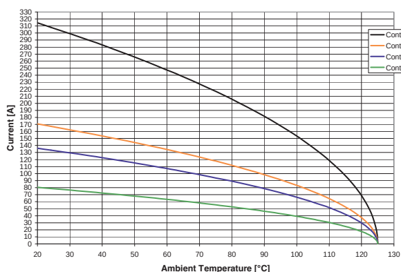
Derating Curves ITT-Cannon
