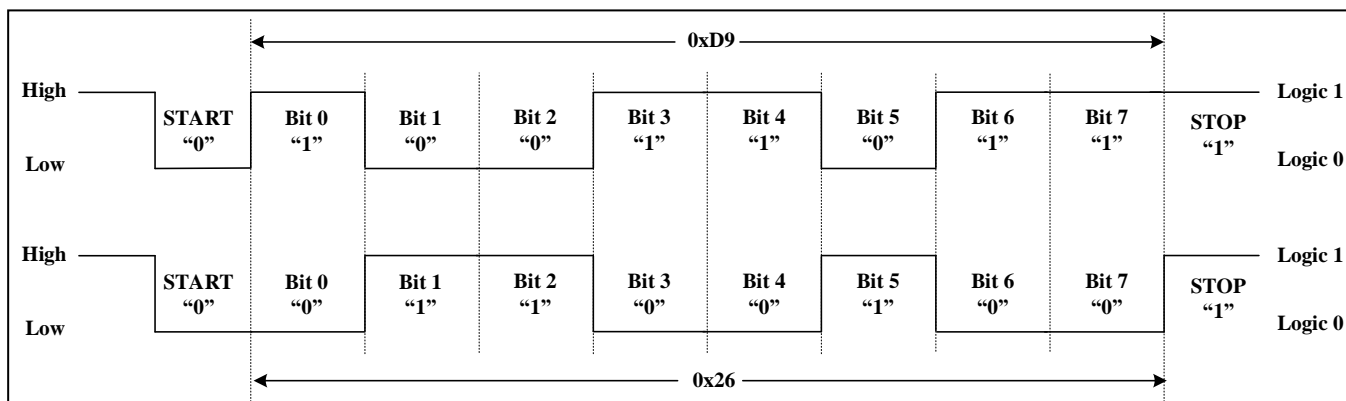
Figure 15 UART Data Transaction Example
