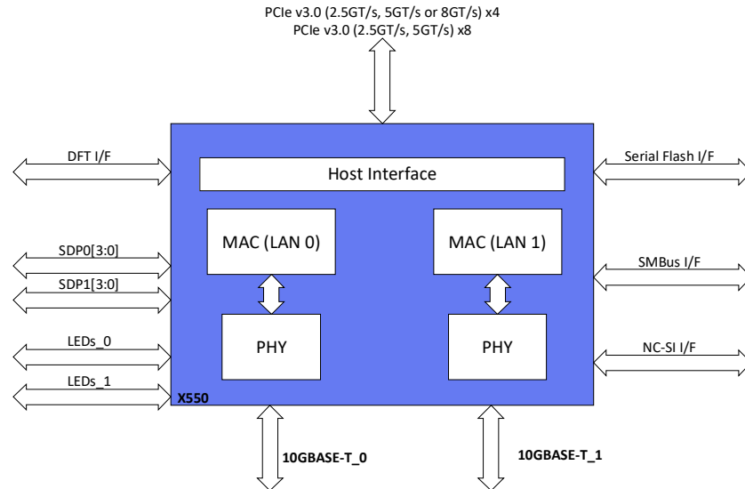
Figure 1-2. X550 External Interfaces Diagram
