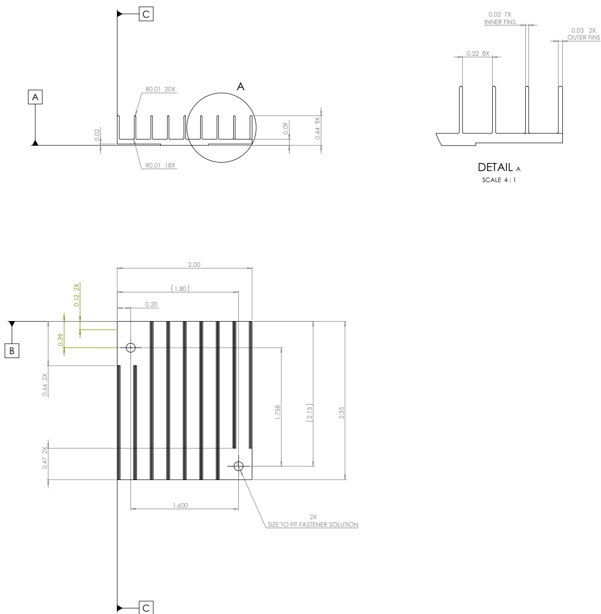
Figure 14-3. X550 Extruded Heat Sink
