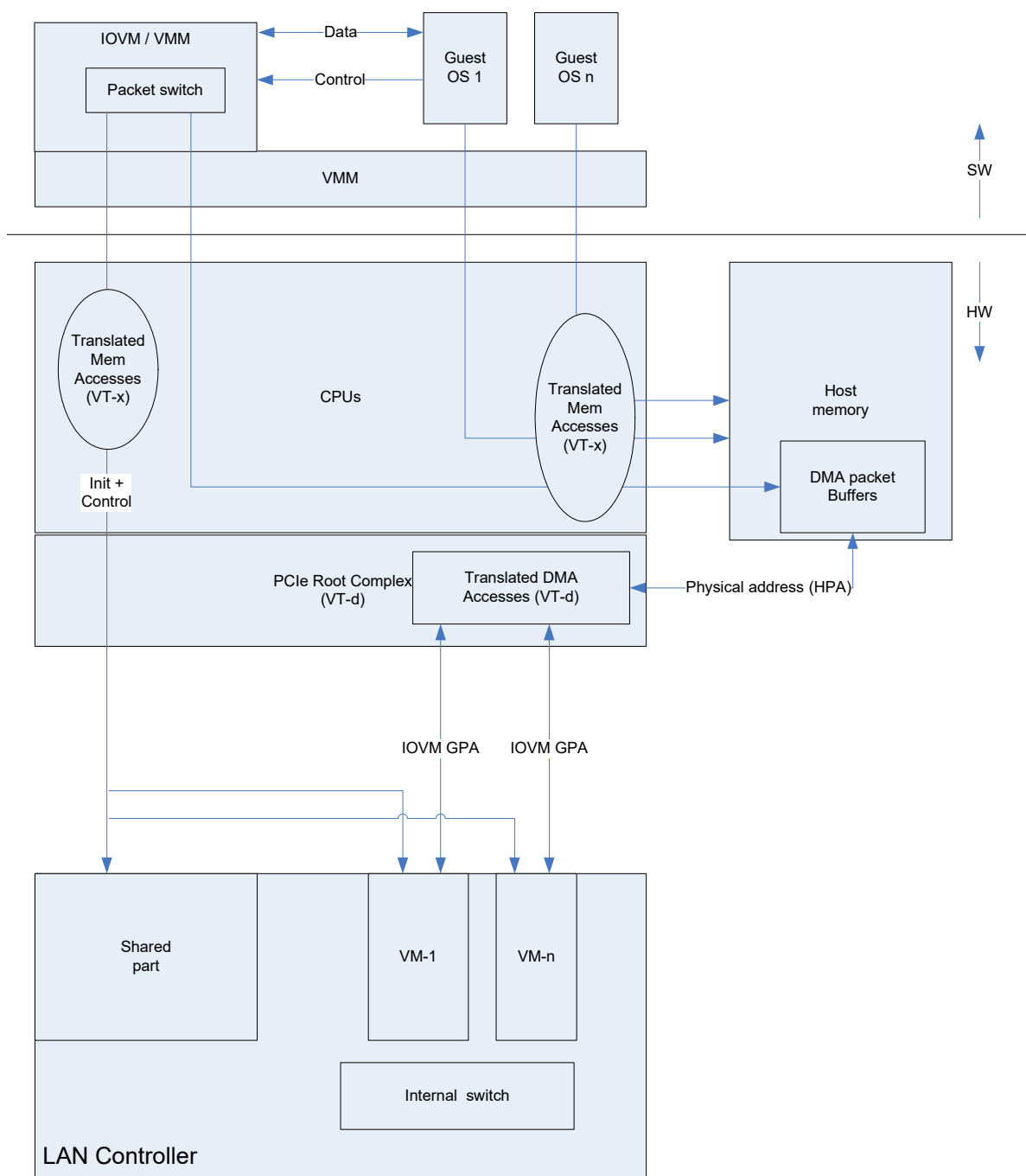
Figure 9-3. VMDq System
