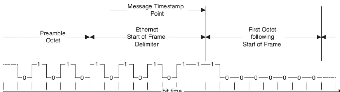
Figure 9-19. Timestamp Point
