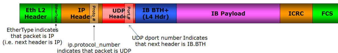
Figure A-41. RoCEv2 Packet Format
