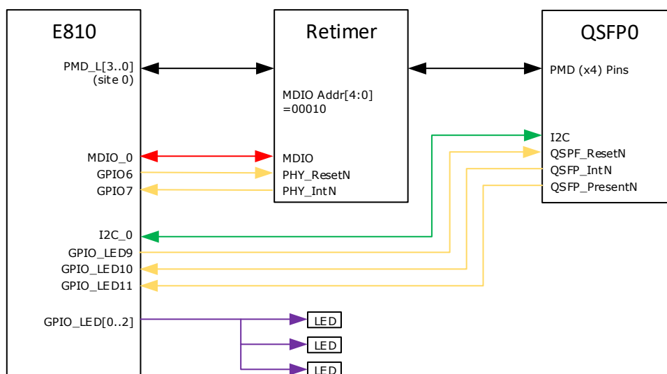
Figure 3-20. NIC Topology Use Case
