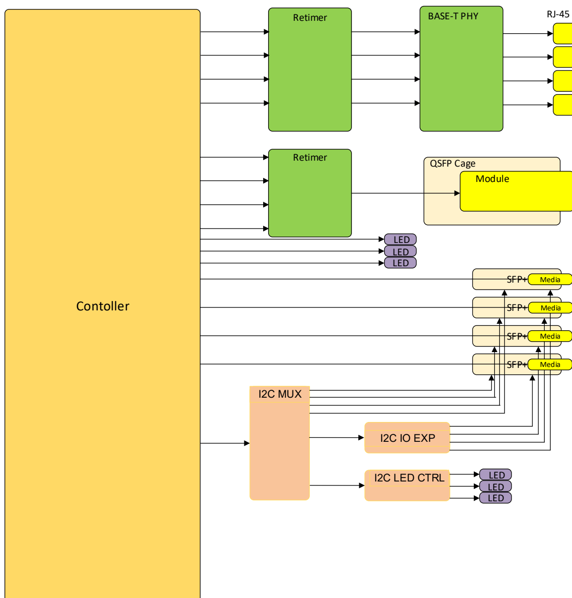
Figure 3-18. Topology Schematic
