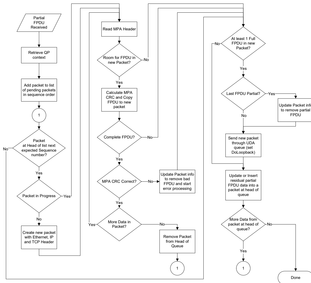
Figure 11-21. Partial FPDU Software Algorithm
