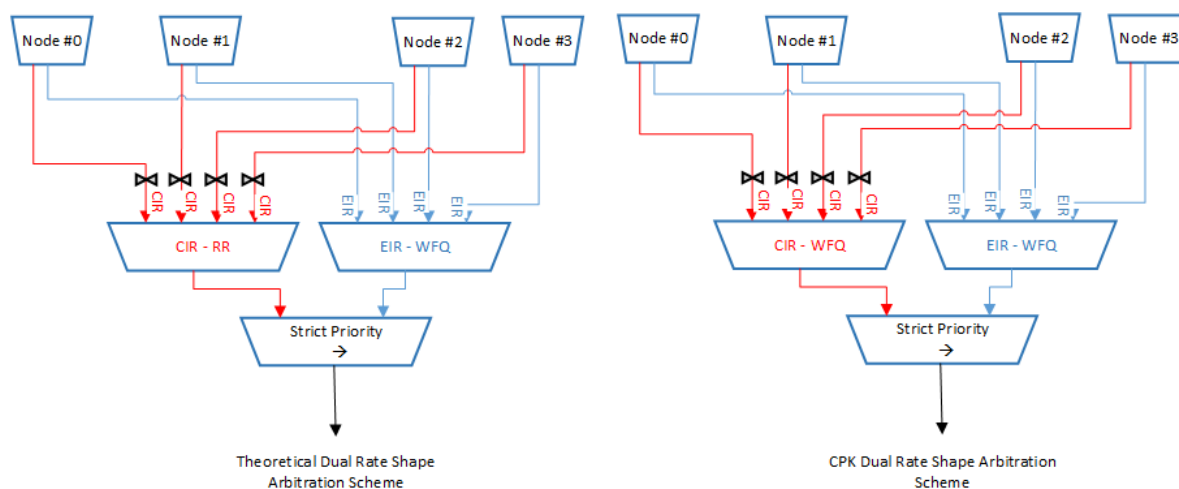
Figure 8-5. Dual Rate Shaper Arbitration Scheme
