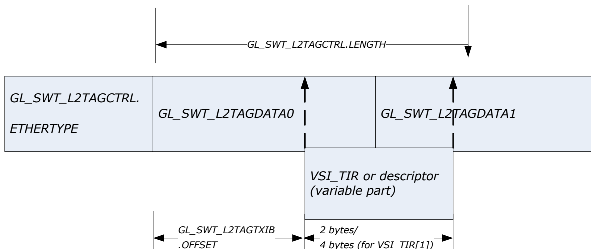
Figure 7-38. Tag Insertion
