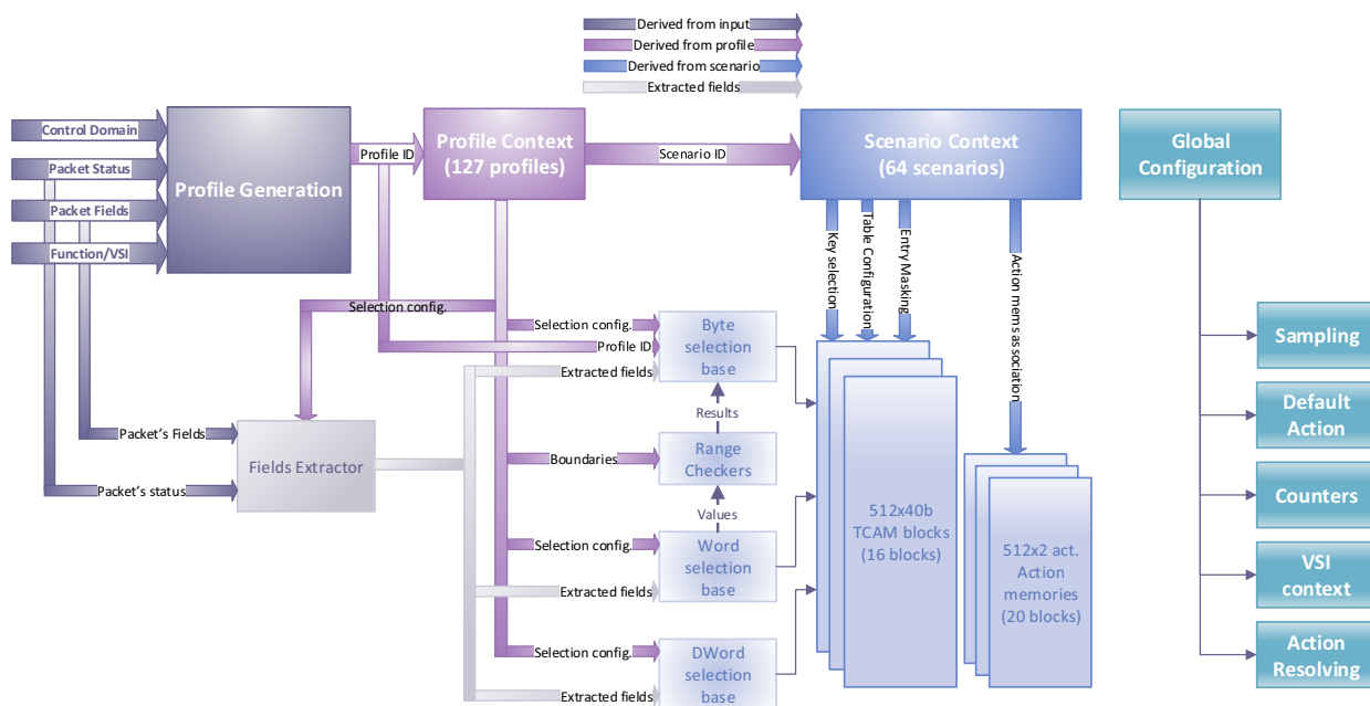
Figure 7-27. Configuration Sources 1
