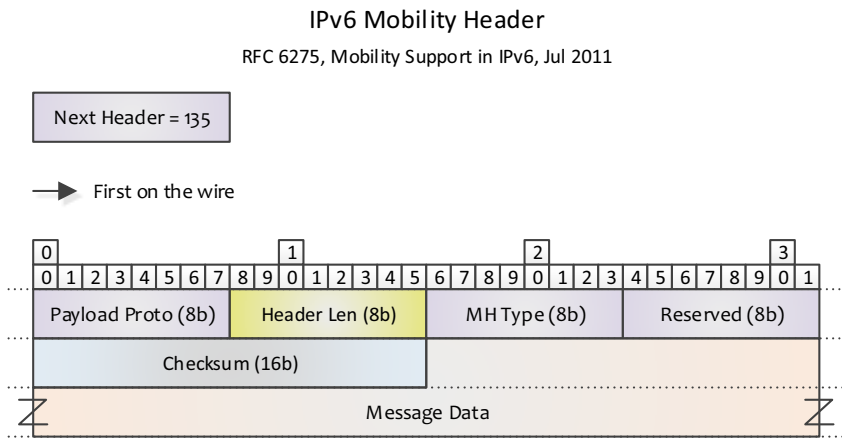
Figure A-21. IPv6 Mobility Header
