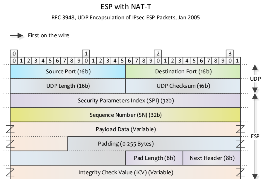
Figure A-44. ESP NAT-T Header Structure
