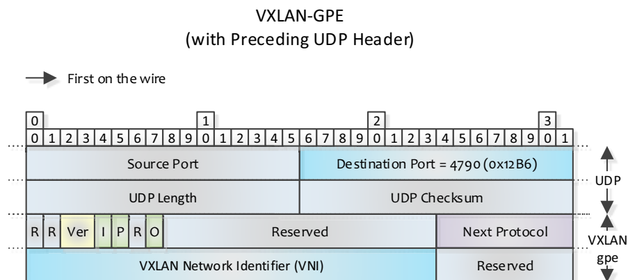
Figure A-38. VXLAN-GPE over UDP
