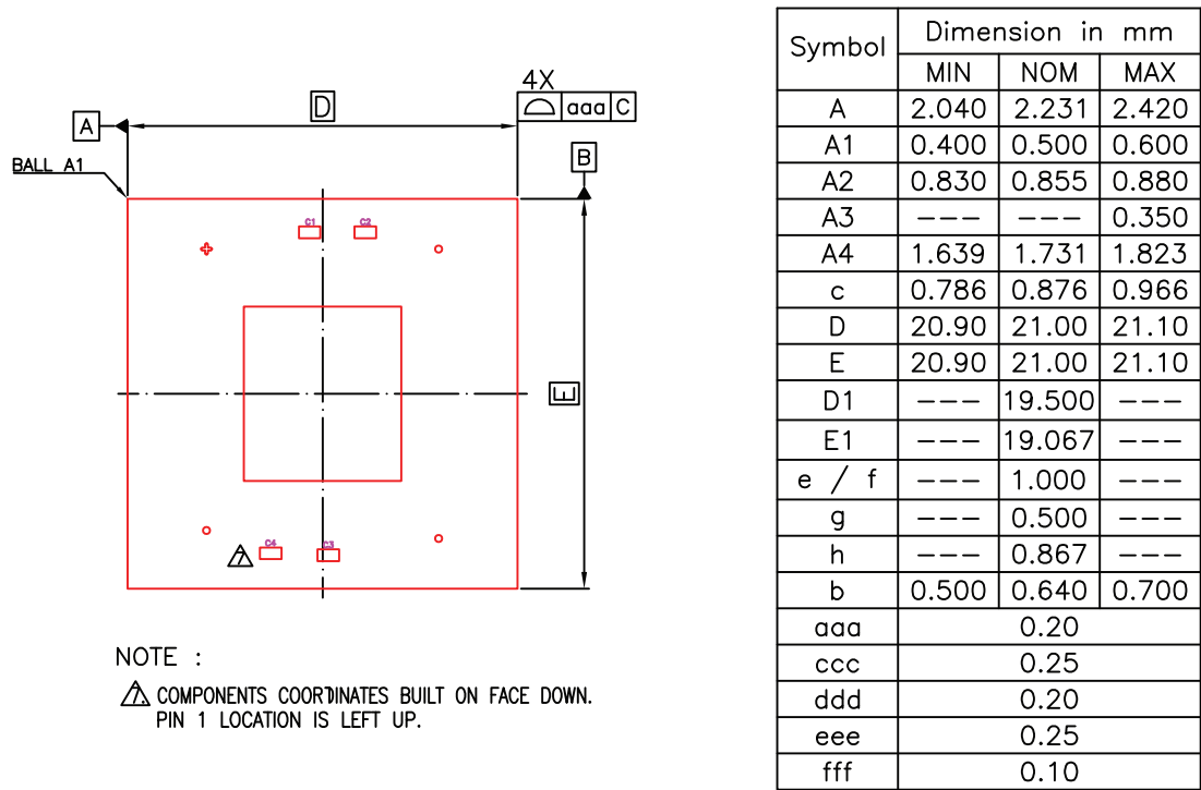
Figure 16-13. E810-XXVAM2 Mechanical Package Diagram (Top View)
