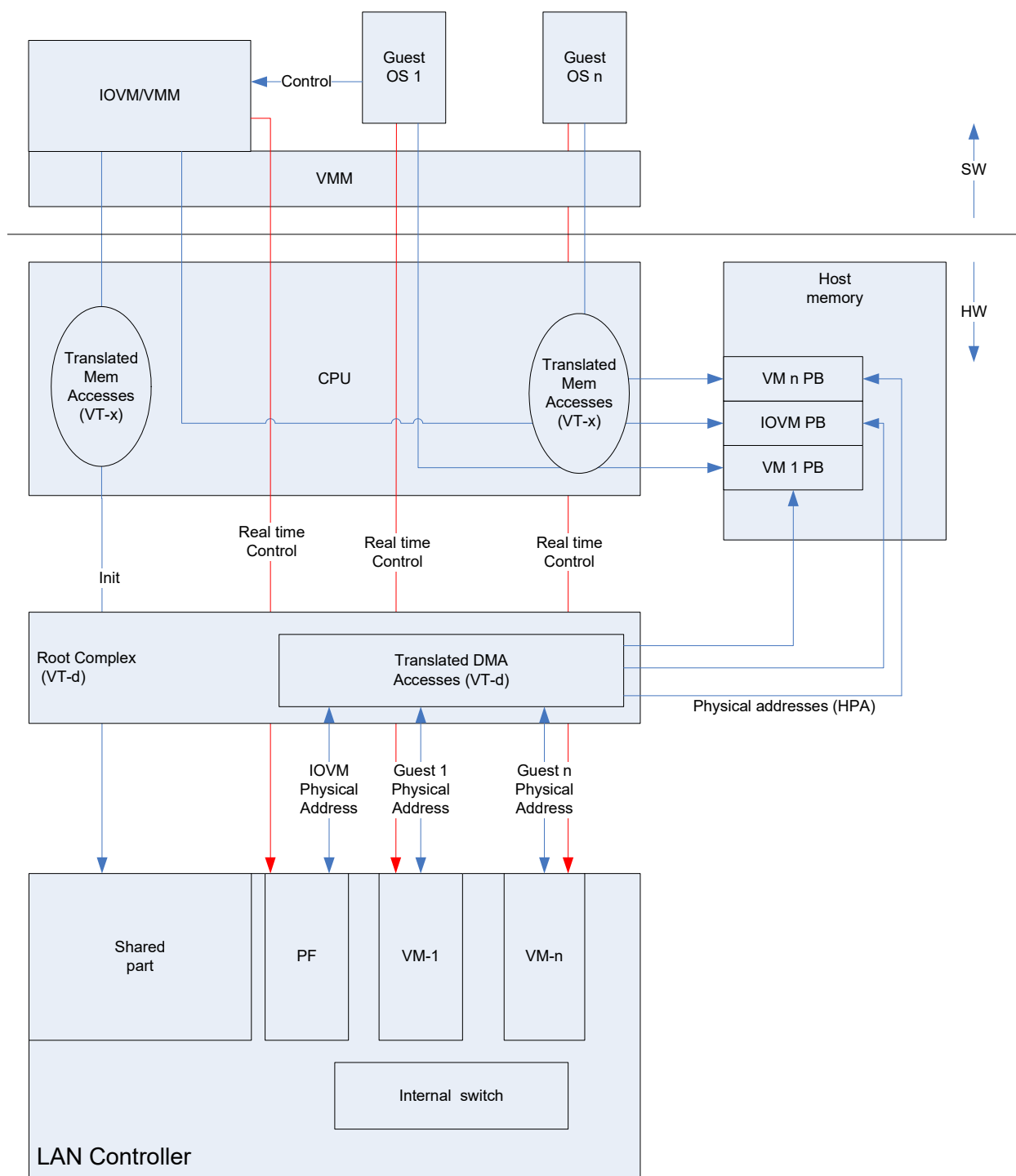
Figure 9-4. SR-IOV Based System
