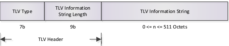
Figure A-11. Structure of an LLDP TLV
