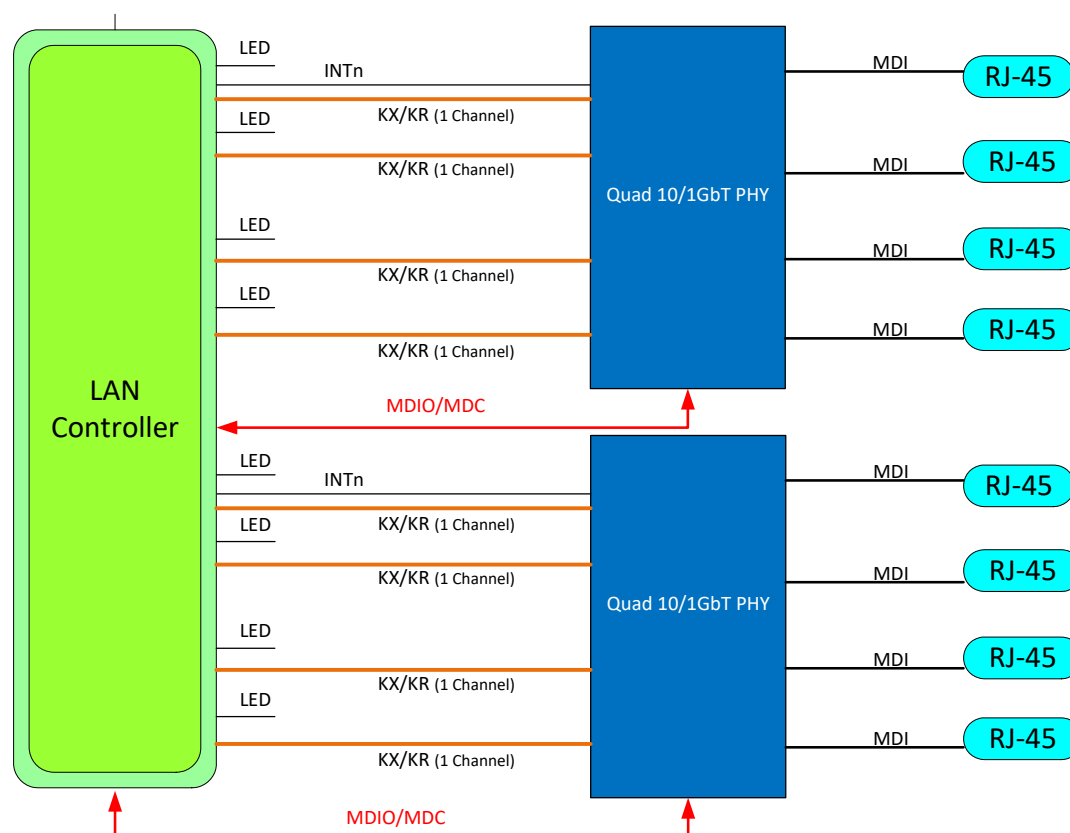
Figure 3-14. Octal 10GBASE-T/1GBASE-T
