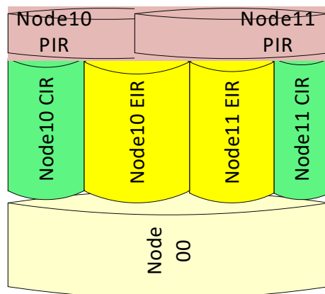
Figure 8-6. Parent Bandwidth Distribution Between Two Child Nodes
