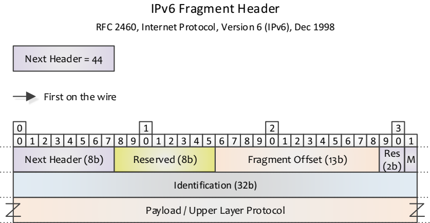
Figure A-18. IPv6 Fragment Header
