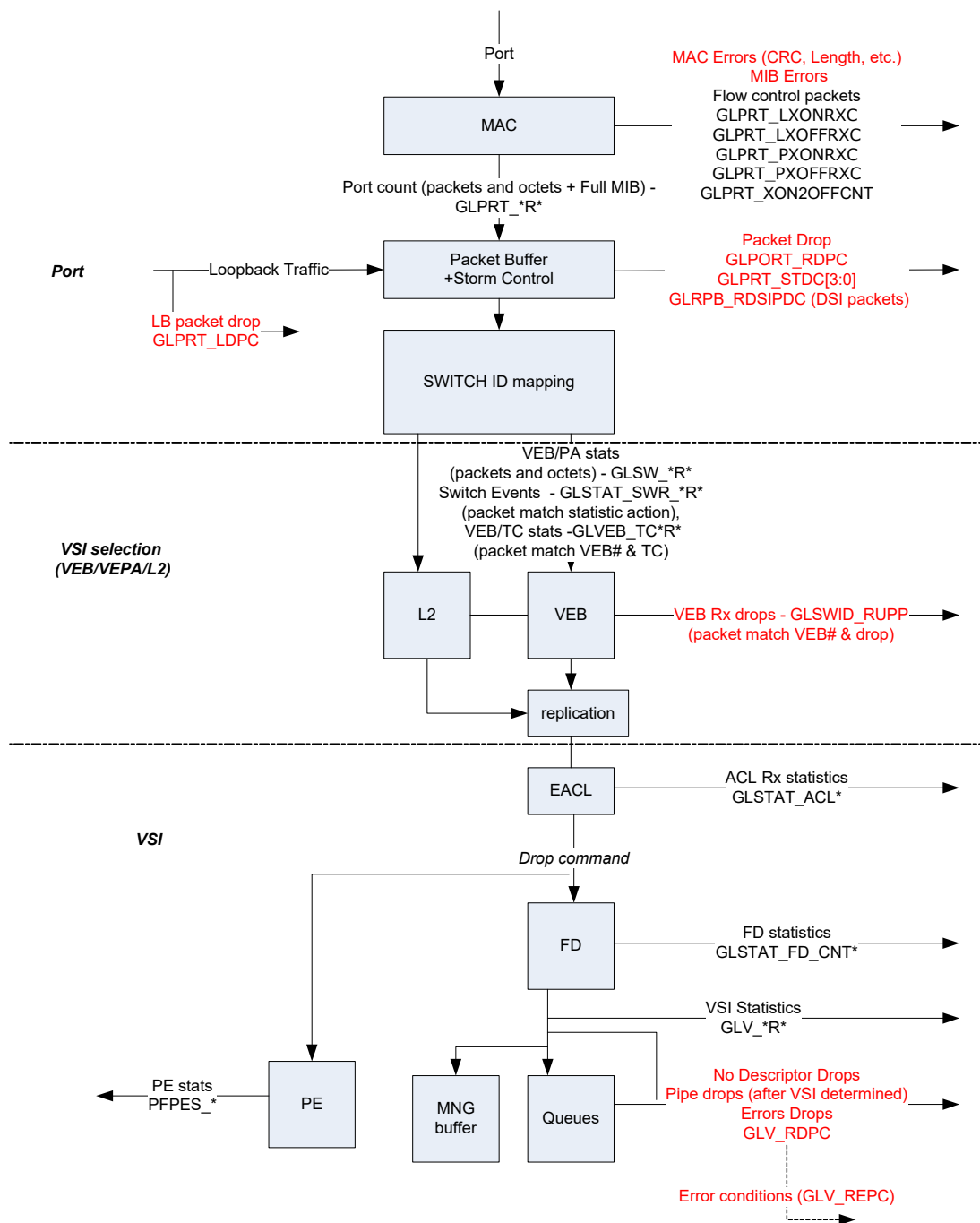
Figure 9-11. Rx Statistics Sampling Points
