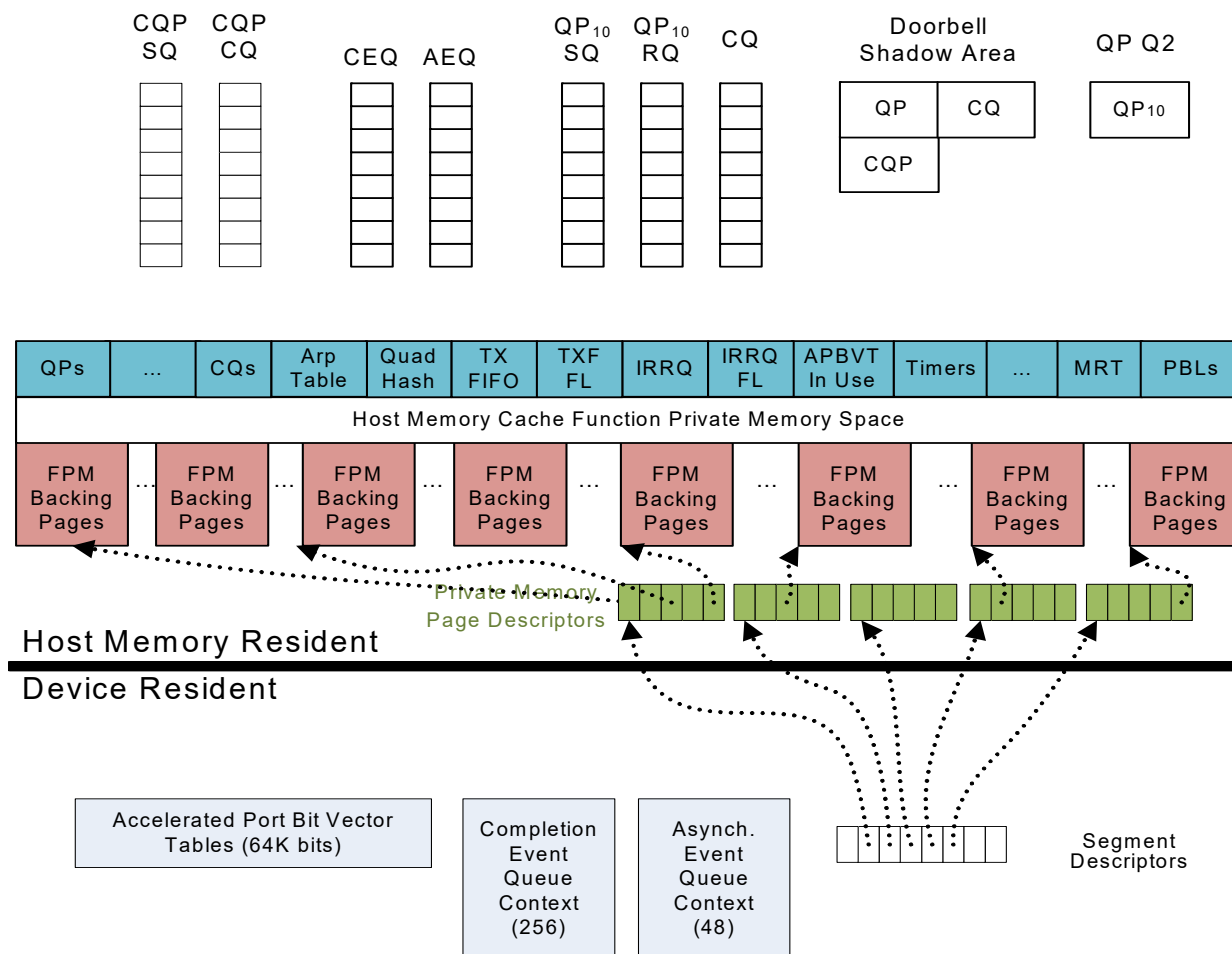
Figure 11-22. E810 and Host Memory Data Structures
