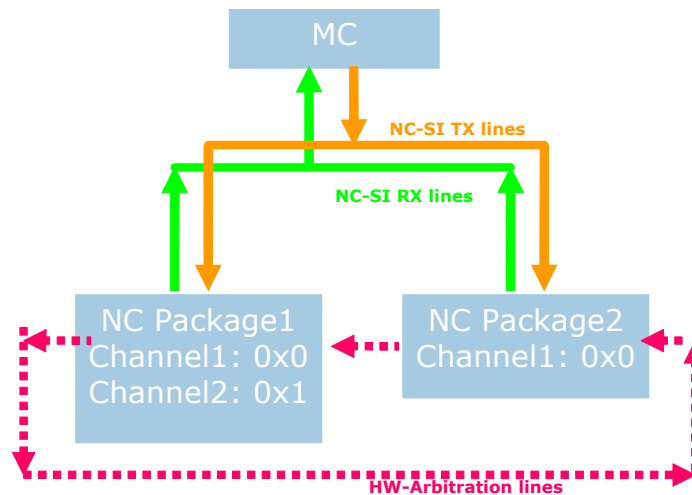
Figure 12-9. Multi-NC Environment
