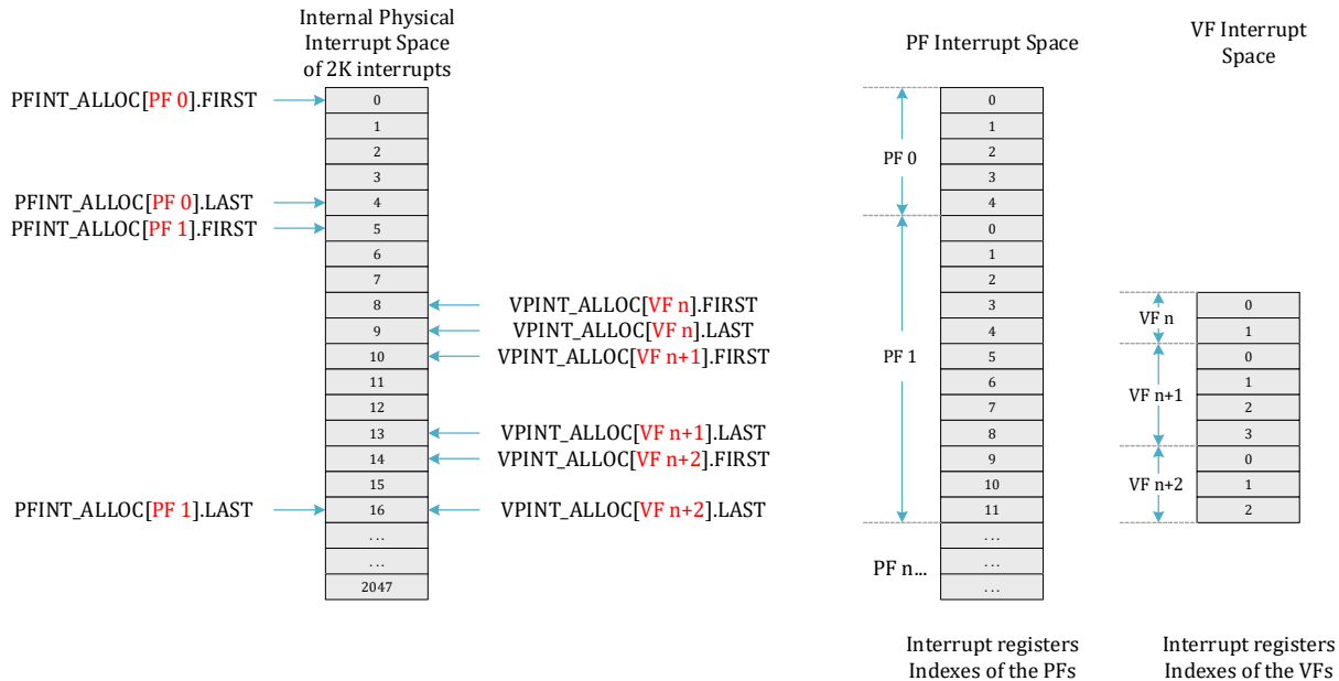
Figure 9-1. Example for Interrupt Vectors and CEQ Interrupt Control Registers Mapping to the Internals Space
