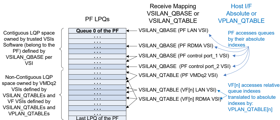
Figure 10-2. PF Queues (Example)
