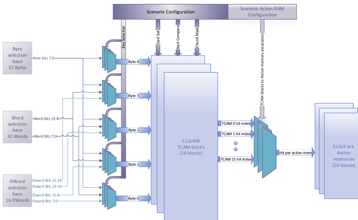
Figure 7-28. Scenario-Dependent Configuration
