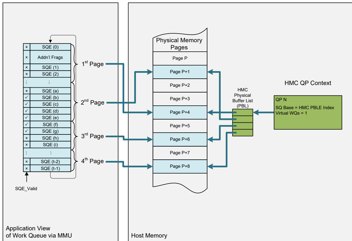
Figure 11-15. PE Operation: Virtual SQ
