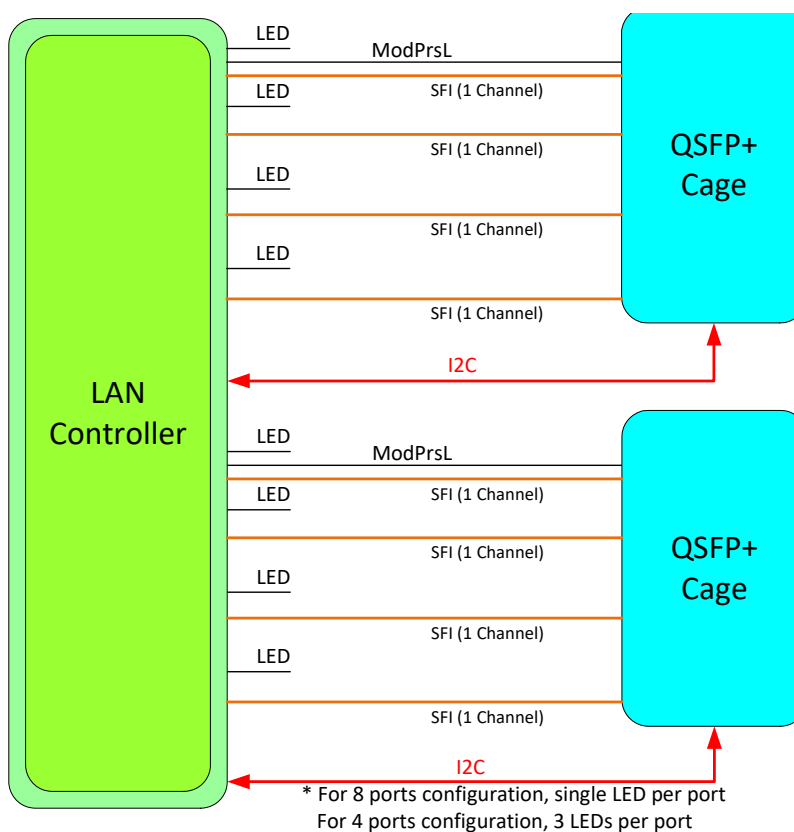
Figure 3-12. Octal 10GDual QSFP+
