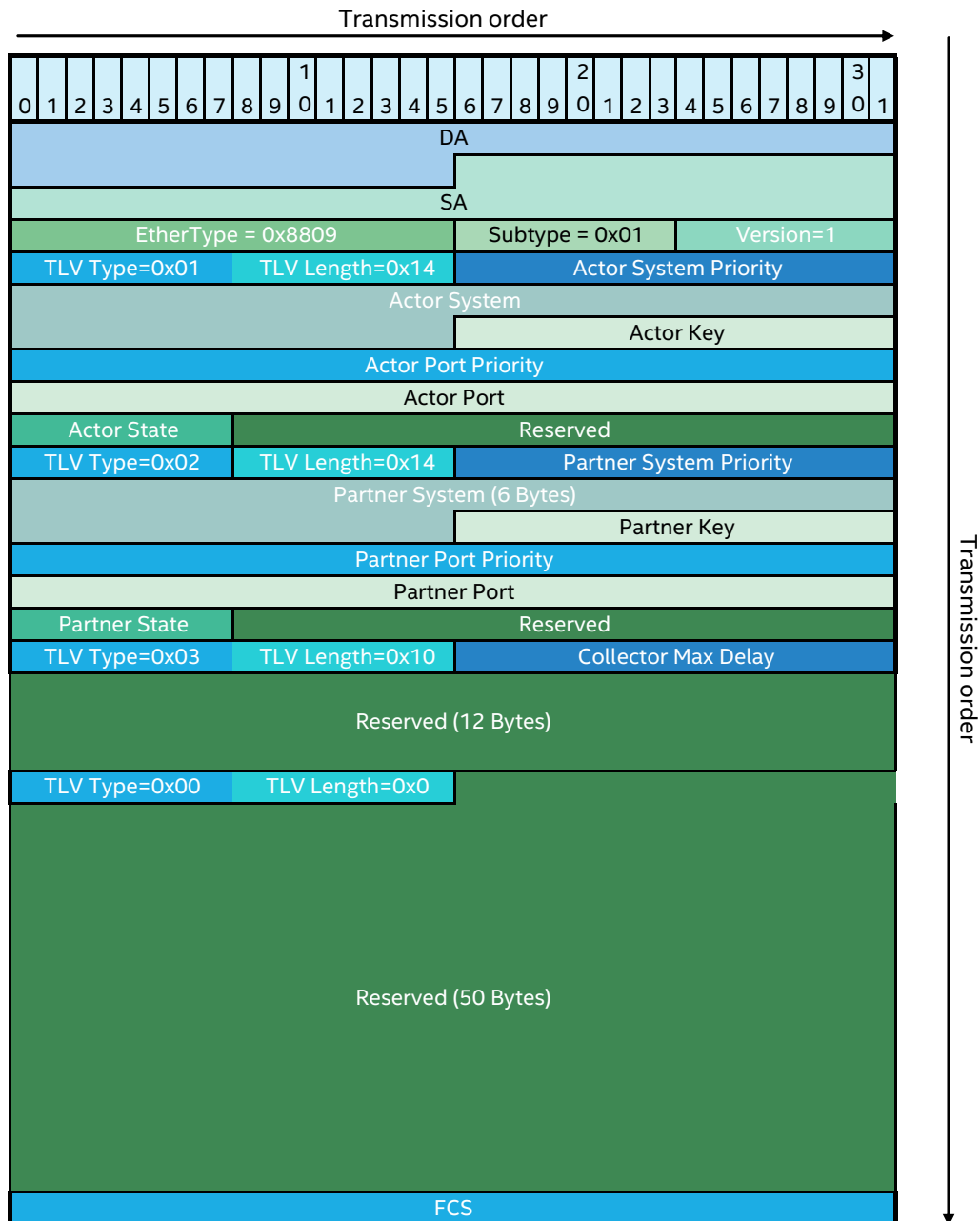
Figure A-5. LACP Version 1 Frame Format
