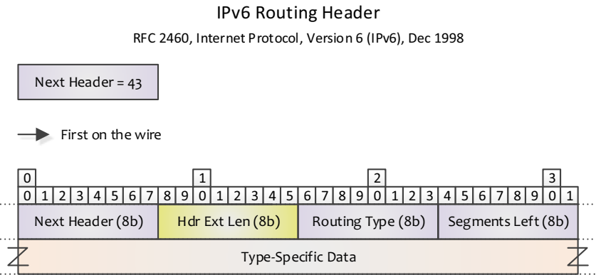
Figure A-17. IPv6 Routing Header
