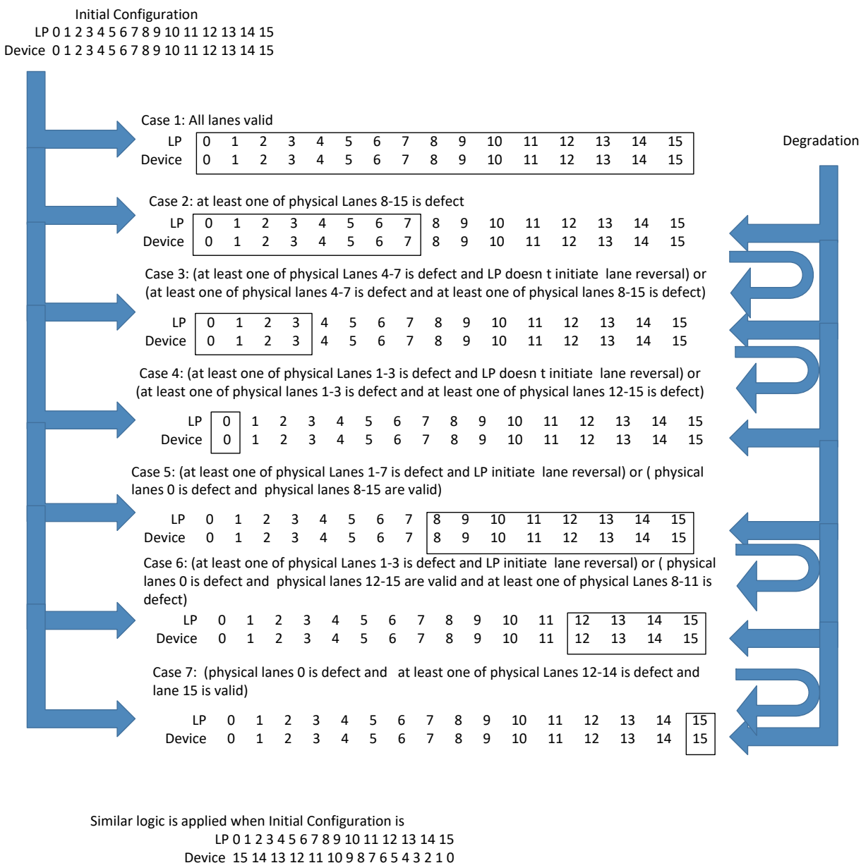
Figure 3-4. Link Width Configurations for a x16 Port
