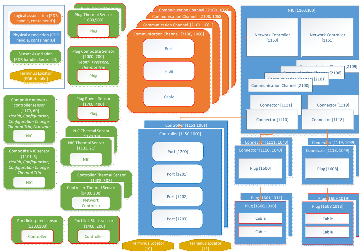
Figure 12-13. PDR/Sensor Diagram
