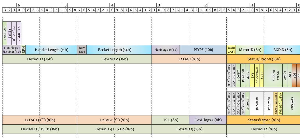
Figure 7-8. Receive Flex Descriptor (with Flags)
