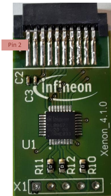
Figure 5 Xenon – SPI TPM board - pin configuration
