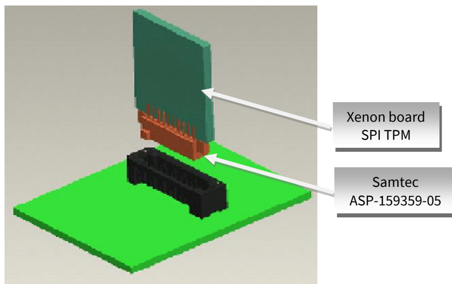
Figure 6 Board connection Xenon –SPI TPM board with motherboard
