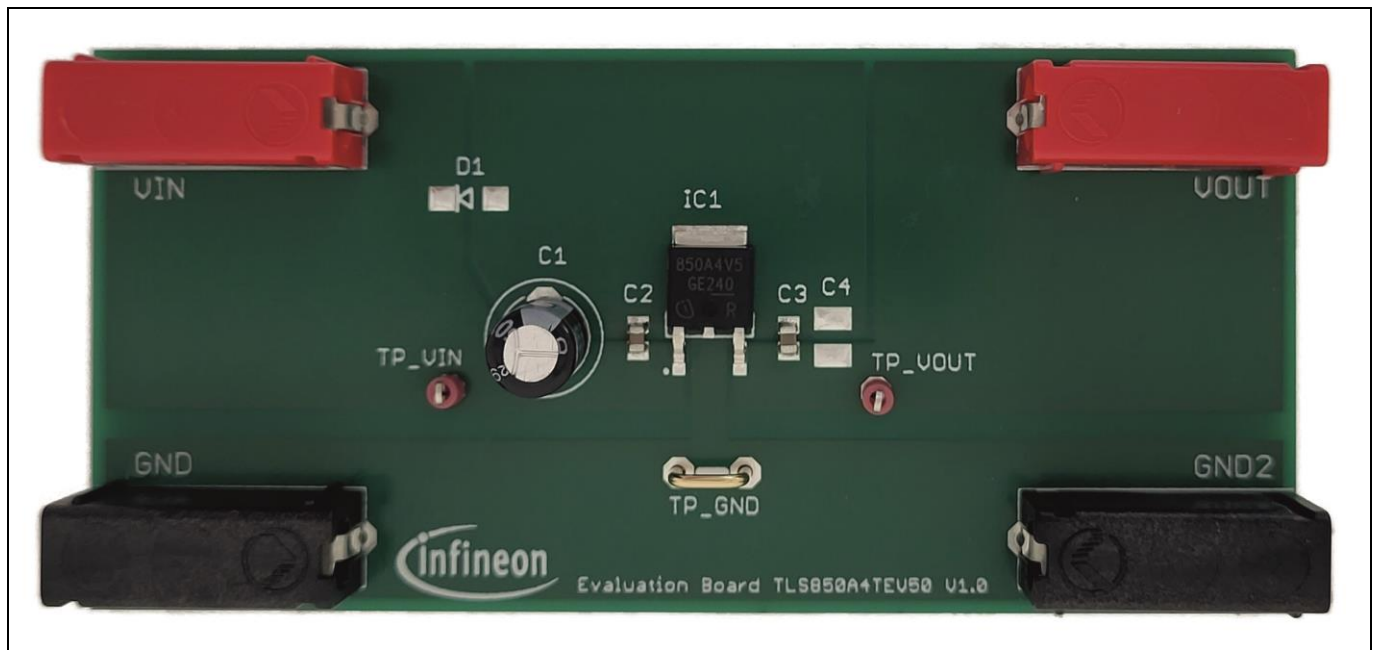
Figure 2 TLS850A4TEV50 demoboard
