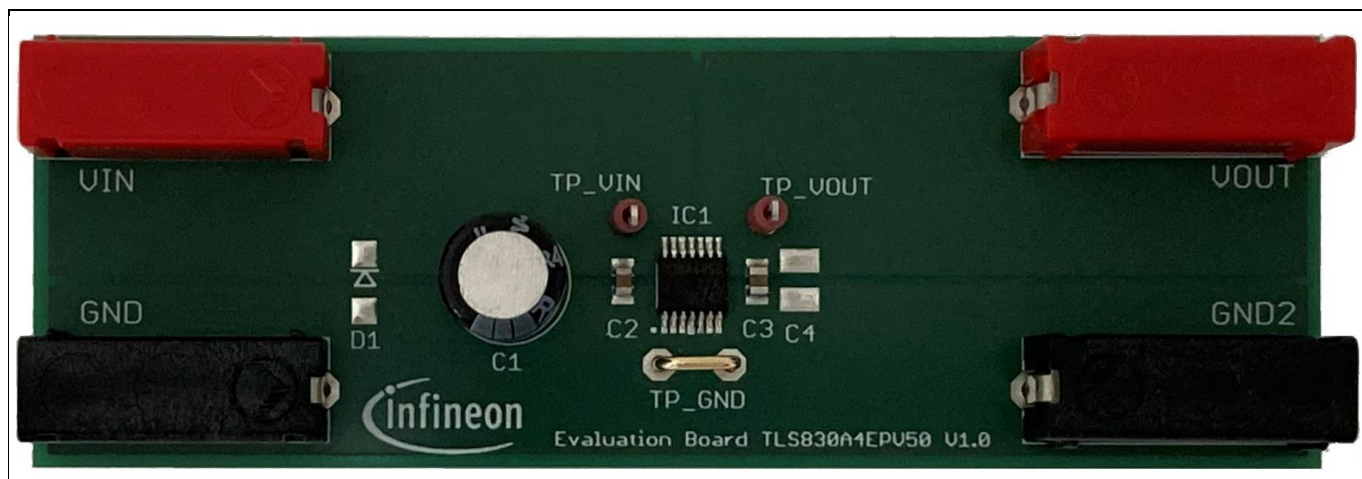
Figure 2 TLS830A4EPV50 demoboard
