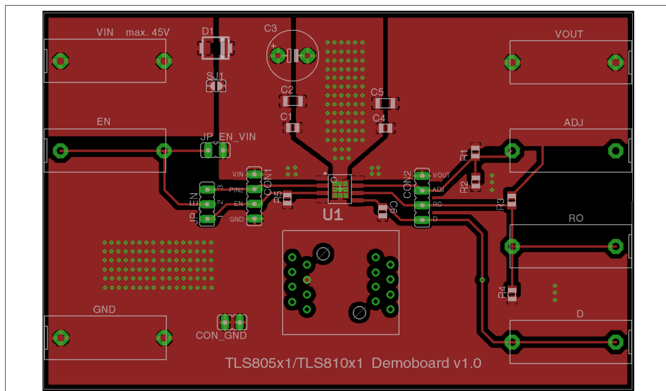
Figure 4 Top layer of TLS805x1xJ/TLS810x1xJ Demoboard
