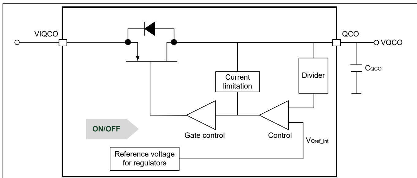
Figure 8 Block diagram LDO-QCO
