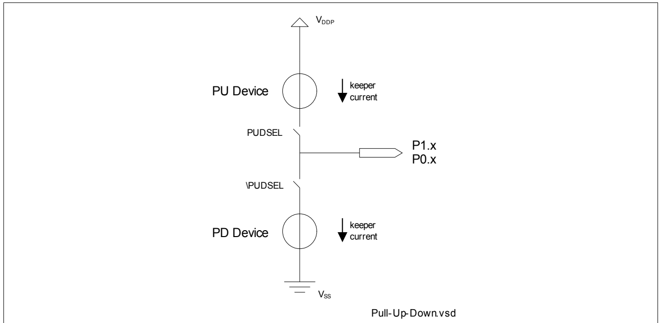
Figure 34 Pull-Up/Down Device
