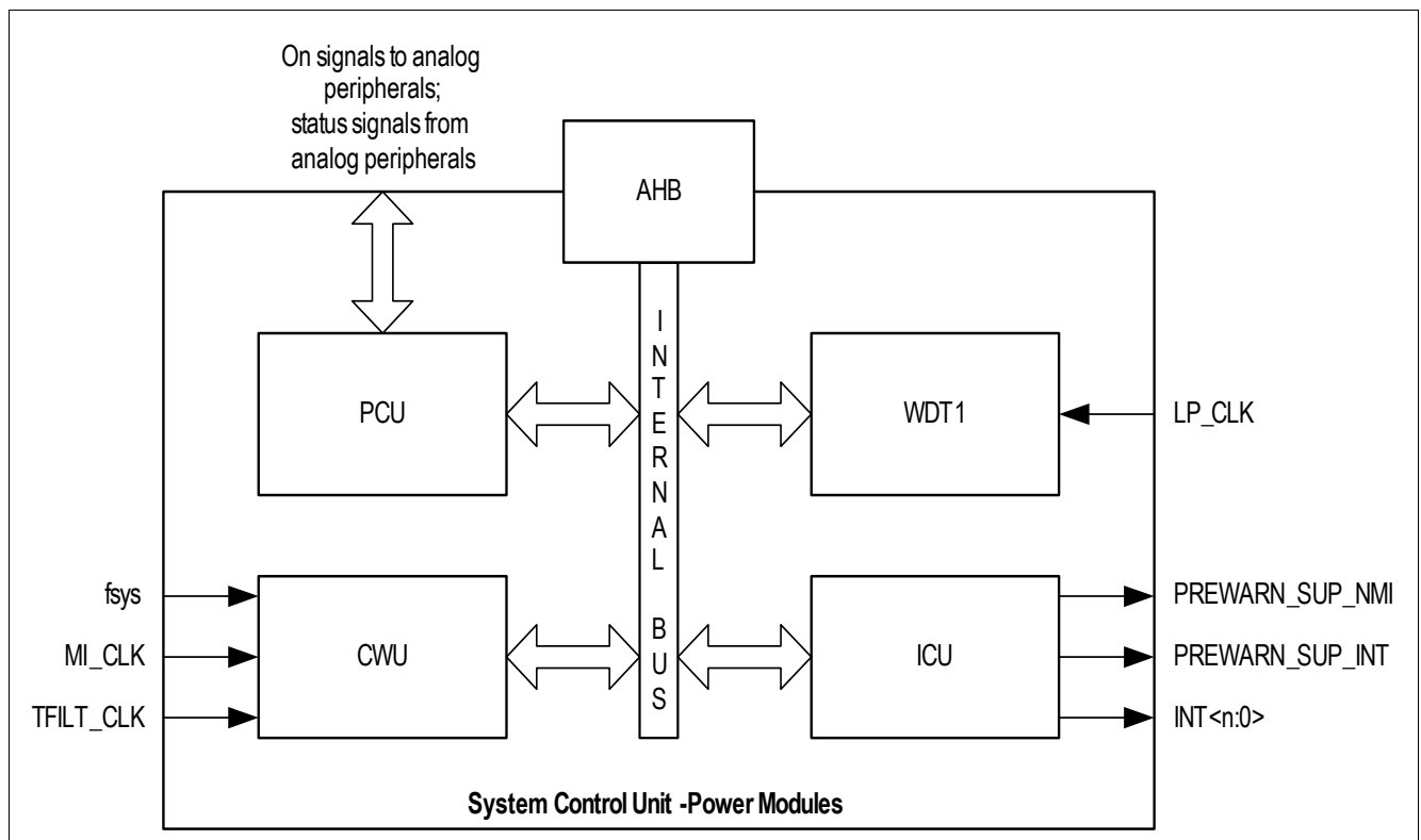
Figure 11 Block diagram of System Control Unit - Power Modules
