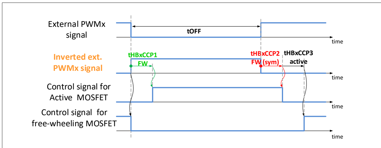
Figure 28 Internal signals for PWM operation - General case: t_{OFF} > t_{HBxCCP1} , t_{ON} > t_{HBxCCP2} active, motor operating as generator
