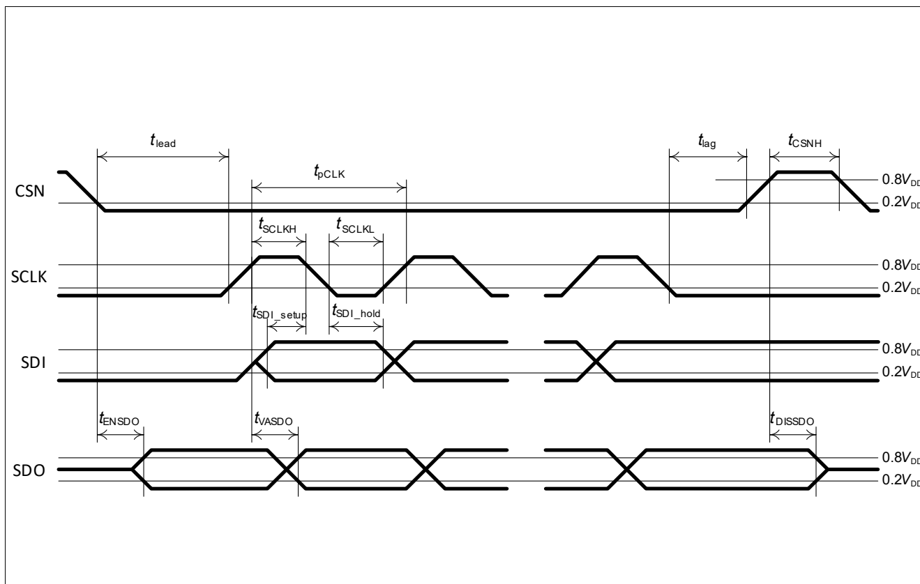
Figure 48 SPI timing parameters
