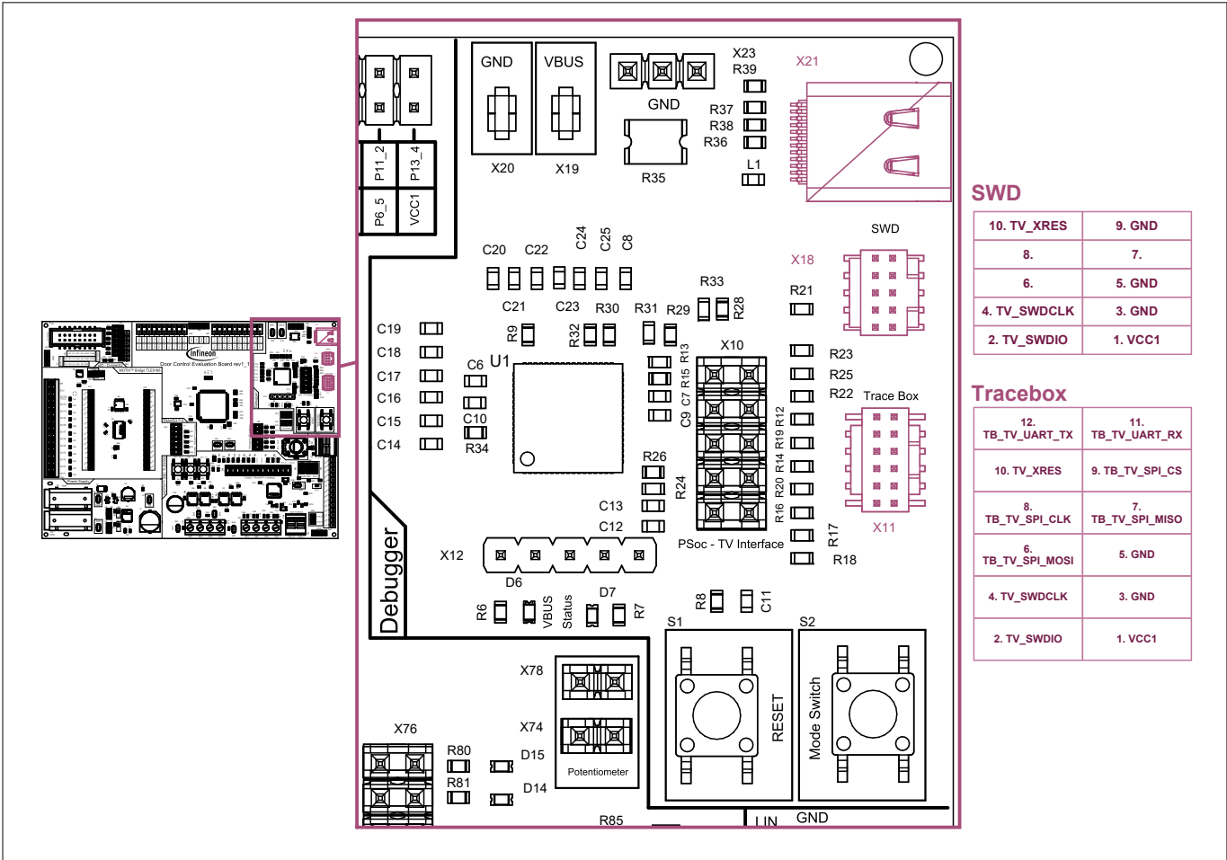
Figure 40 Connectors and available signals
