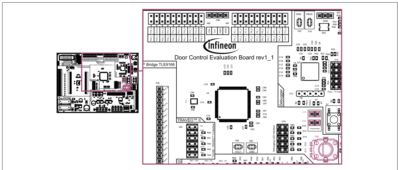
Figure 31 Placement and pinout of the potentiometer
