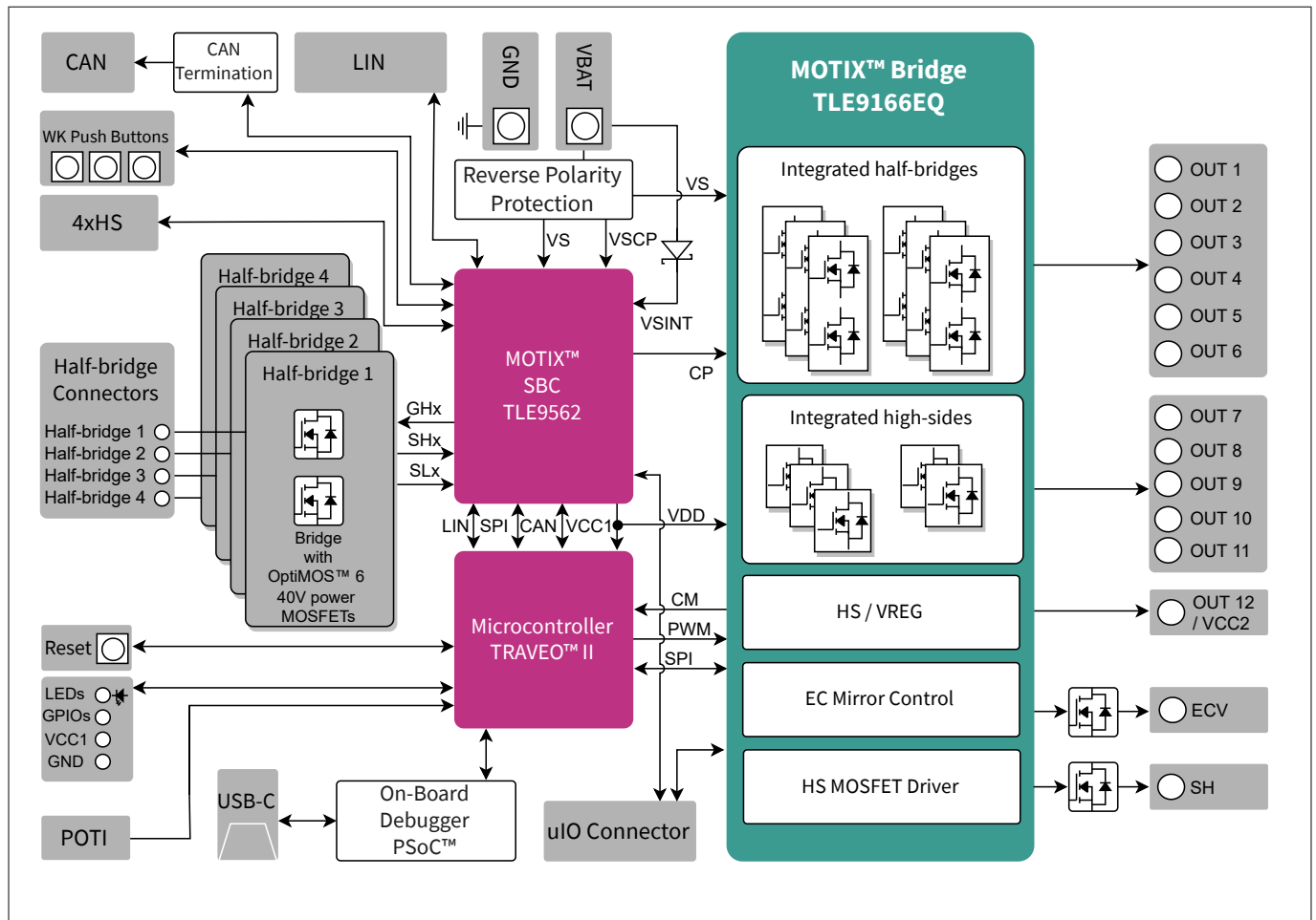
Figure 3 Block diagram
