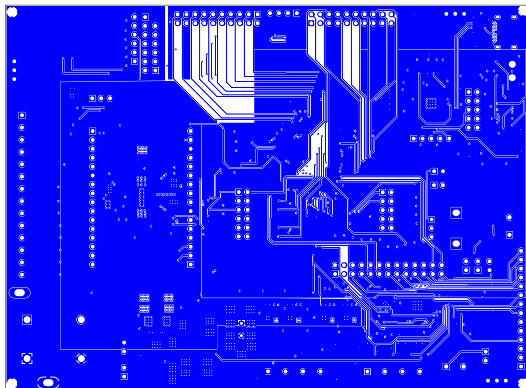
Figure 57 Door control evaluation board layer 4 (bottom layer, power)
