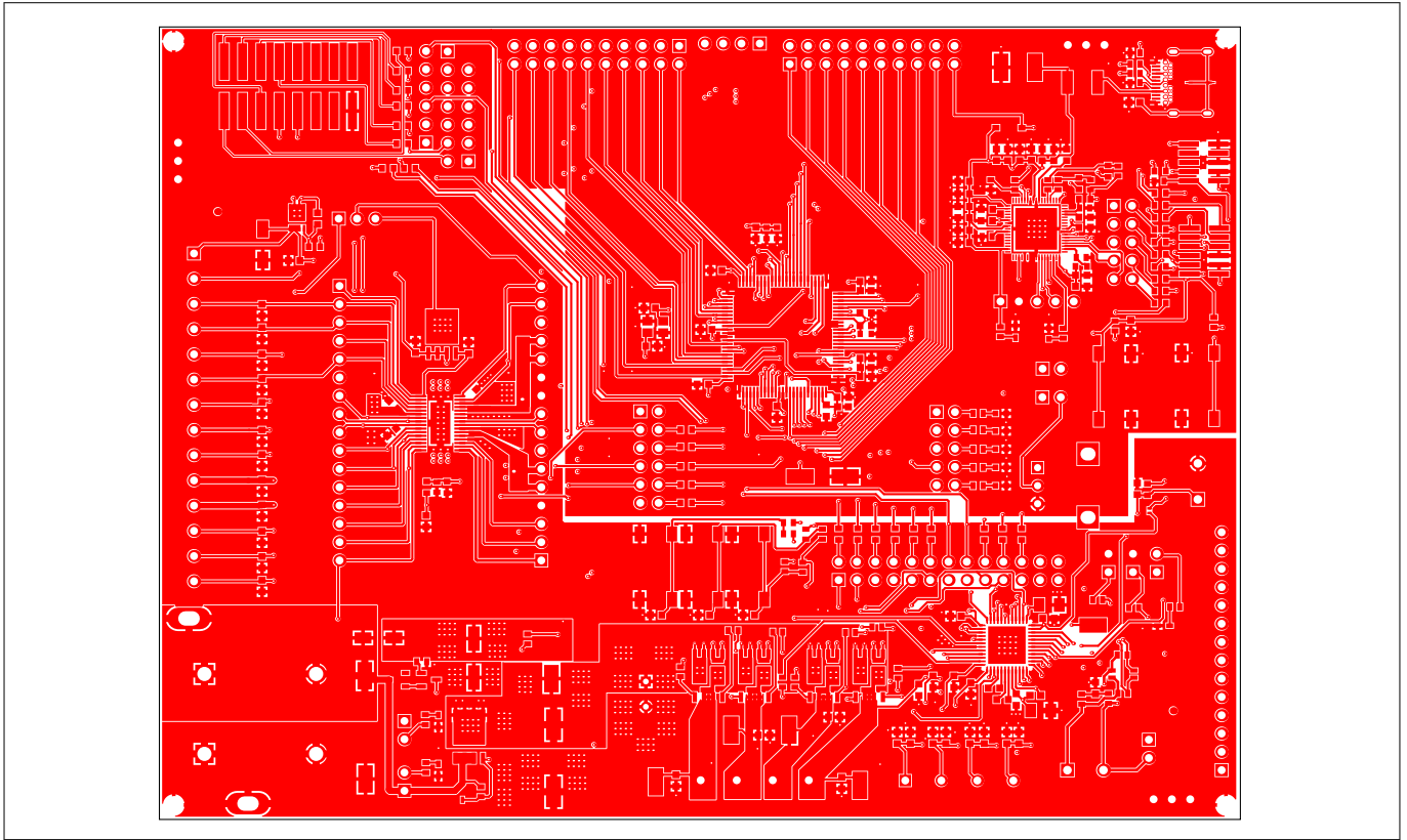
Figure 54 Door control evaluation board layer 1 (top layer, signal)
