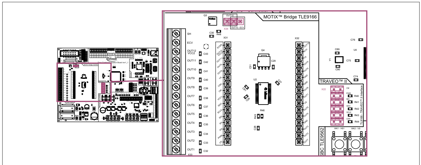
Figure 15 Jumpers
