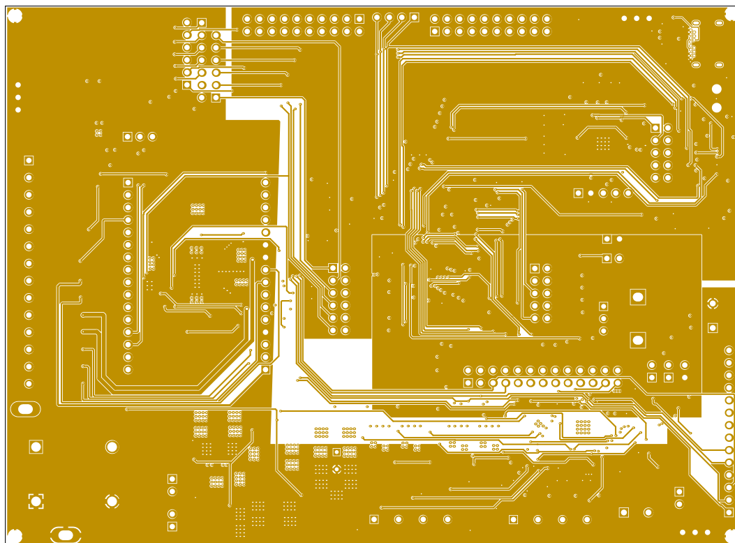
Figure 56 Door control evaluation board layer 3 (middle layer, signal)
