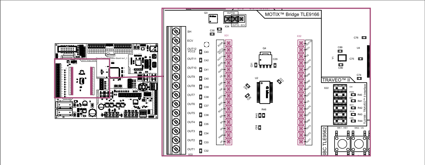
Figure 16 Signal pin headers
