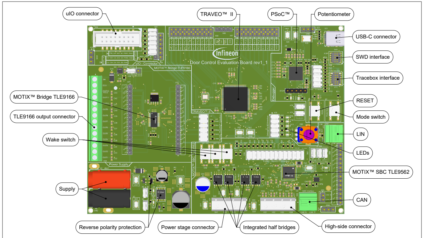
Figure 4 Board description
