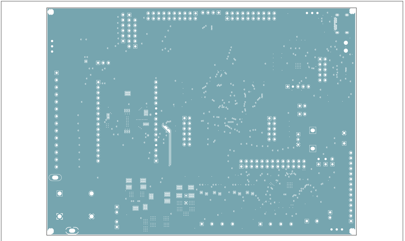
Figure 55 Door control evaluation board layer 2 (middle layer, GND )
