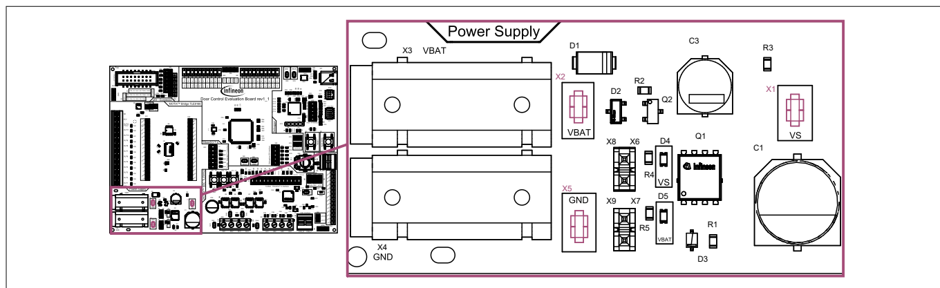
Figure 35 Test points
