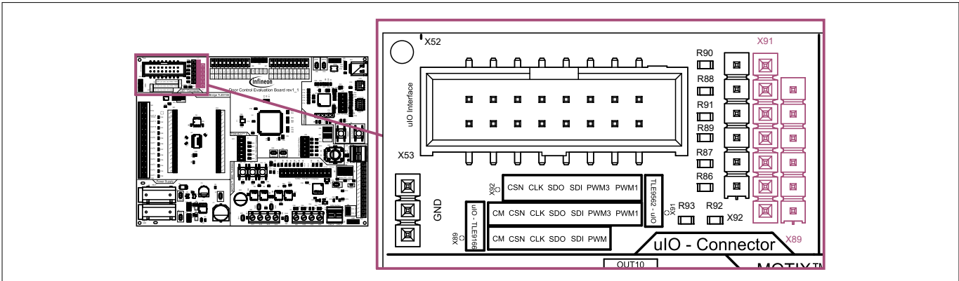
Figure 38 Using the uIO-Stick connector to configure MOTIX™ devices over the configuration wizard
