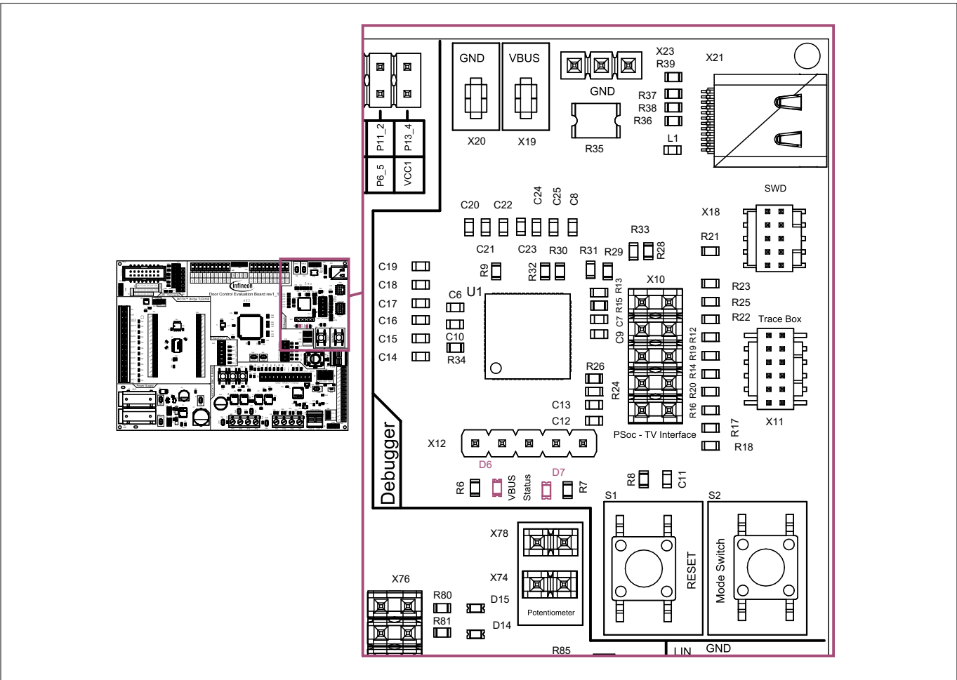
Figure 45 LEDs
