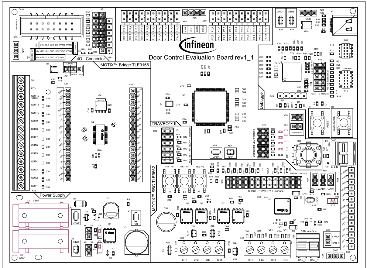
Figure 13 Supply connector and LEDs
