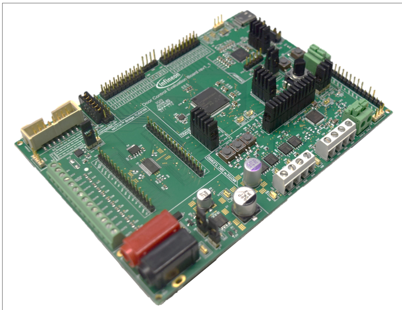
Figure 1 Door control evaluation board
