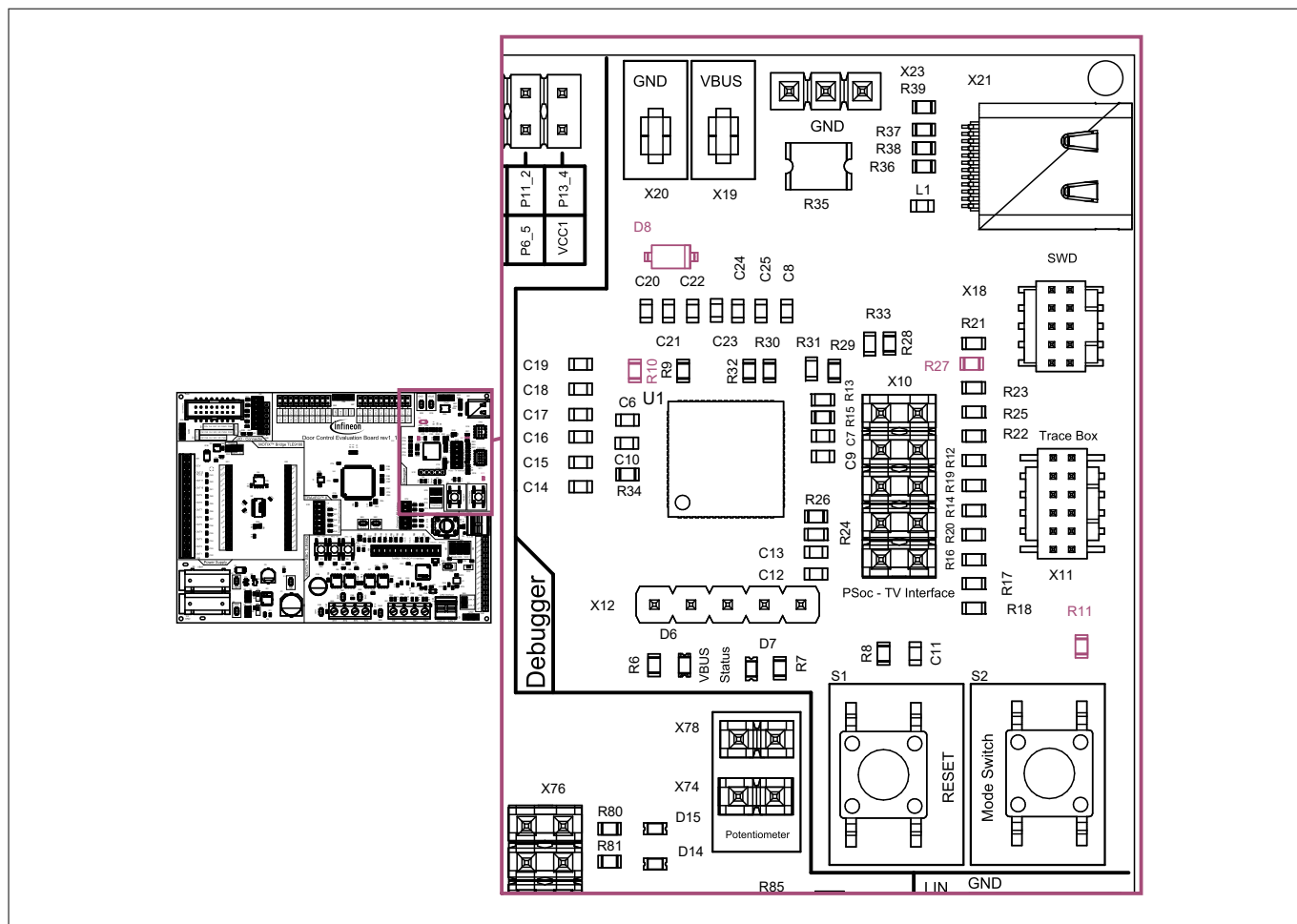
Figure 46 Assembly options
