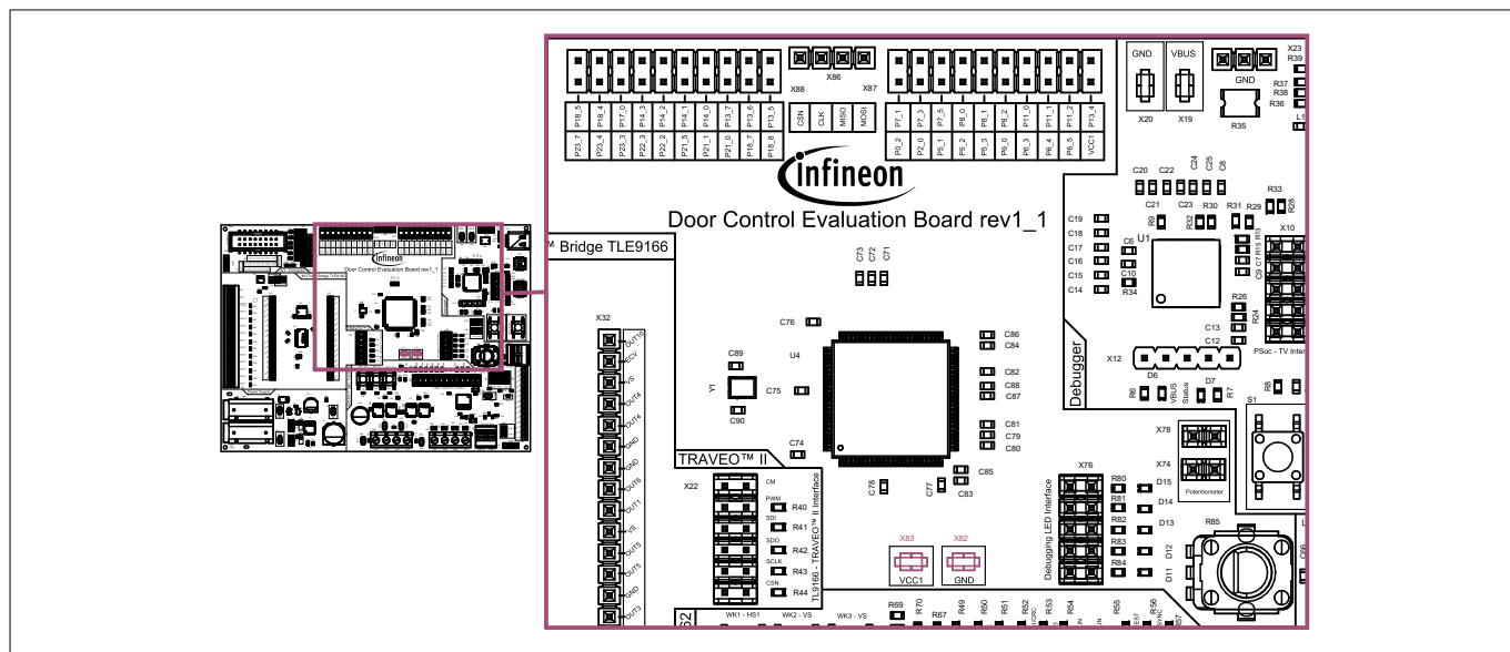
Figure 28 Test points
