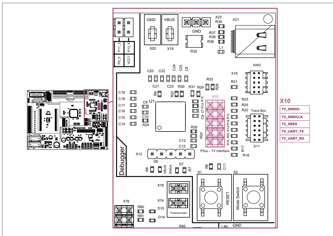
Figure 41 Jumpers
