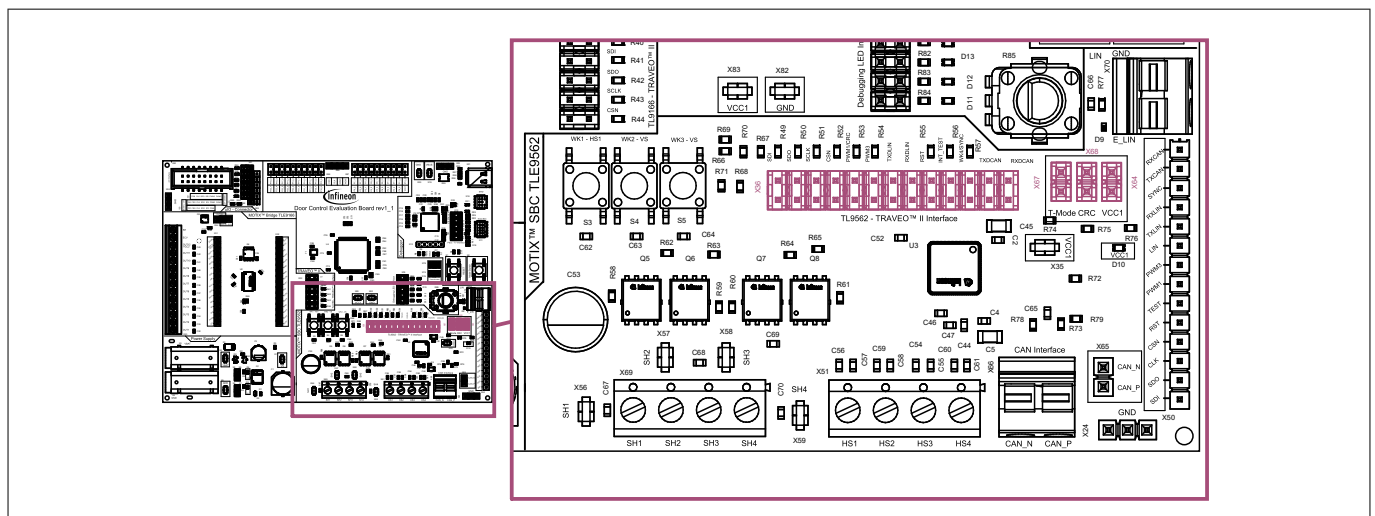
Figure 19 Jumpers
