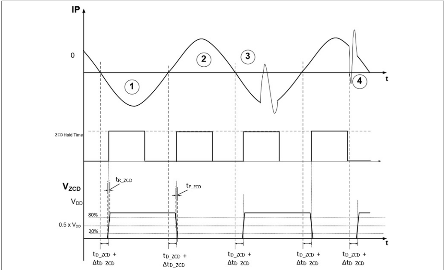
Figure 17 ZCD output timing diagram
