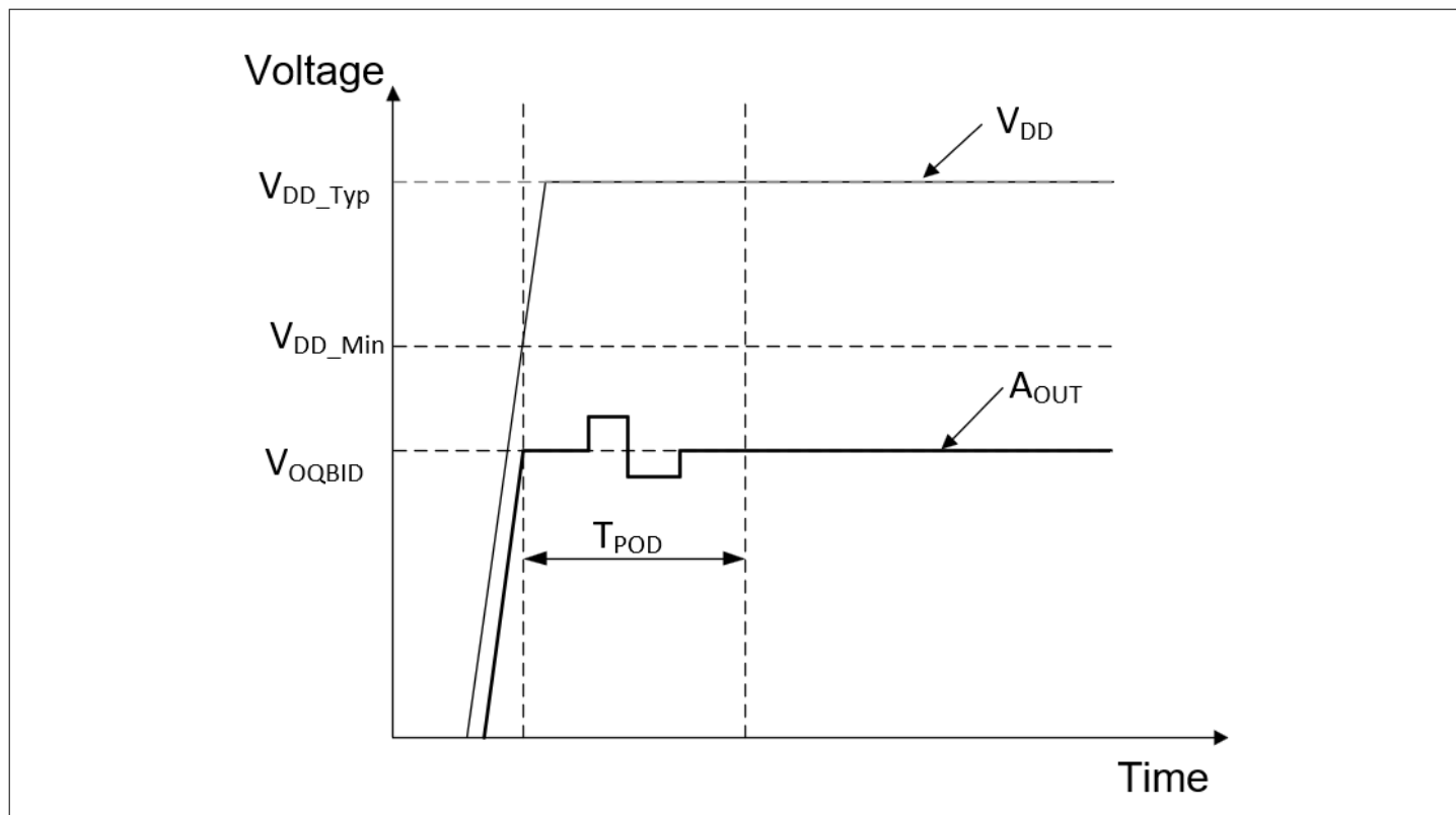
Figure 14 Power ON delay behavior
