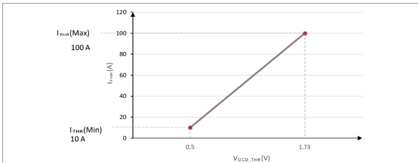
Figure 16 Threshold voltage ( V_{OCD\_THR} ) vs threshold current ( I_{THR} )
