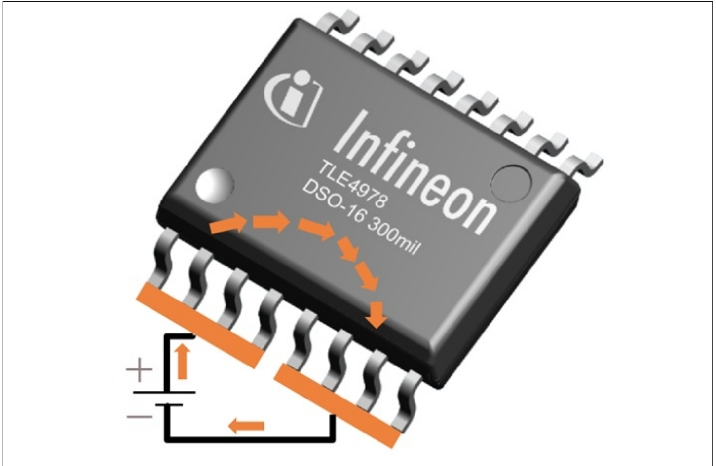
Figure 4 Polarity illustration DSO-16 300mil package
