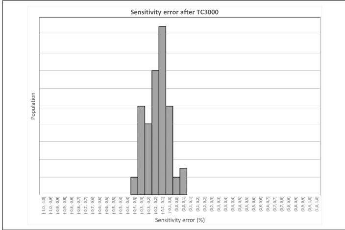
Figure 12 Population vs sensitivity error
