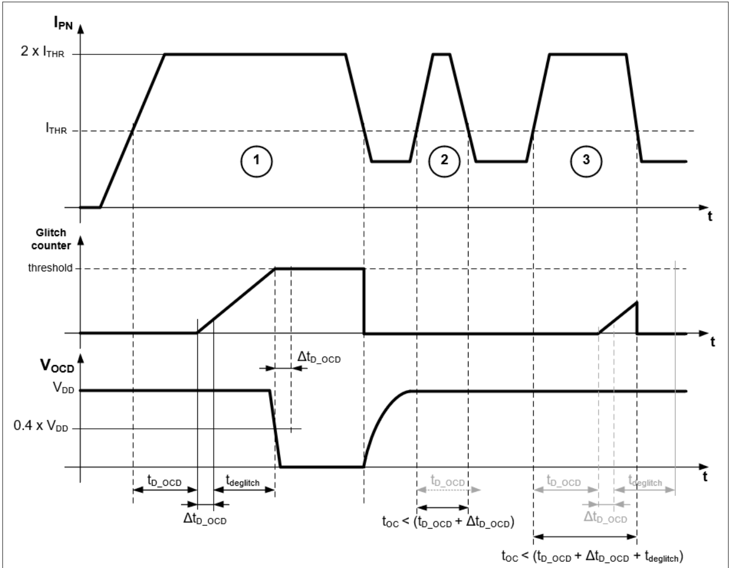
Figure 15 OCD output timing behavior
