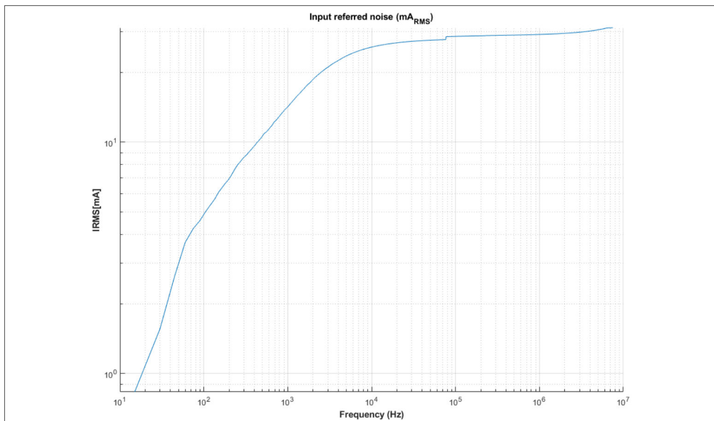
Figure 11 Input referred accumulated noise vs Frequency
