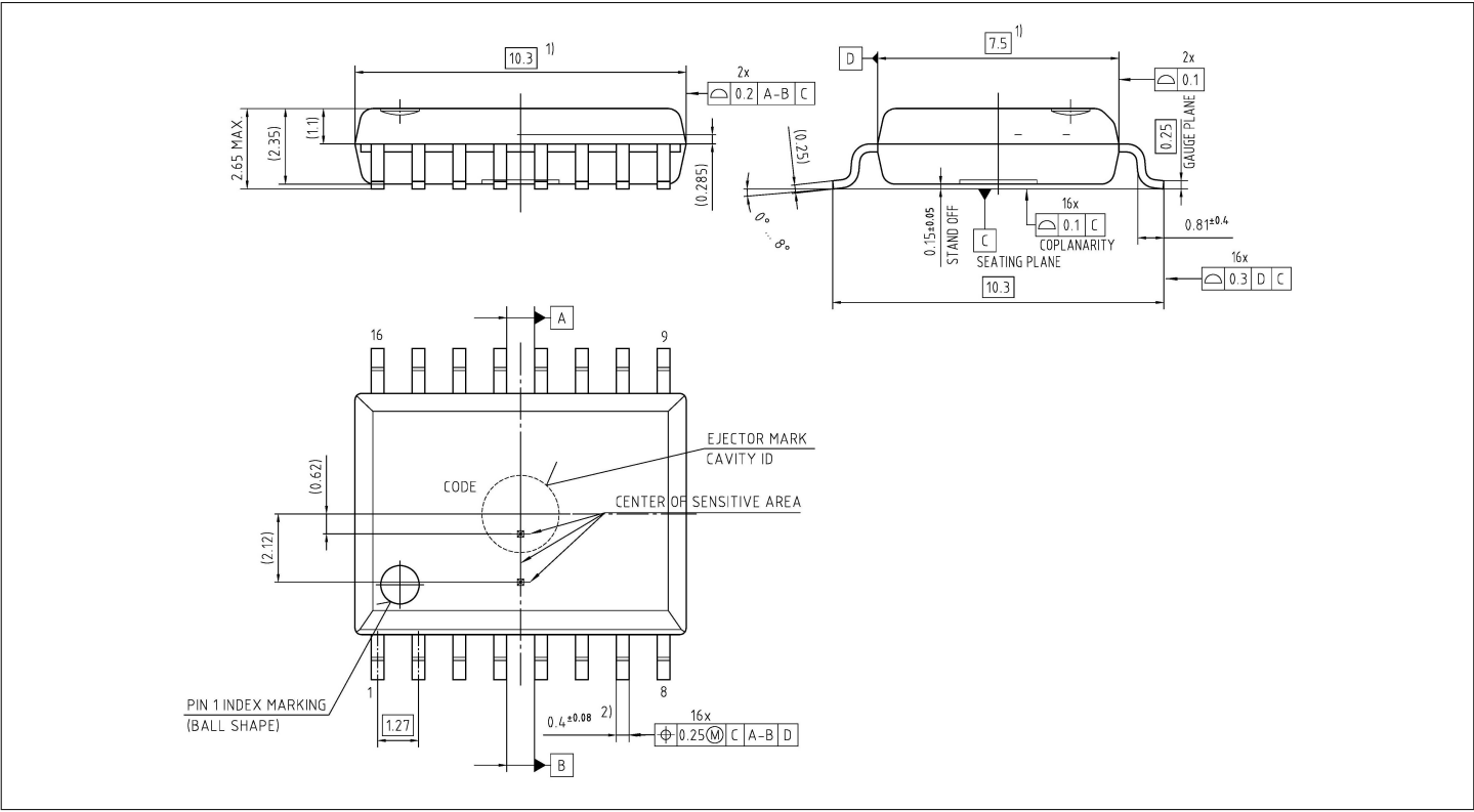
Figure 18 PG-DSO-16 package outline
