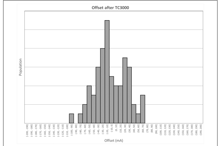
Figure 13 Population vs offset
