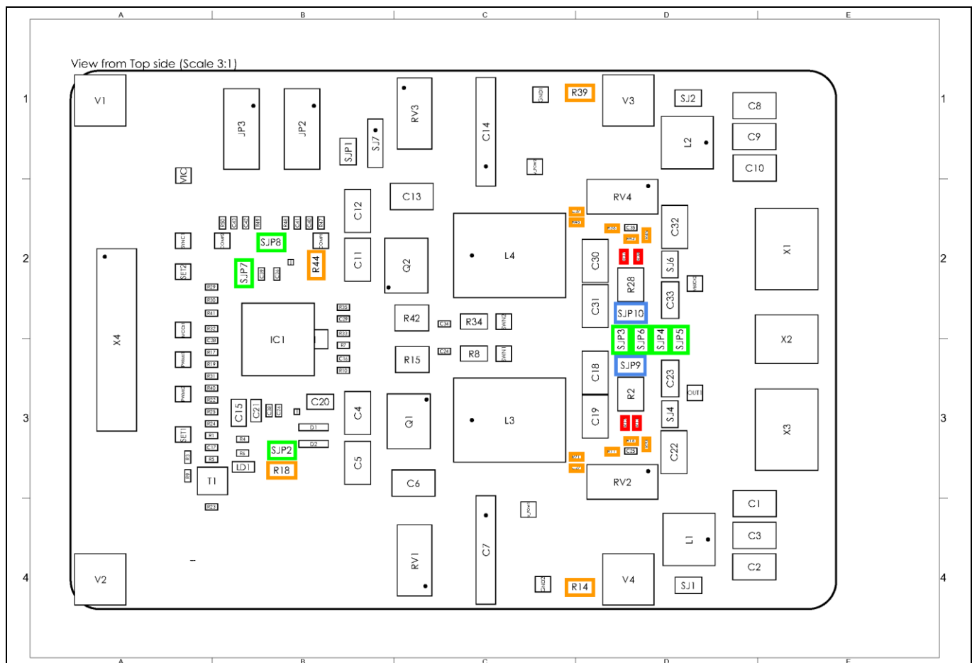
Figure 13 TLD5501-2 BUCK DEMO configuration for “Dual buck parallel voltage regulator” application
