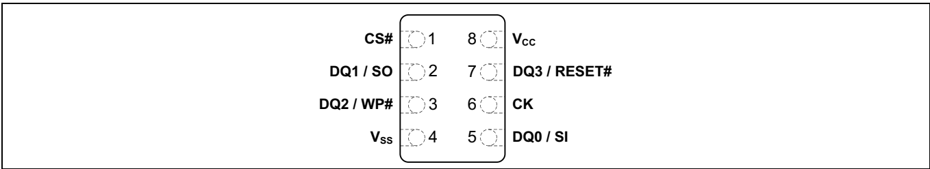
Figure 3 8-connector package (WSO6 6 × 8), top view
