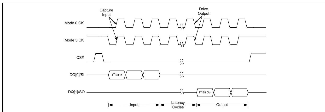
Figure 5 SPI SDR mode support
