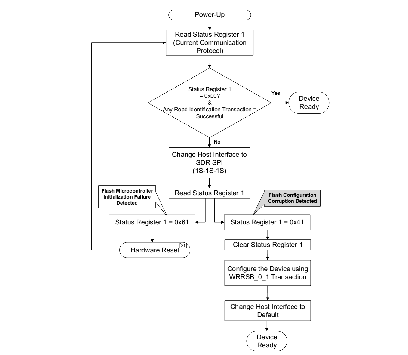
Figure 54 Host polling sequence for configuration corruption detection
