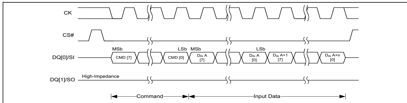
Figure 11 SPI program transaction with command and data input
