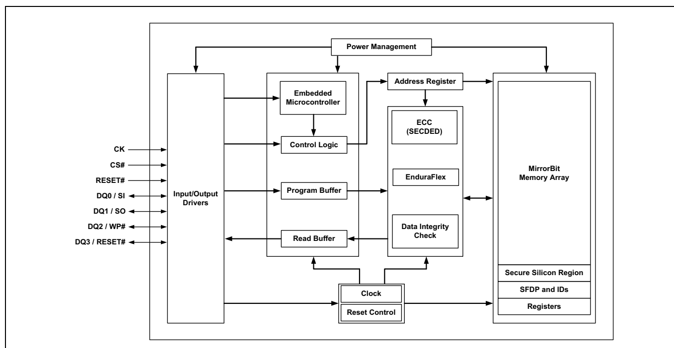
Figure 4 Logic block diagram
