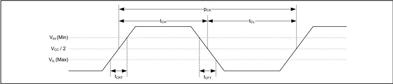
Figure 78 Clock timing
