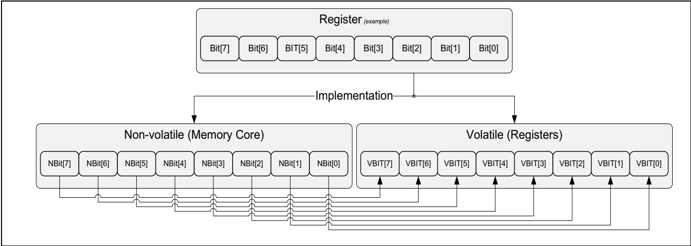
Figure 68 Register structure
