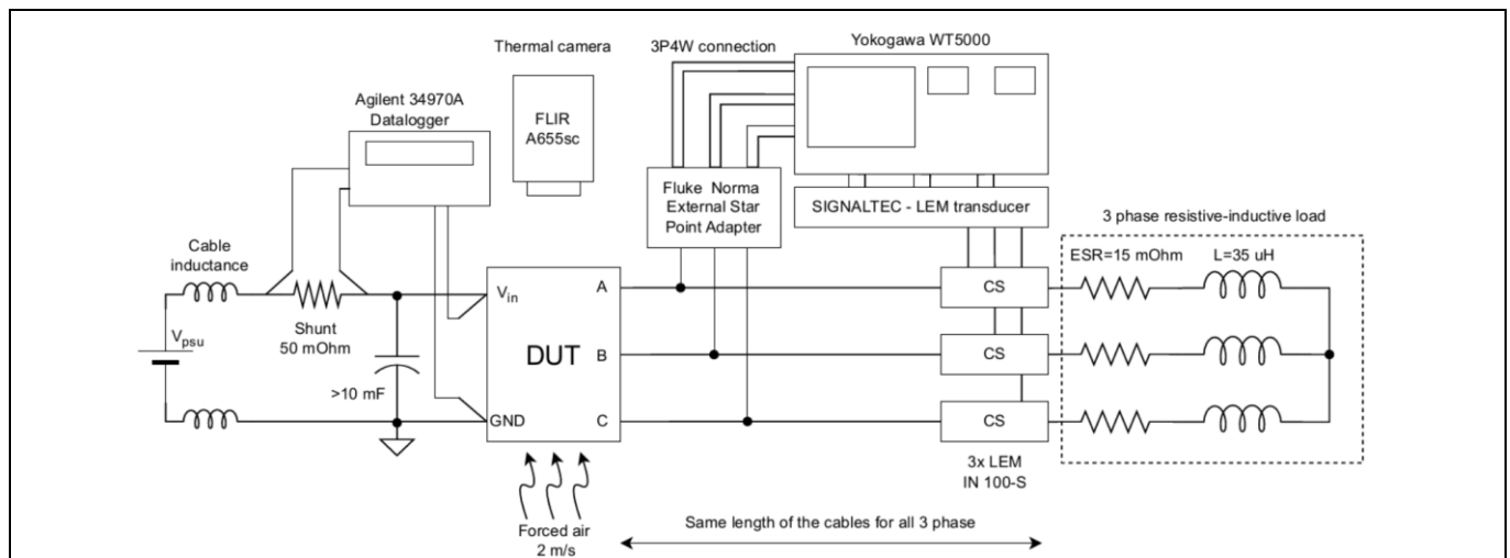
Figure 21 Measurement setup
