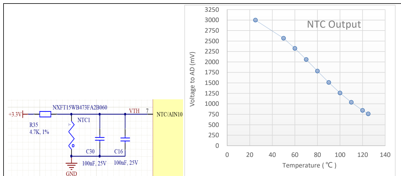
Figure 34 NTC circuit and output voltage curve
