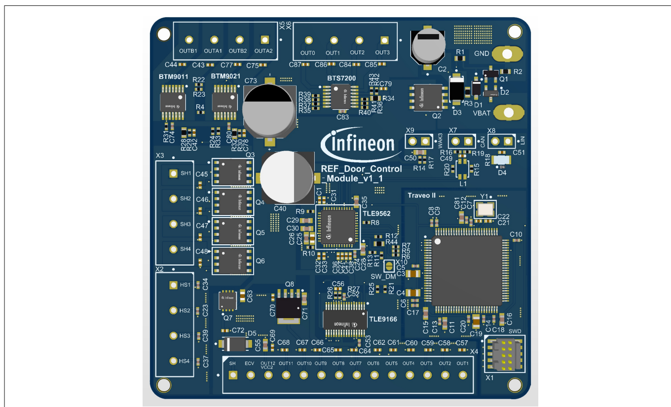
Figure 1 Door control reference design
