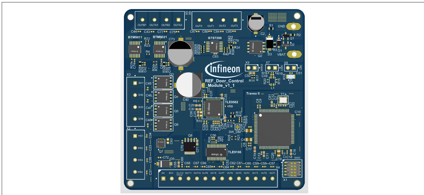
Figure 3 Infineon door control module reference design
