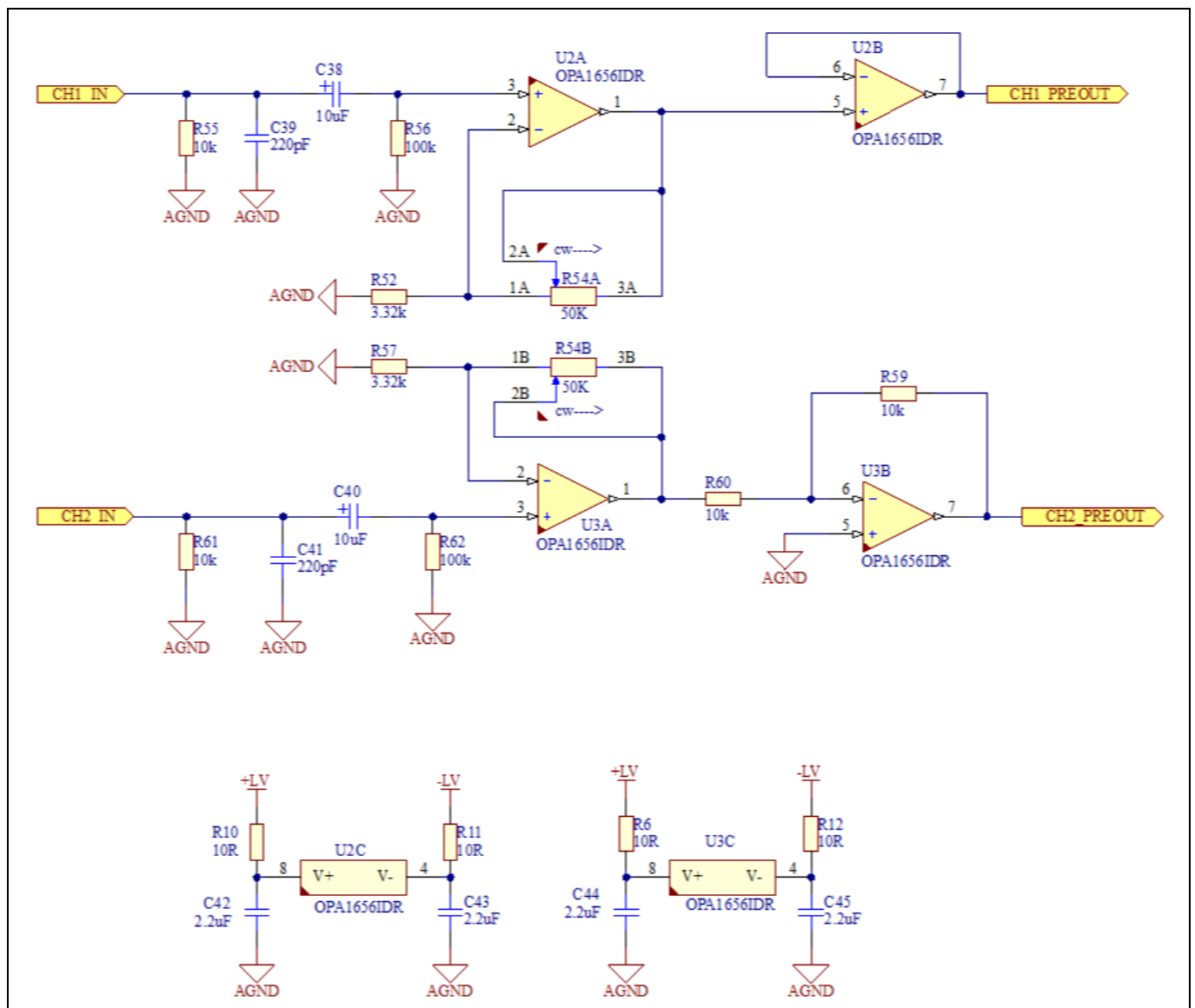
Figure 30 Preamplifier
