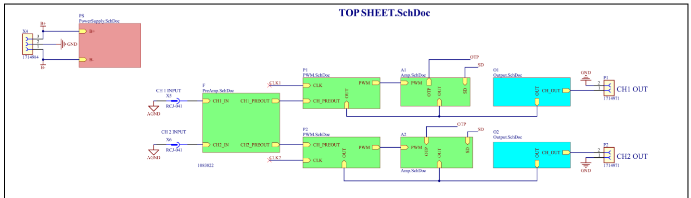
Figure 29 Signal chain
