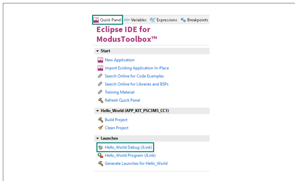
Figure 9 Debugging in ModusToolbox™ software
