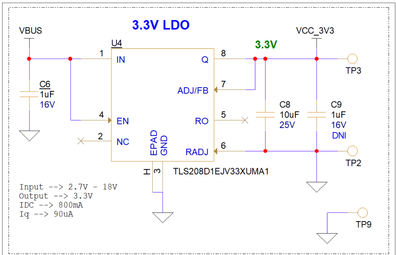
Figure 21 3.3V LDO
