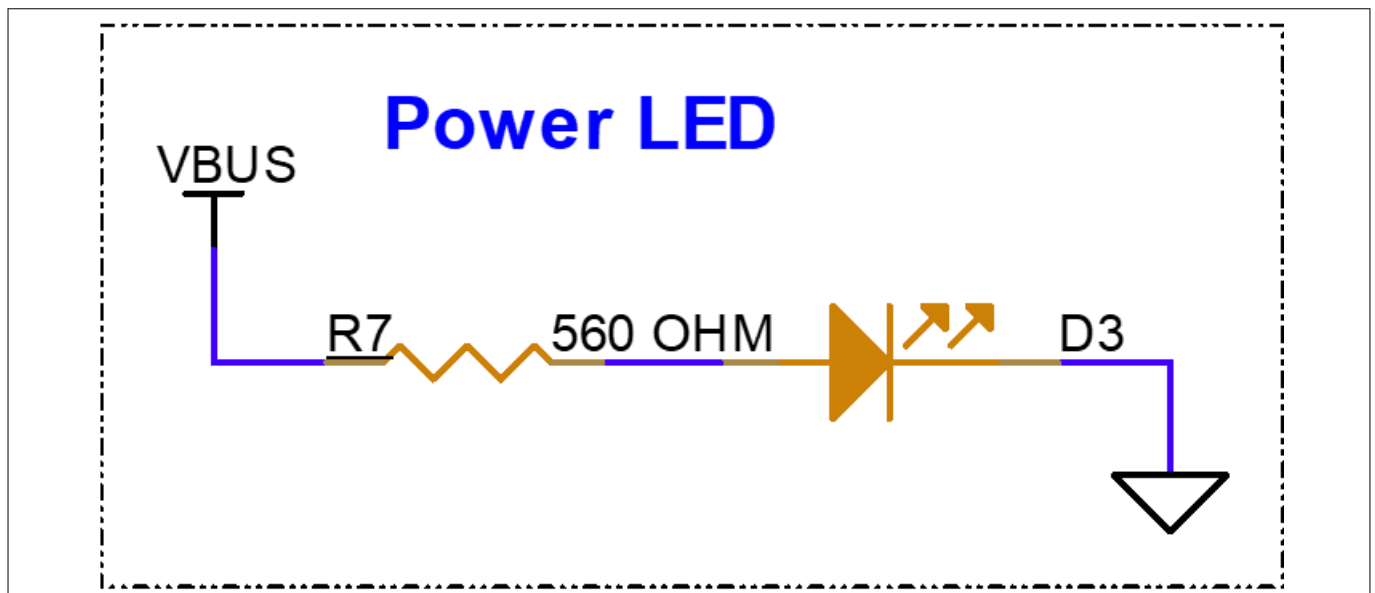
Figure 26 Power LED
