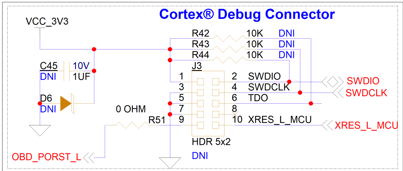
Figure 34 Cortex® debug connector
