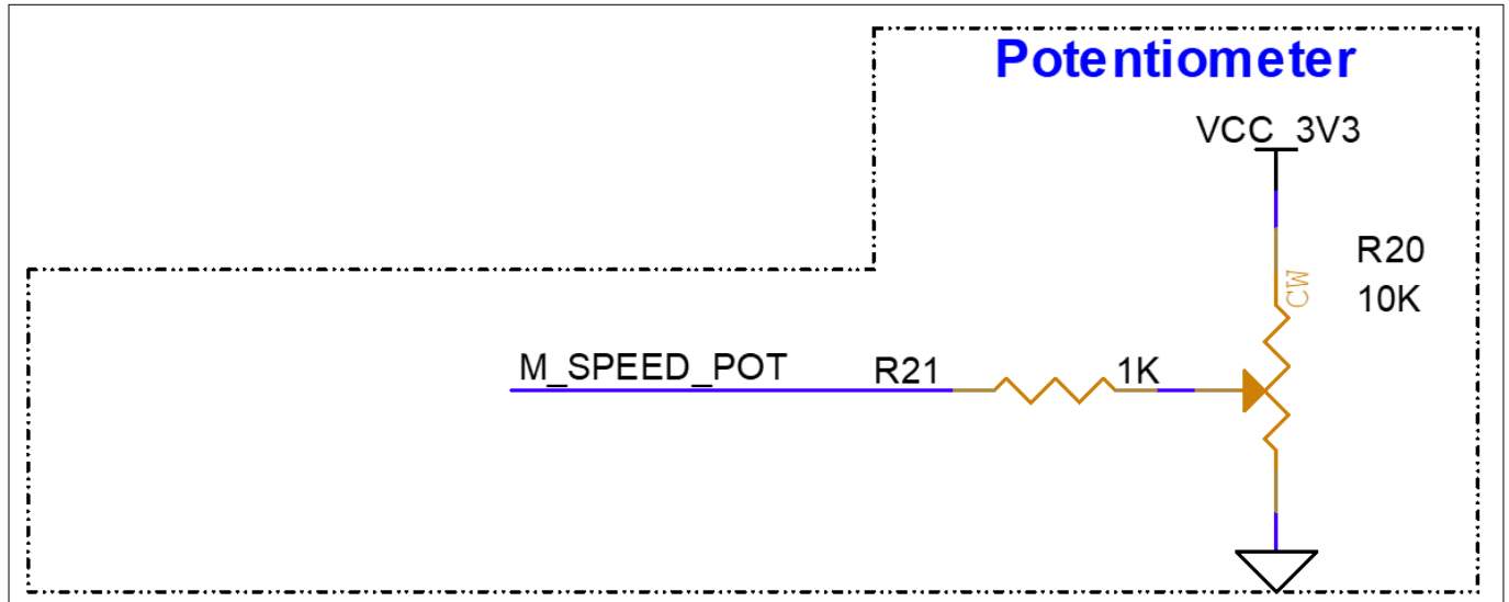
Figure 25 Potentiometer
