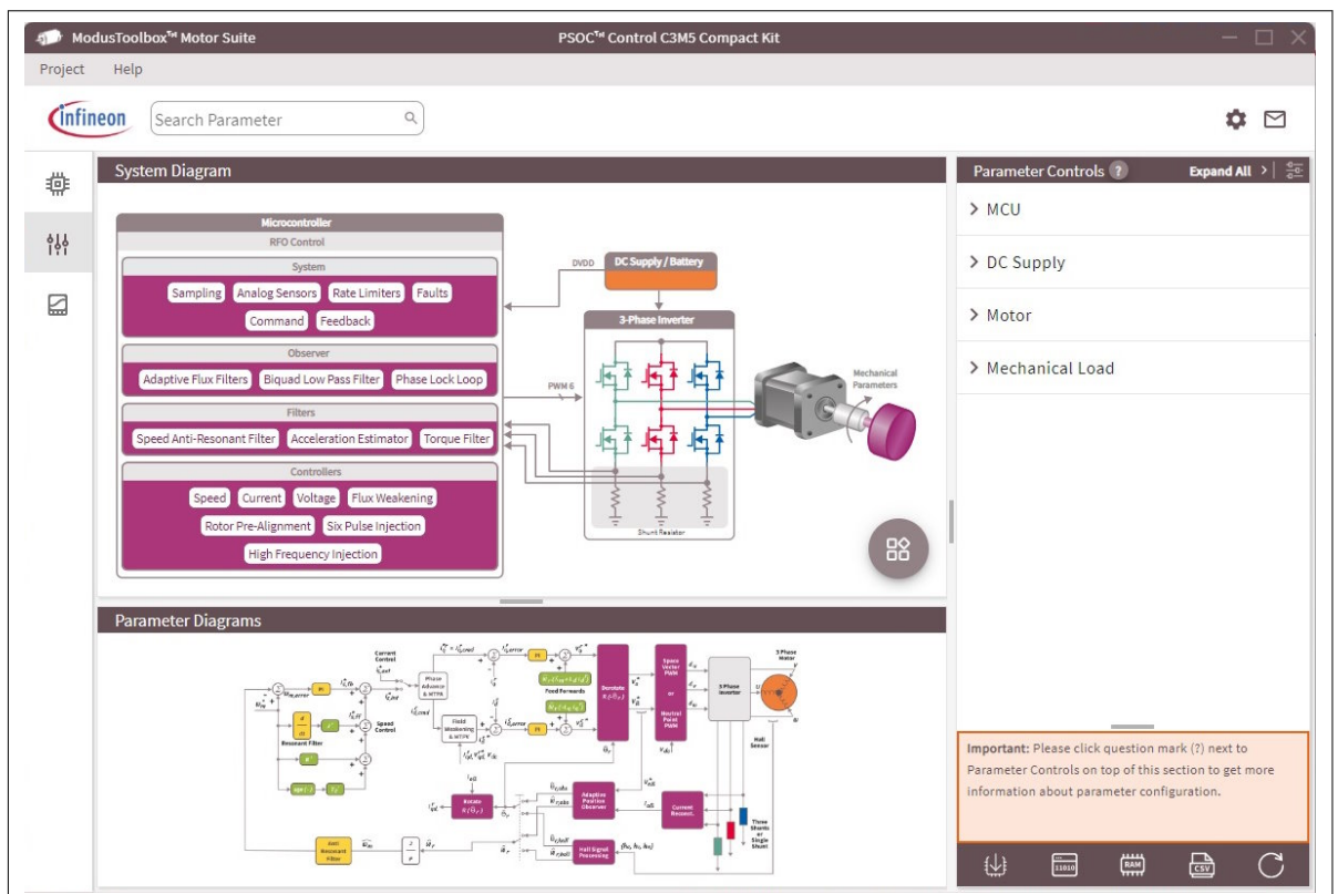
Figure 4 GUI: Configurator view
