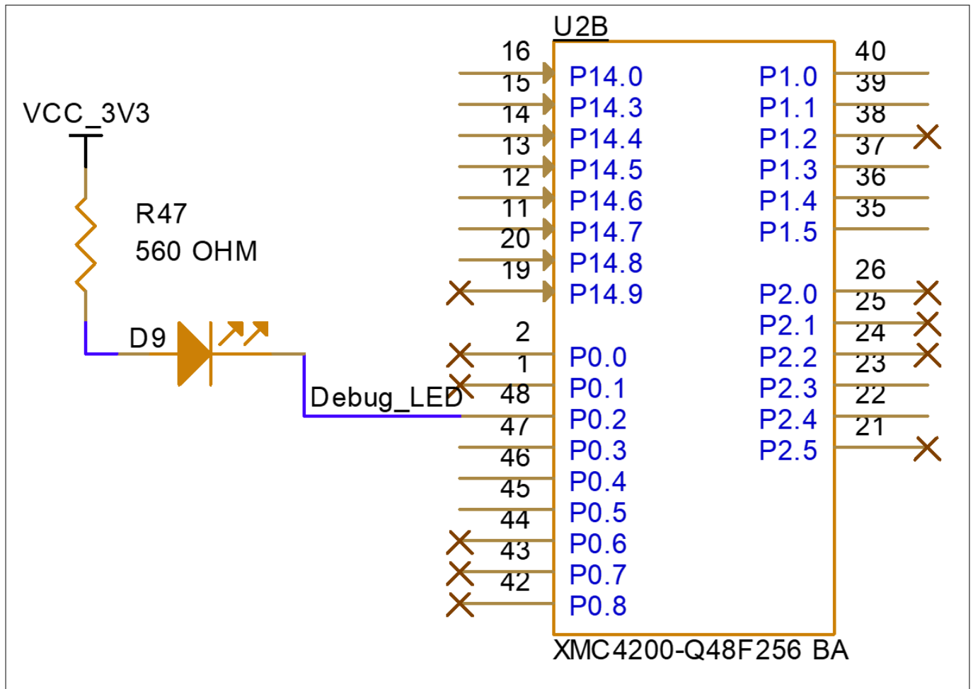
Figure 27 Debug LED
