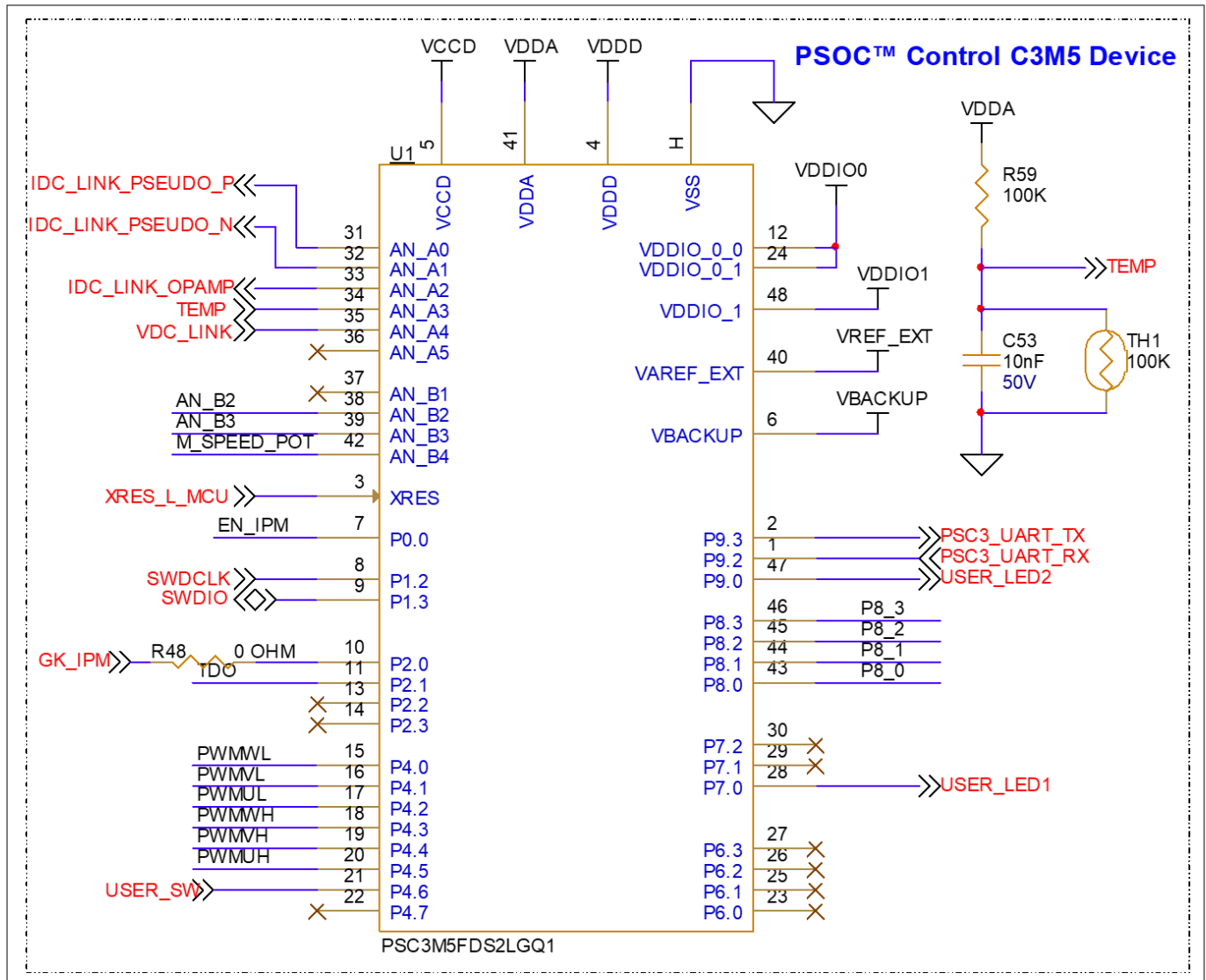
Figure 16 PSOC™ Control C3M5 device design
