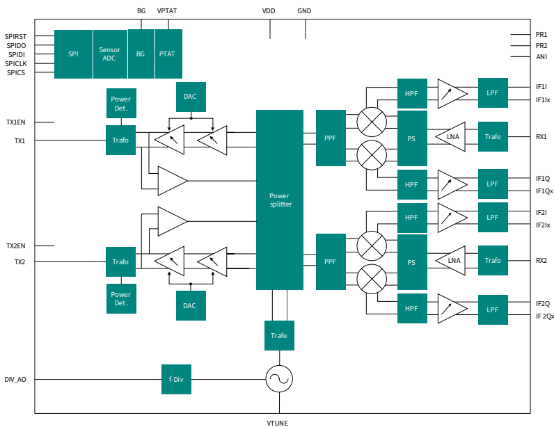
Block diagram of the BGT24LTR22
