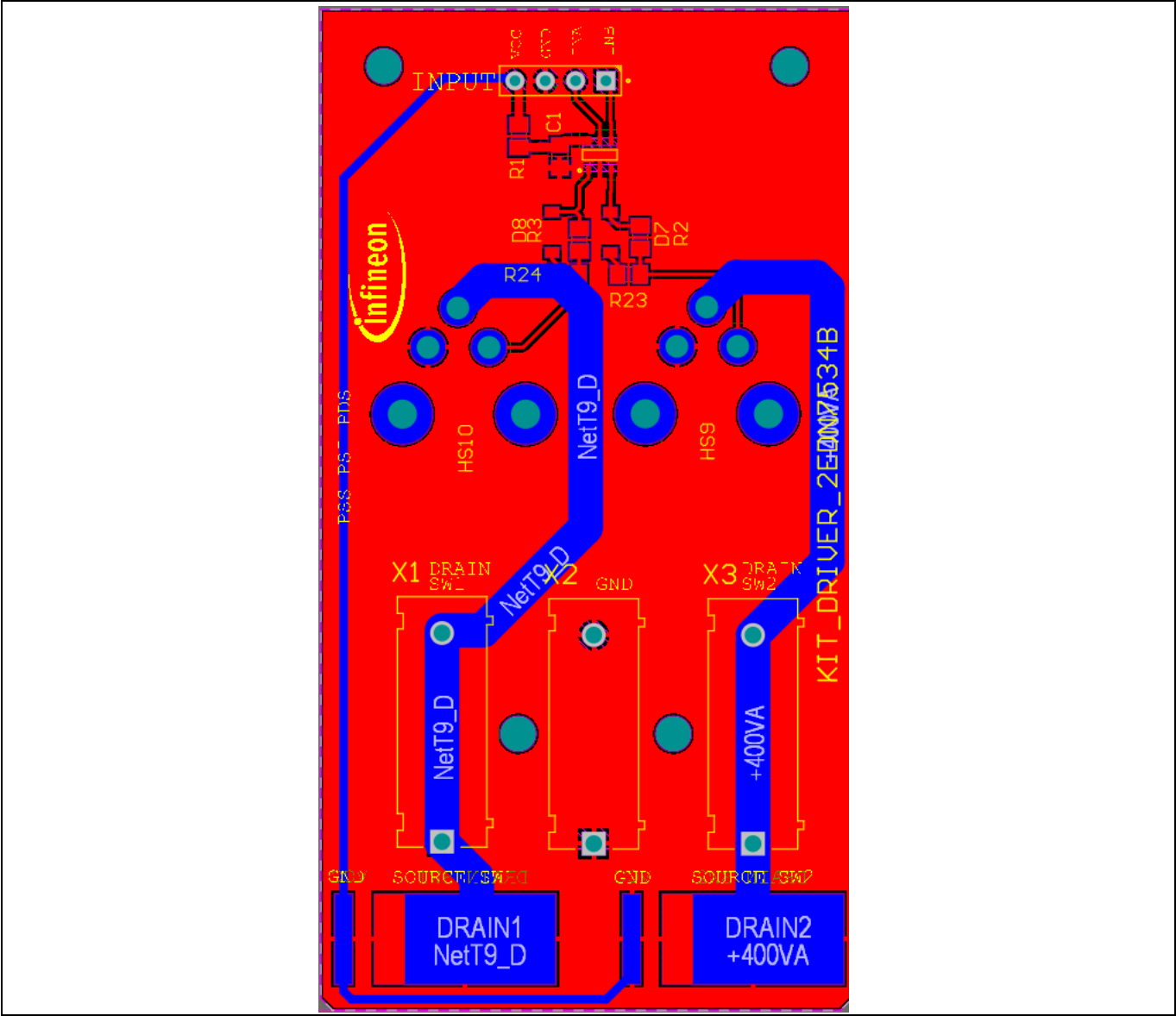
Figure 5 PCB traces
