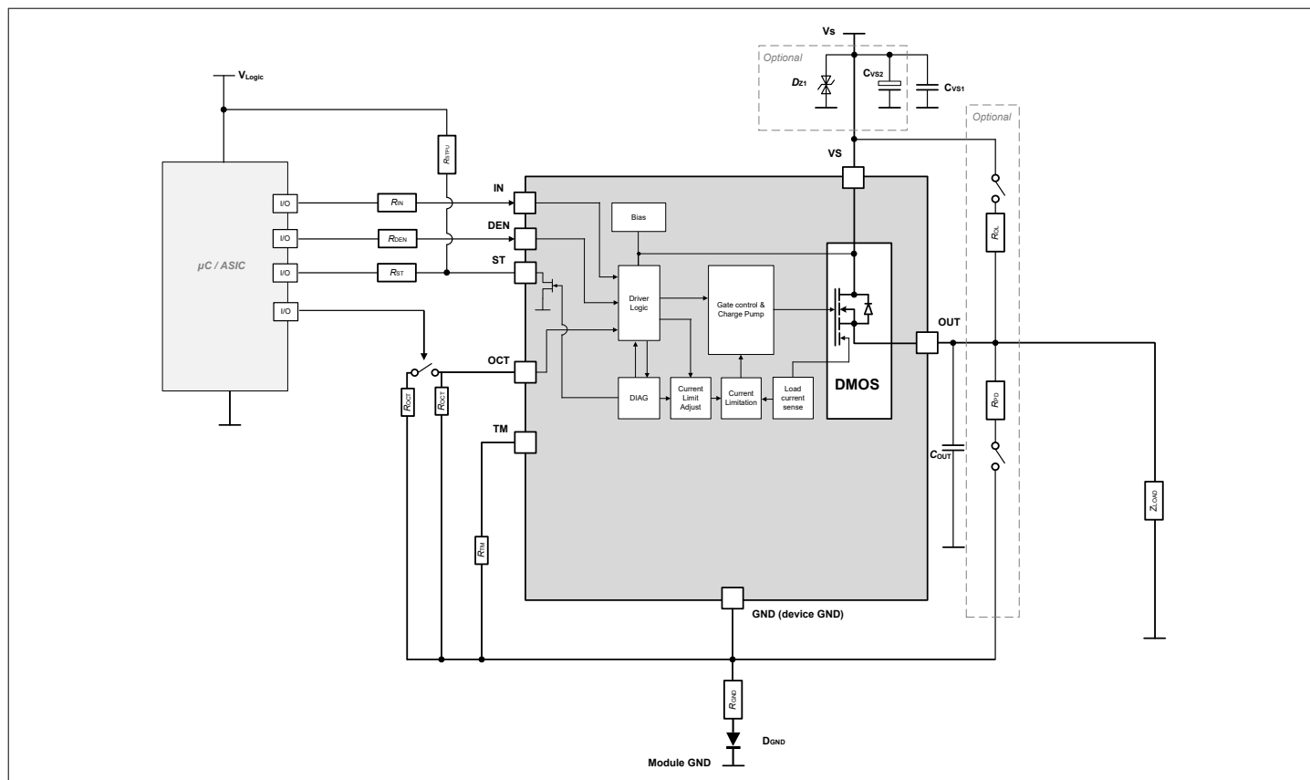
Figure 26 Application diagram with ITS4080S-EP-D controlled by logic levels [μC] with dynamic inrush current control
