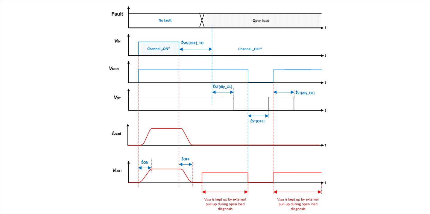
Figure 22 Behavior and timings of the extended diagnostic “open load detection” (the usage of a DEN - controlled switchable pull-up resistor from OUT to V_S in OFF-state is assumed)
