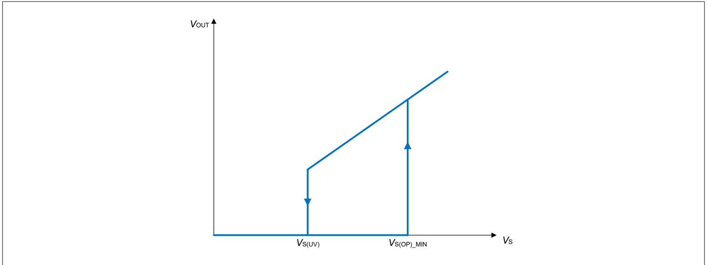
Figure 16 Undervoltage behavior
