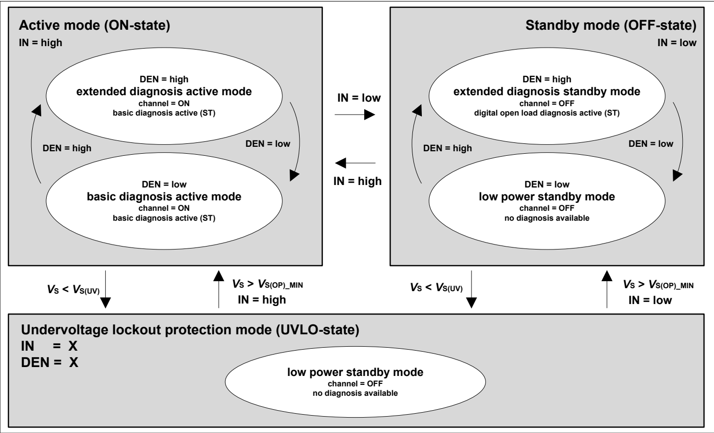
Figure 6 State diagram ITS4080S-EP-D
