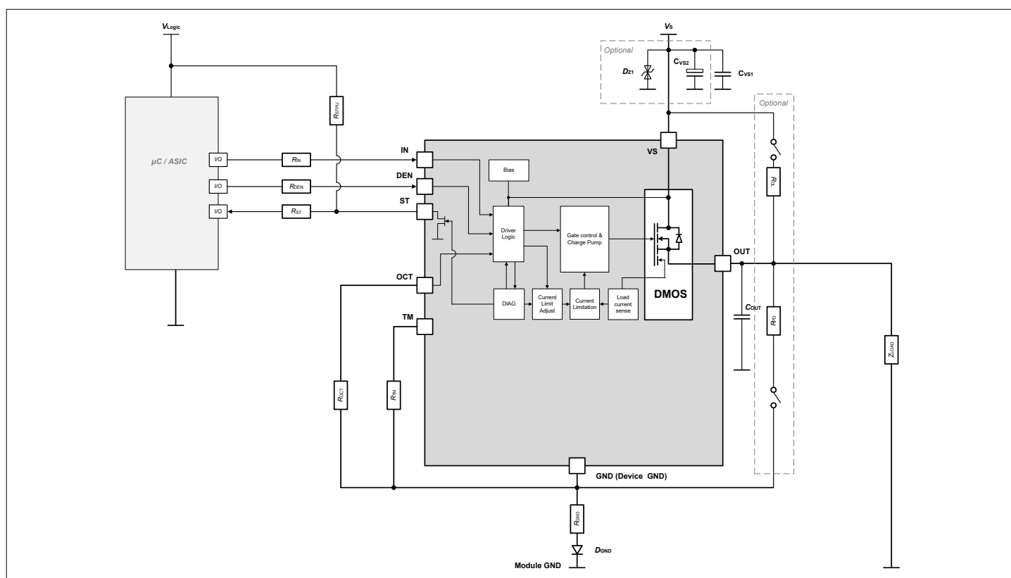
Figure 25 Application diagram with ITS4080S-EP-D
