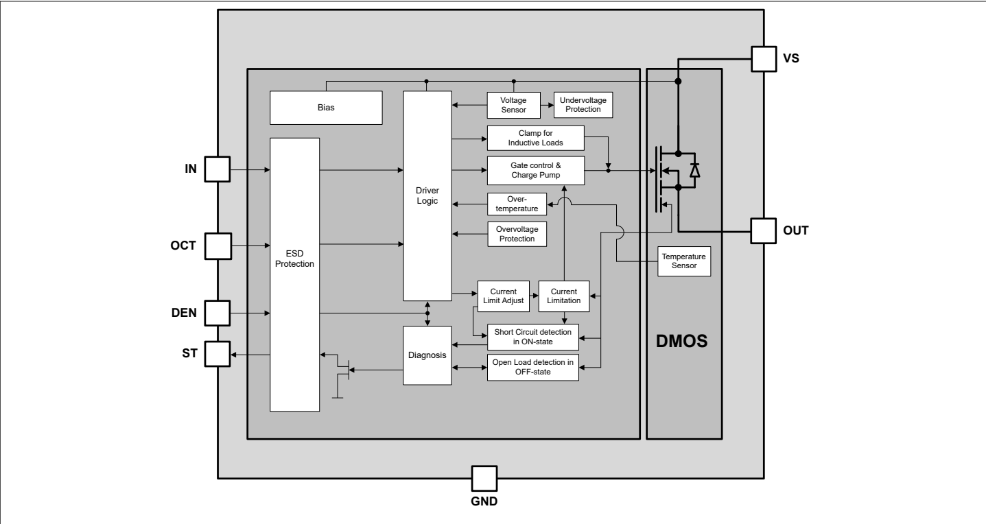
Figure 1 Block diagram ITS4080S-EP-D
