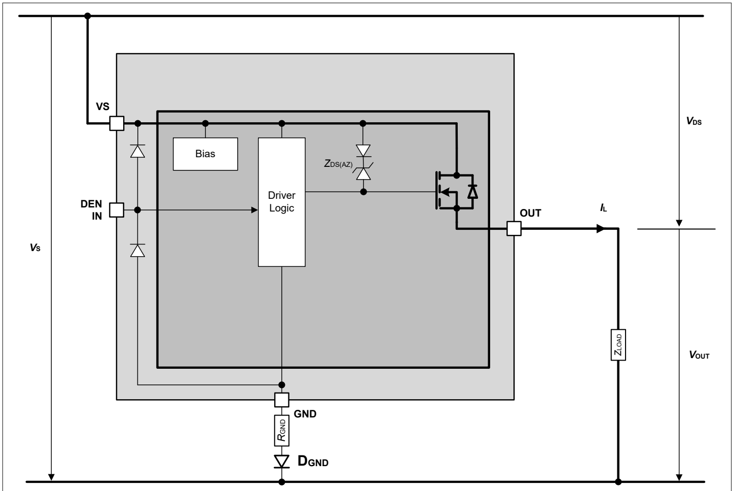
Figure 9 Output clamp ITS4080S-EP-D
