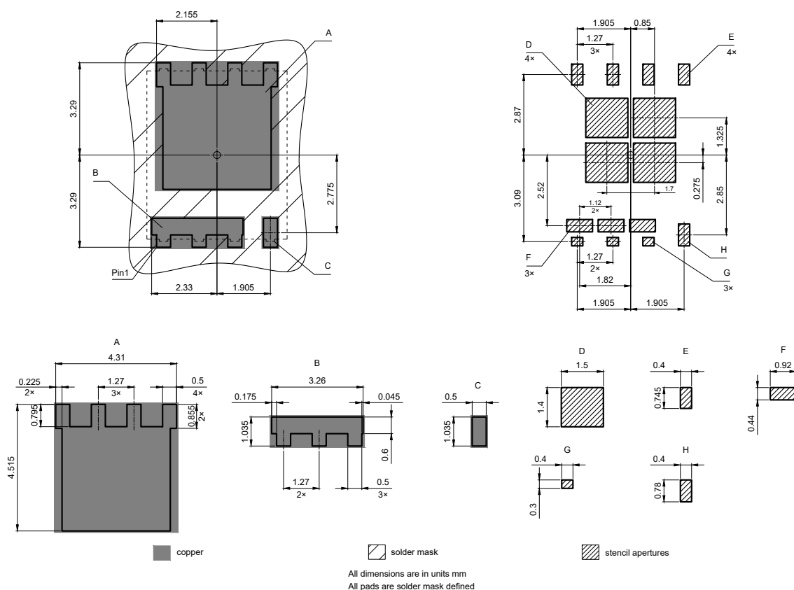
Figure 2 Outline PG-TDSON-8, dimensions in mm
