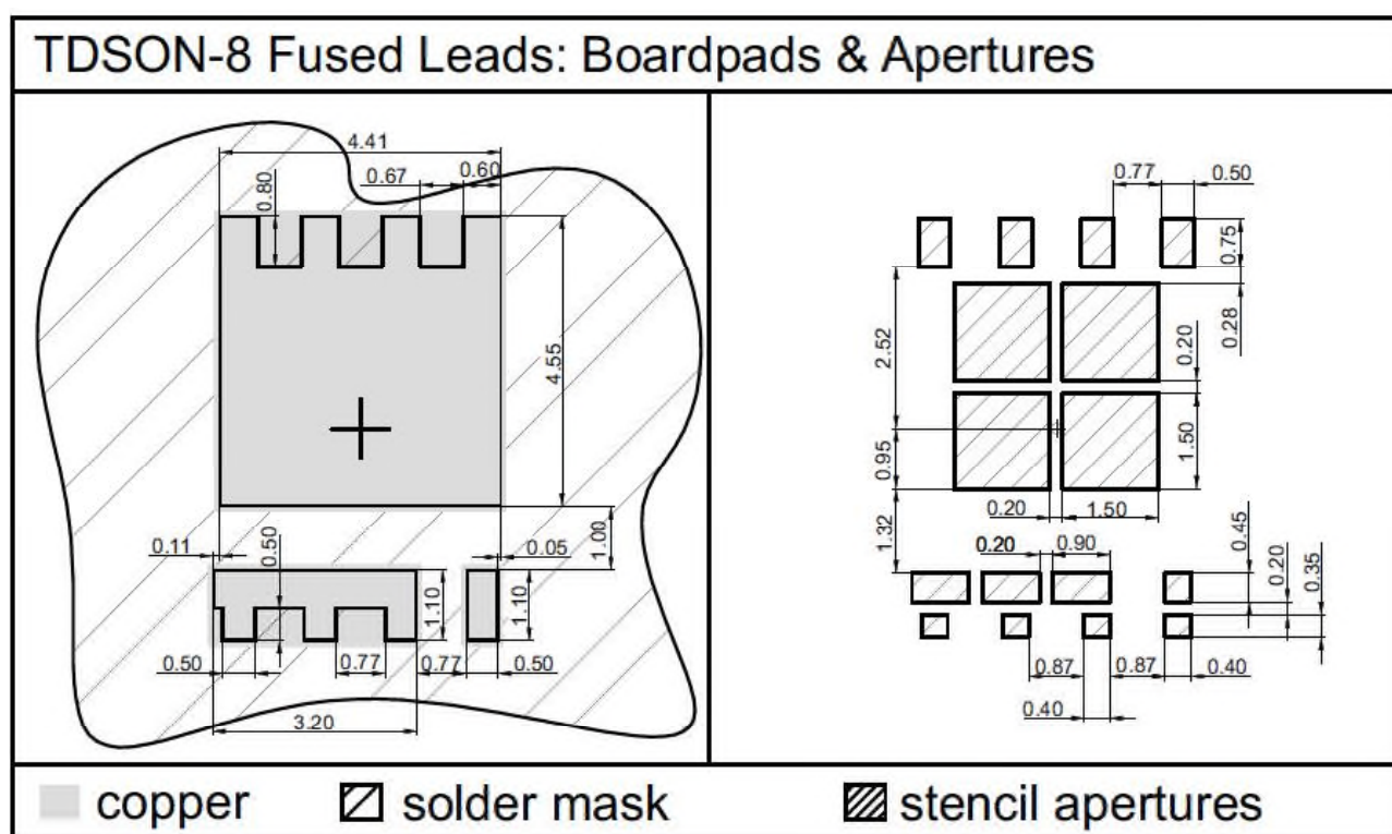
Figure 3 Outline PG-TDSON-8, dimensions in mm
