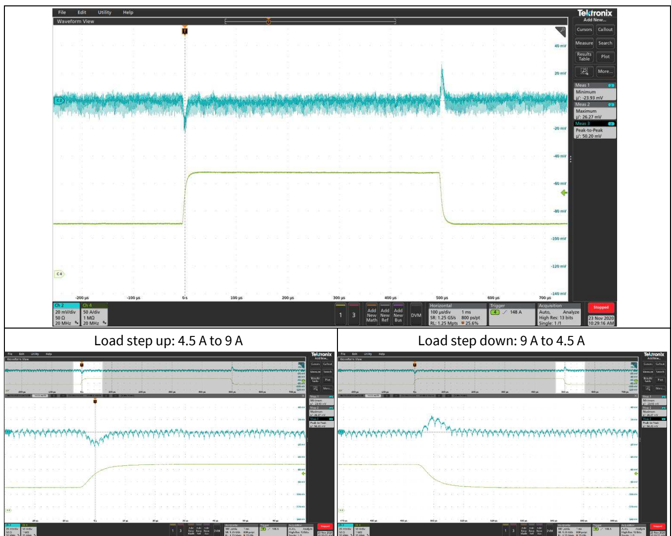
Figure 19 Transient response at 4.5 A step load current: I_o = 4.5 \text{ A} - 9 \text{ A} , (Ch2: Vo, Ch4: I_o ), pk-pk: 50.2 mV, fsw = 600 kHz
