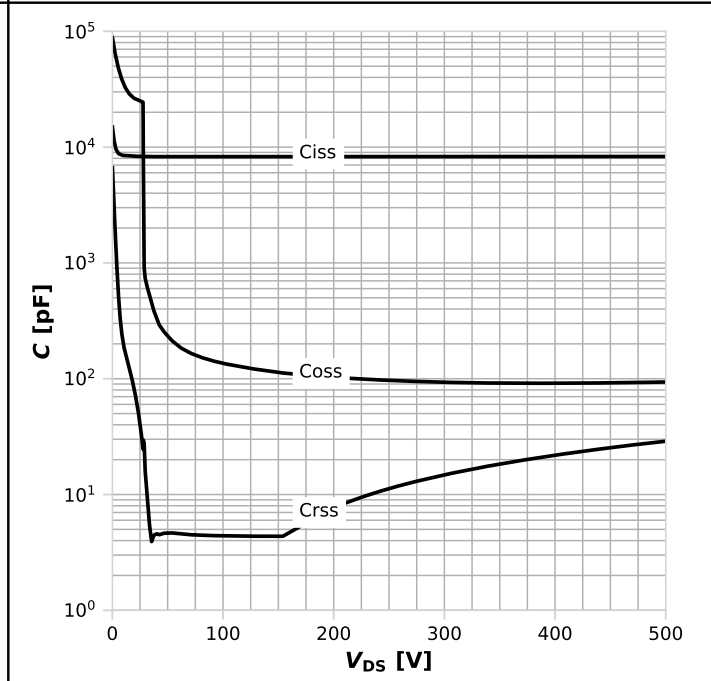
Diagram 14: Typ. capacitances
