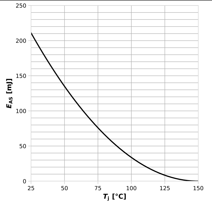
Diagram 12: Avalanche energy
