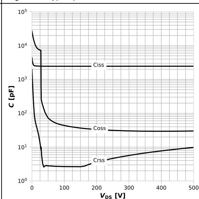
Diagram 14: Typ. capacitances
