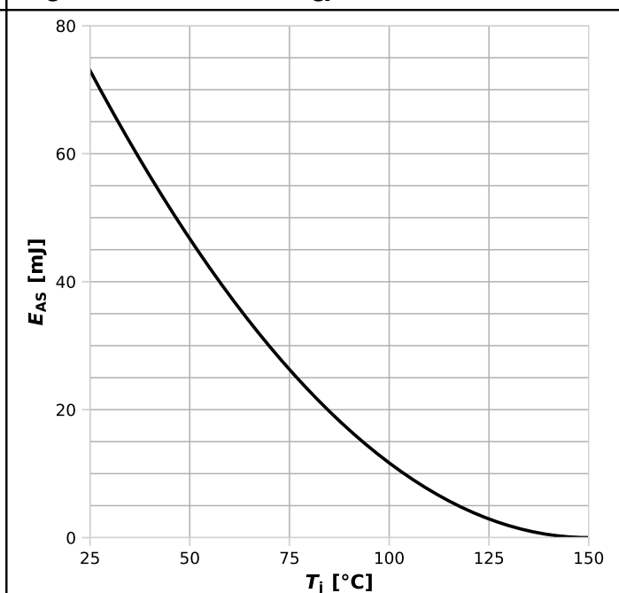
Diagram 12: Avalanche energy
