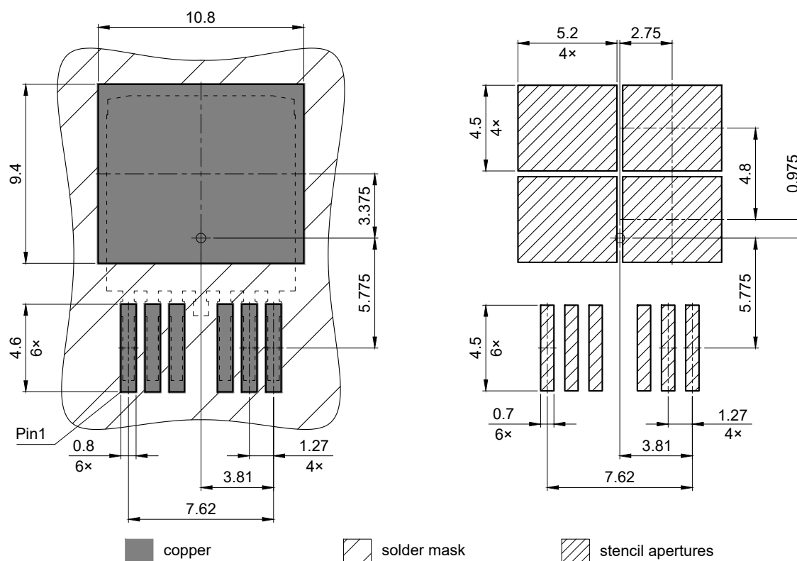
Figure 2 Outline PG-TO263-7, dimensions in mm
