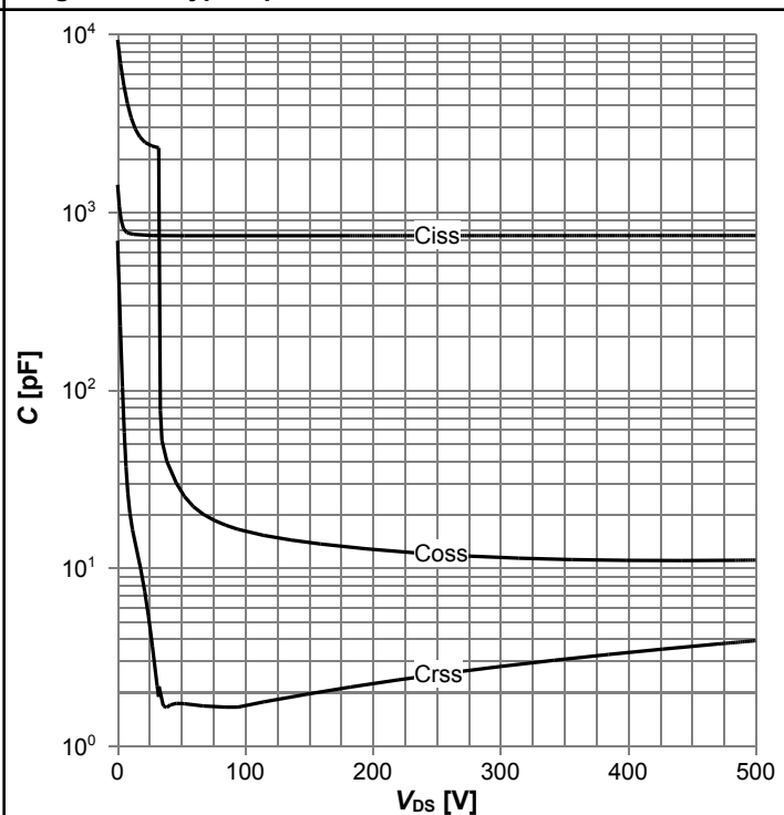
Diagram 14: Typ. capacitances
