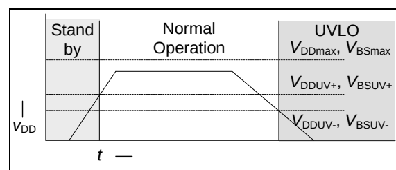
Figure 4: Operation modes
