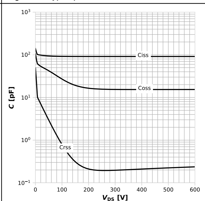
Diagram 18: Typ. capacitances
