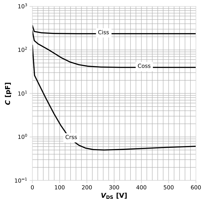
Diagram 18: Typ. capacitances
