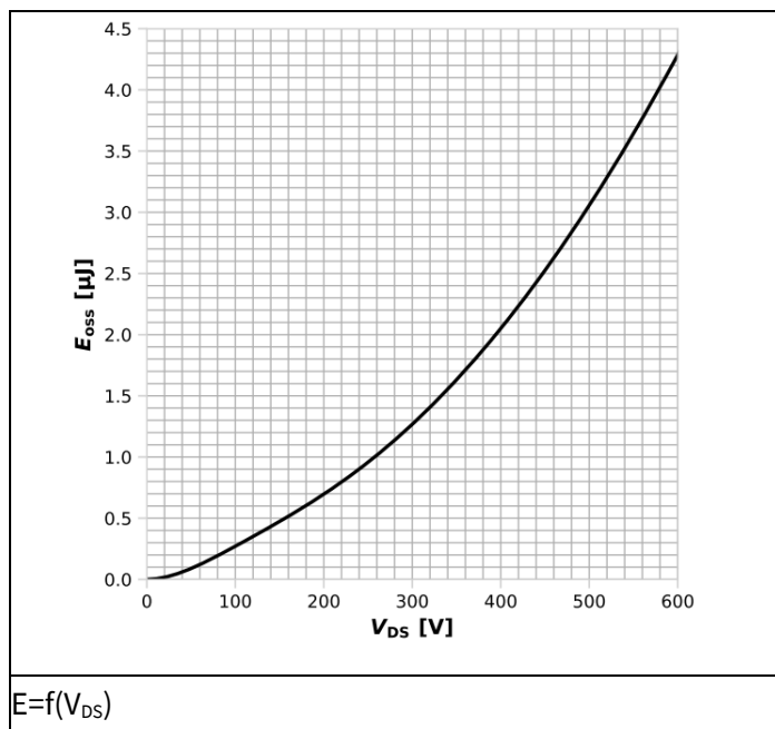
Figure 13 Typical output energy (single switch)
