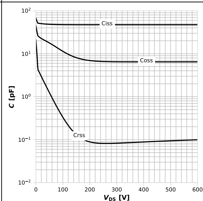
Diagram 18: Typ. capacitances
