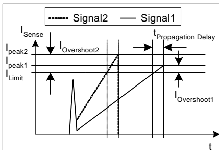
Figure 20 Current Limiting
