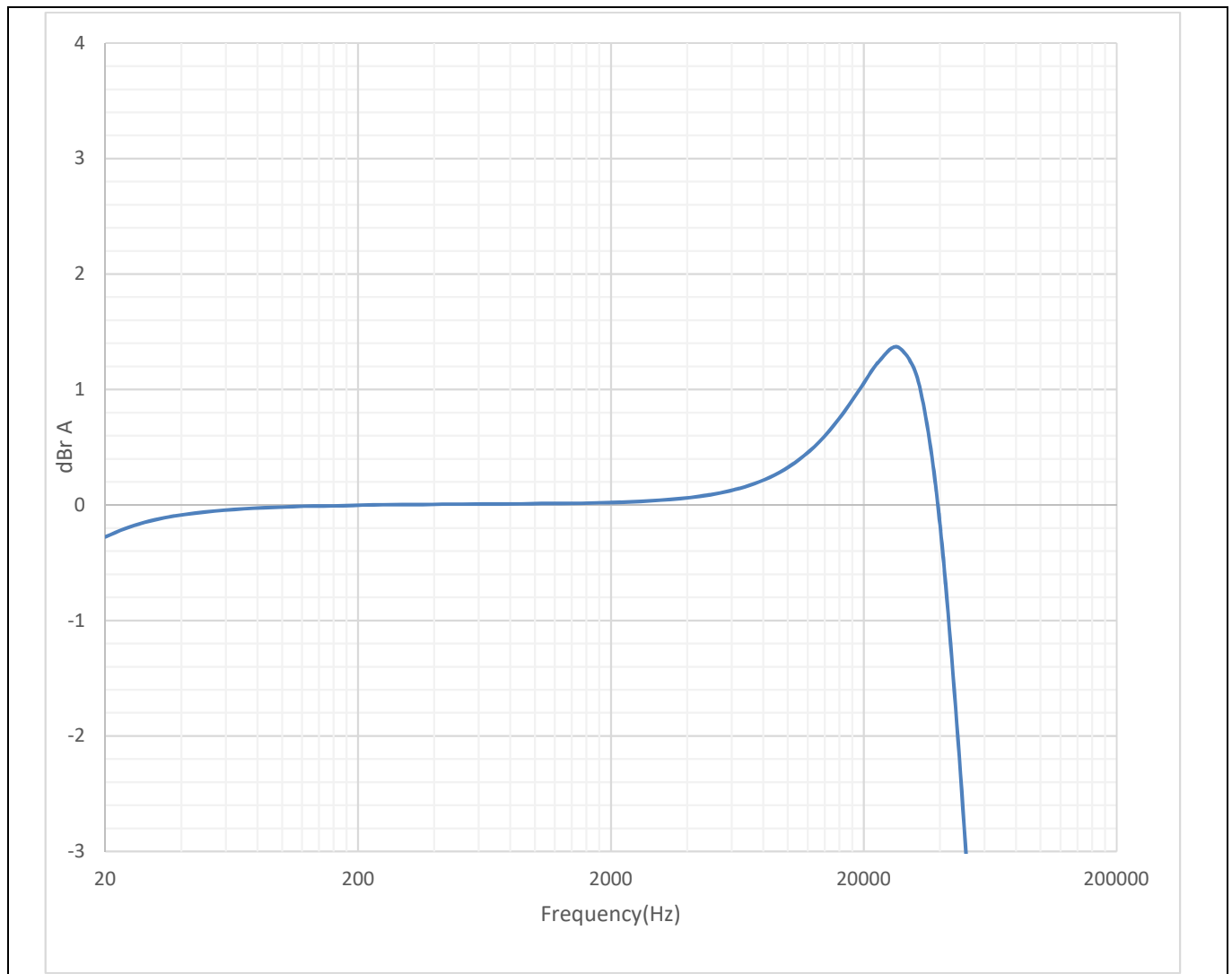
Figure 5 Frequency response 2 Ω load
