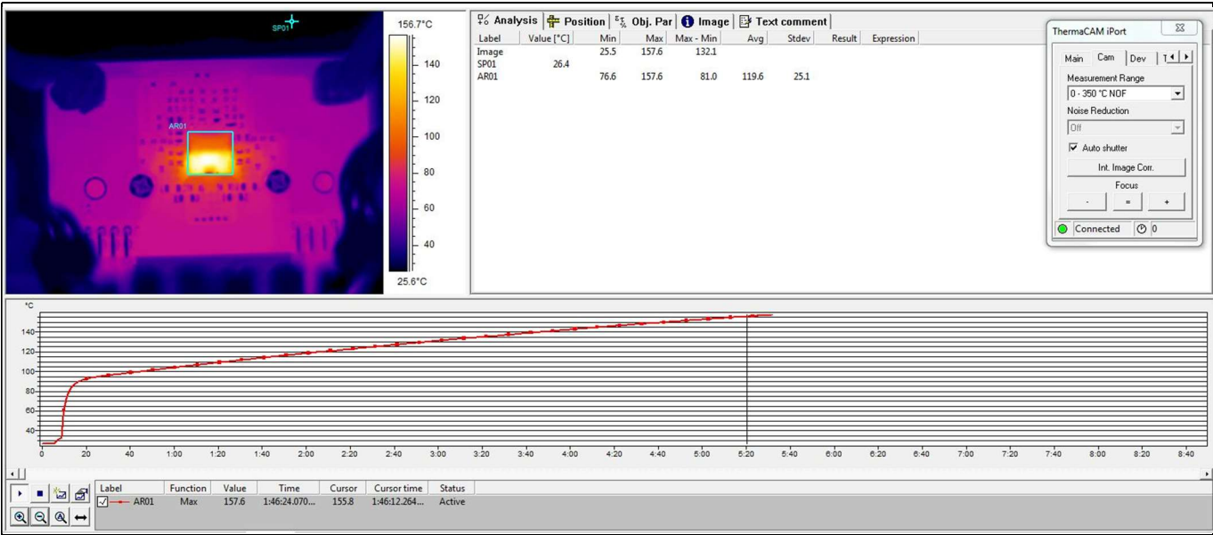
Figure 10 Peak power P_{out} = 190\text{ W} with 6\ \Omega load \pm 44\text{ V}
