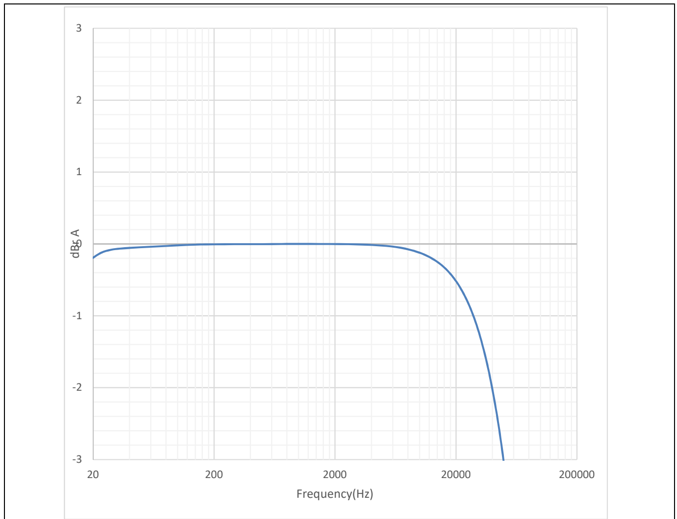
Figure 5 Frequency response 2 Ω load
