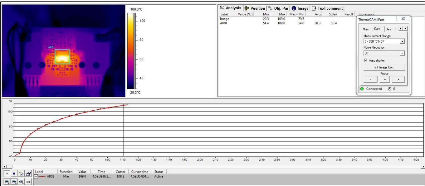
Figure 13 Peak power P_{out} = 102\text{ W} with 4\ \Omega load \pm 30\text{ V}
