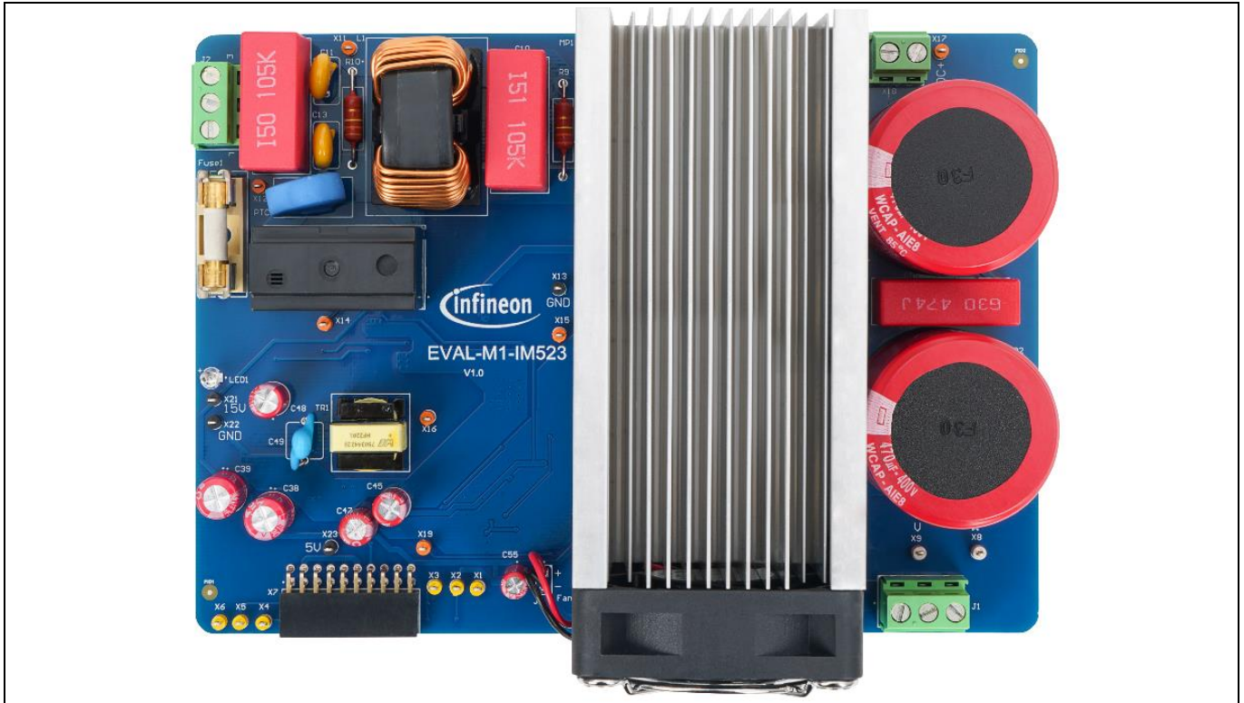
Figure 15 Top-assembly PCBA of the EVAL-M1-IM523
