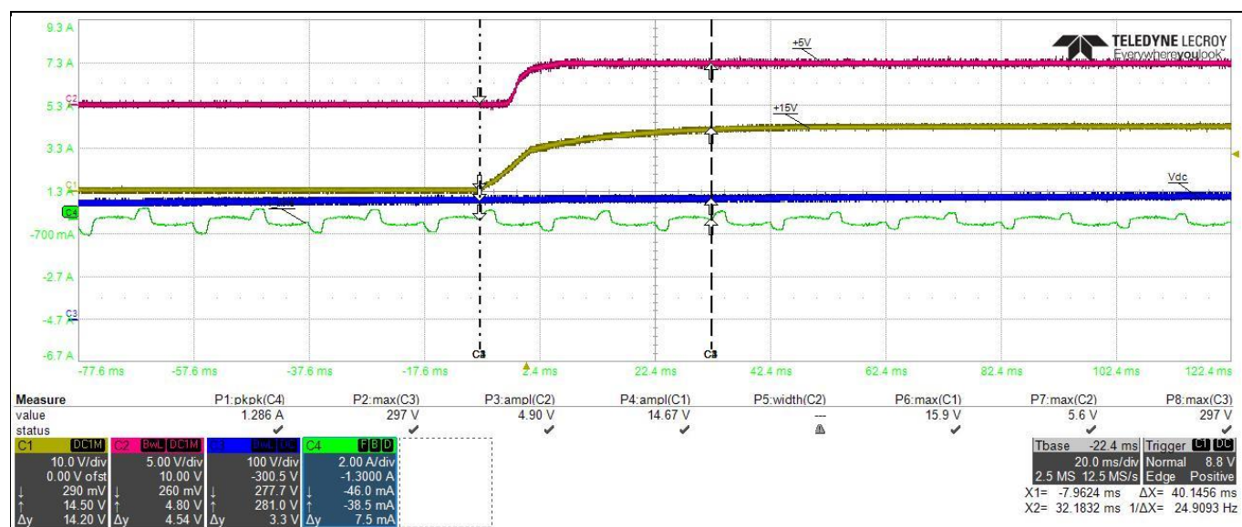
Figure 17 Power supply voltage (15 V & 5 V)
