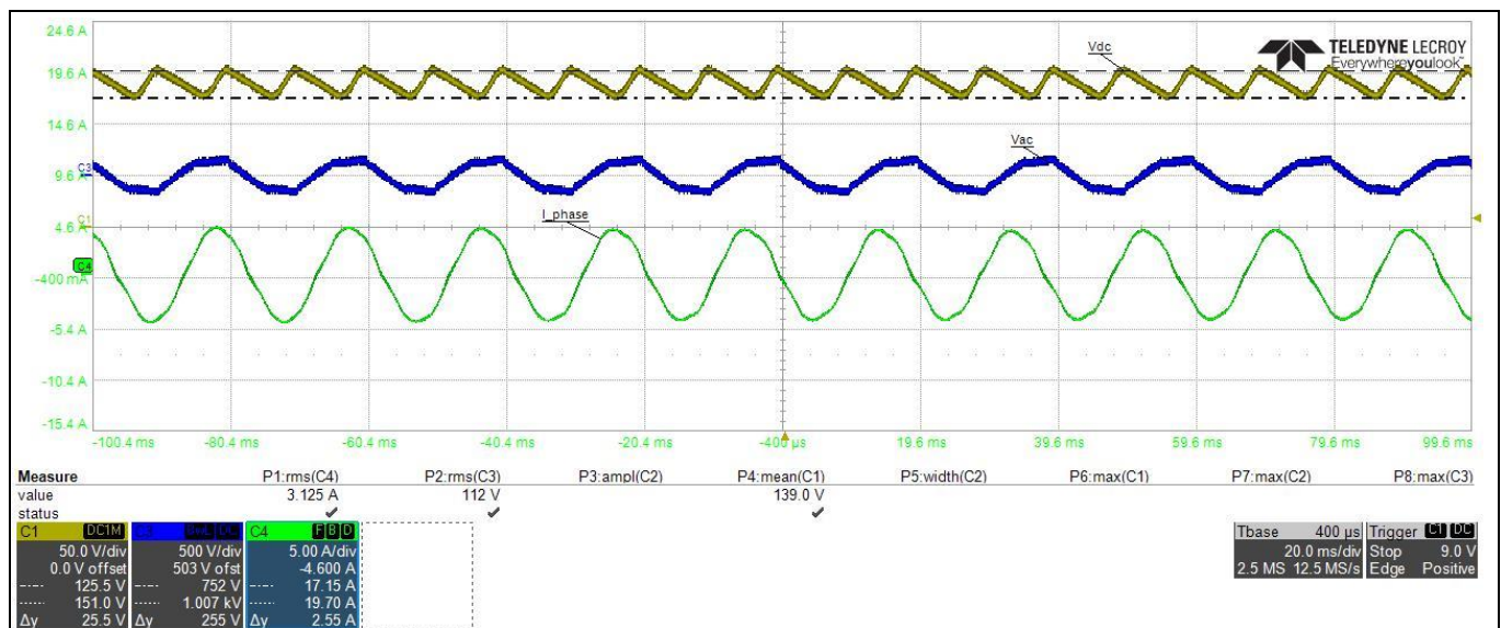
Figure 23 110 V AC input, V DC bus voltage ripple
