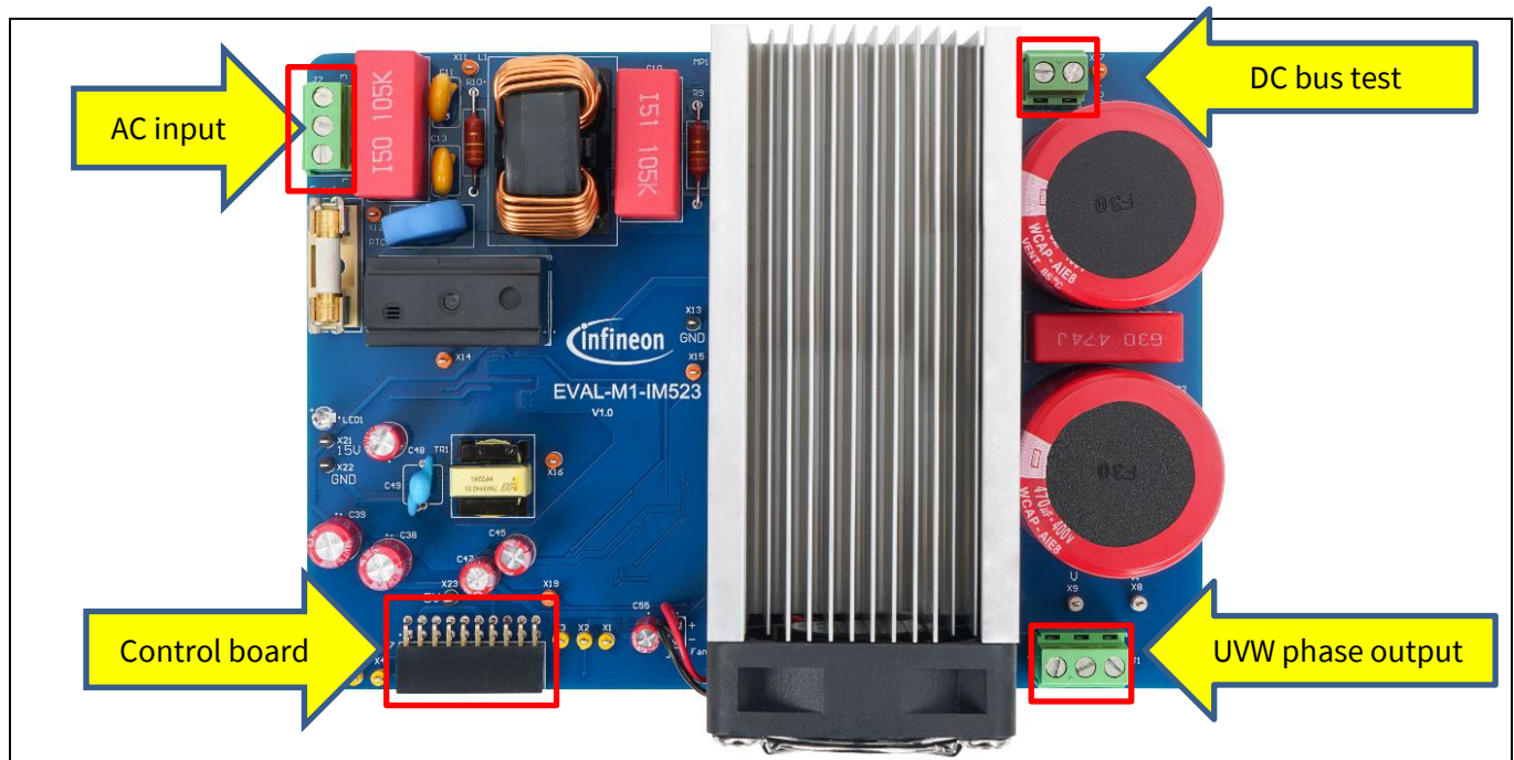
Figure 4 Example of the system connection
