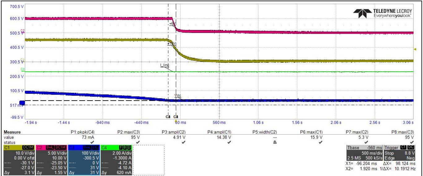
Figure 19 Input 85 V AC
