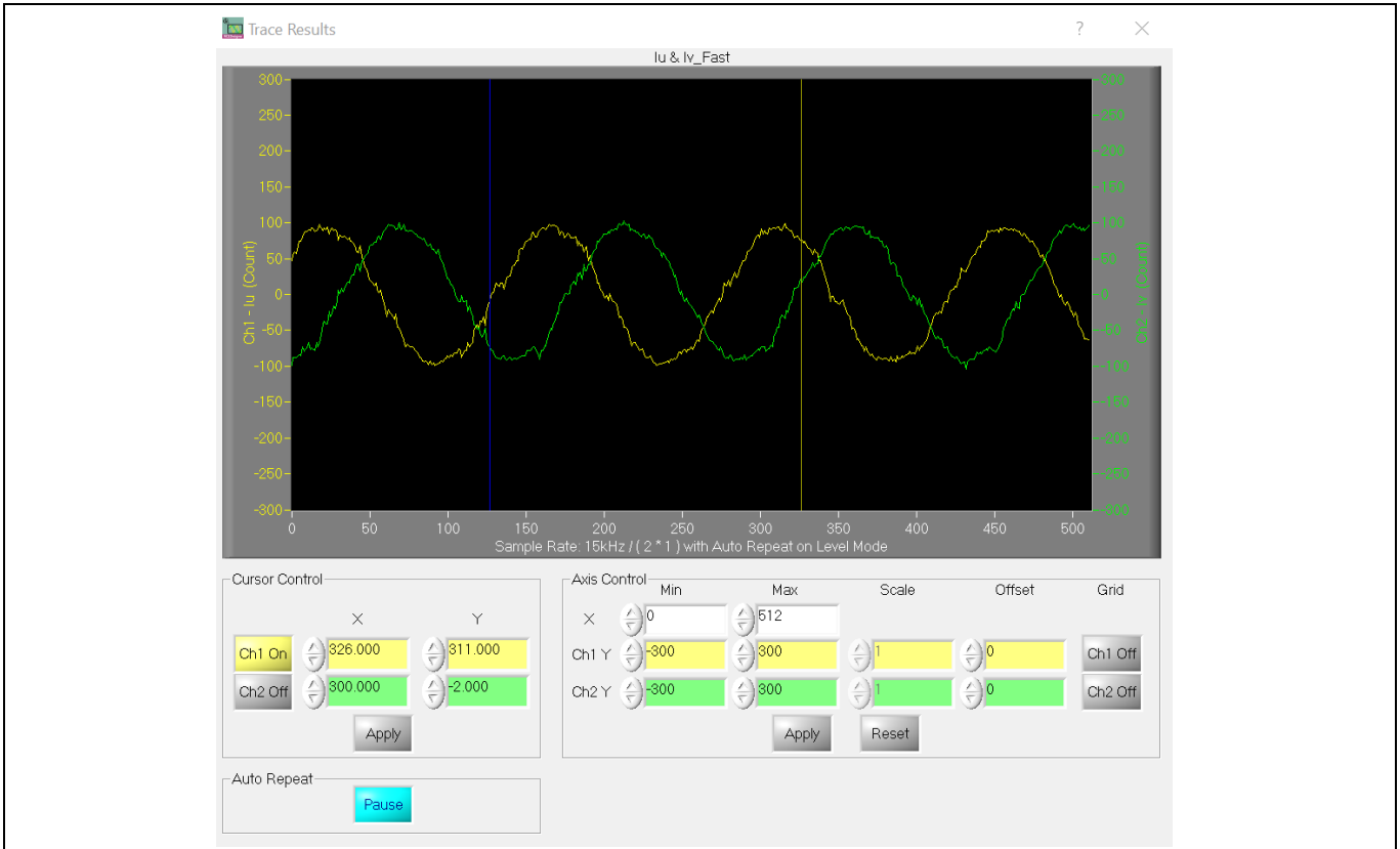
Figure 37 500 W load current feedback, 3 A rms phase current, 15 kHz PWM, 220 V AC input
