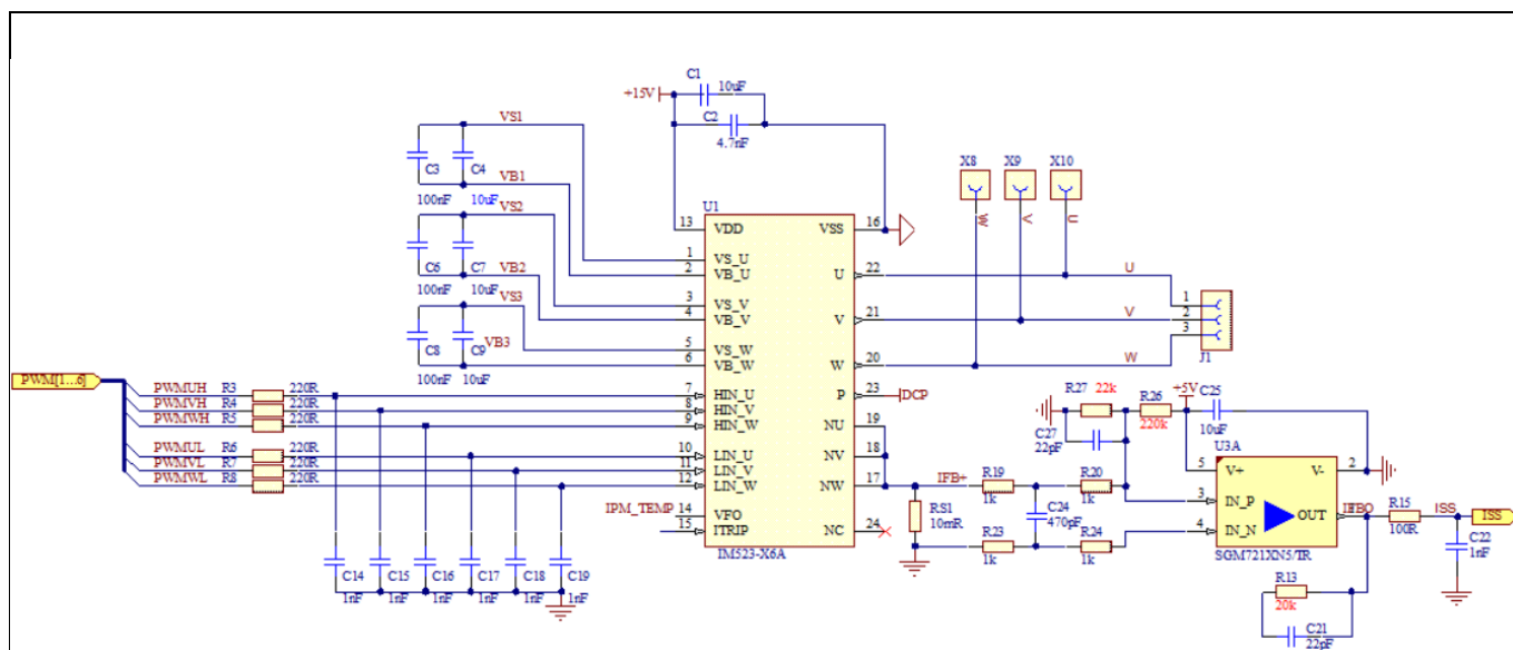
Figure 13 Schematics for the IM523-X6A IPM and peripheral circuit
