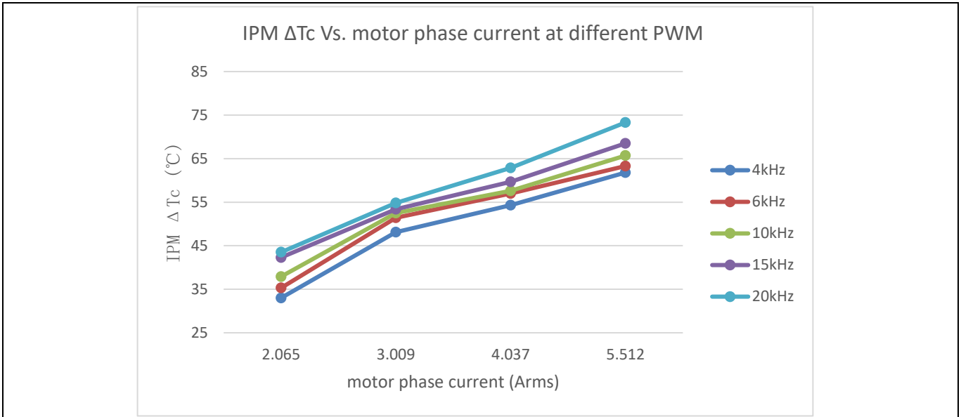
Figure 24 IPM \Delta T_c Vs. motor phase current at different PWM
