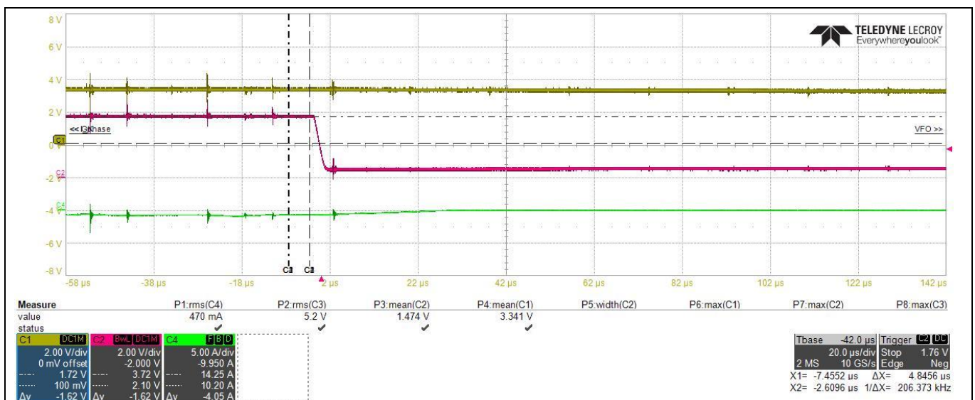
Figure 33 Hardware over-temperature protection
