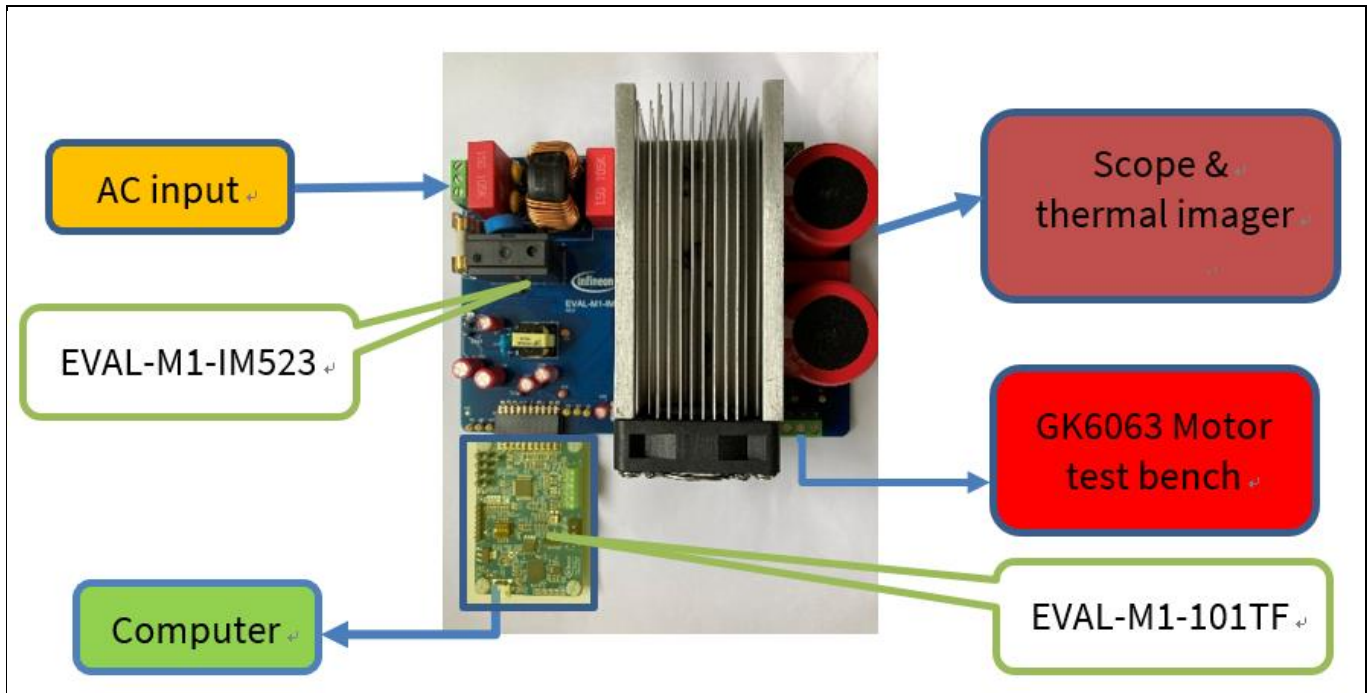
Figure 3 The functional groups of the EVAL-M1-IM523 evaluation design
