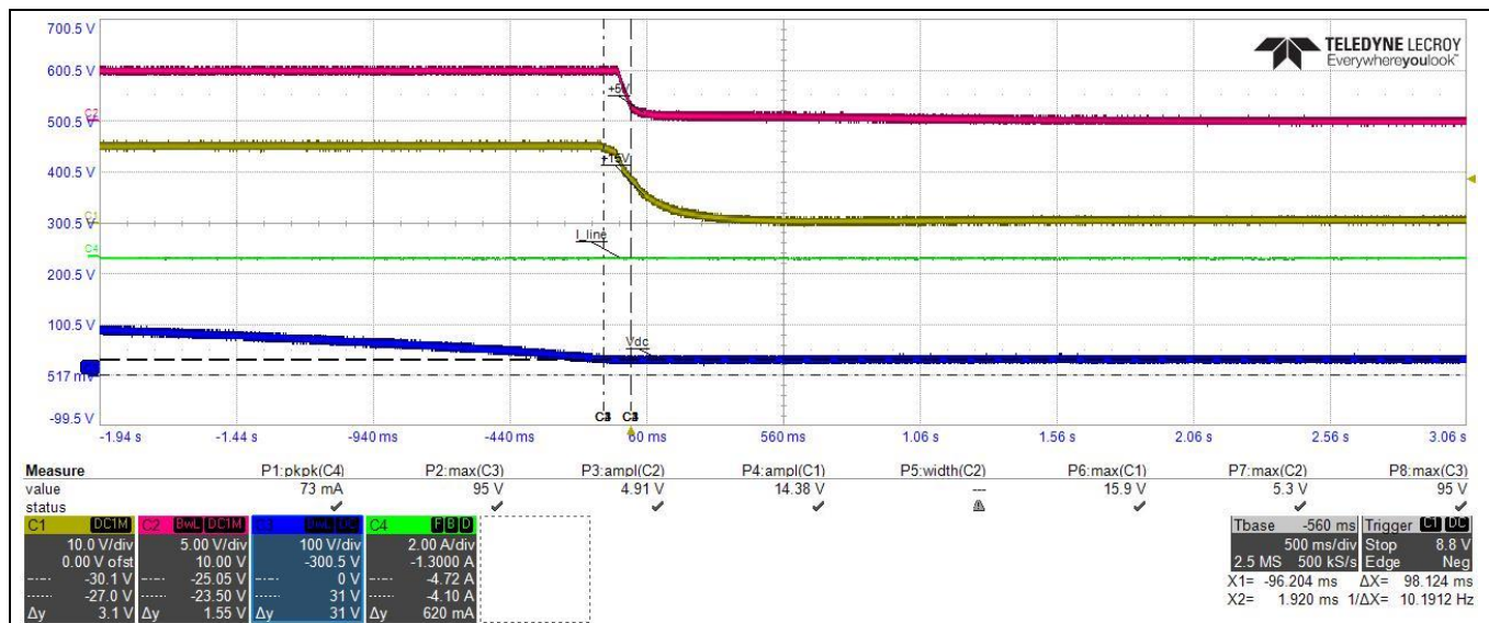
Figure 21 Input 255 V AC
