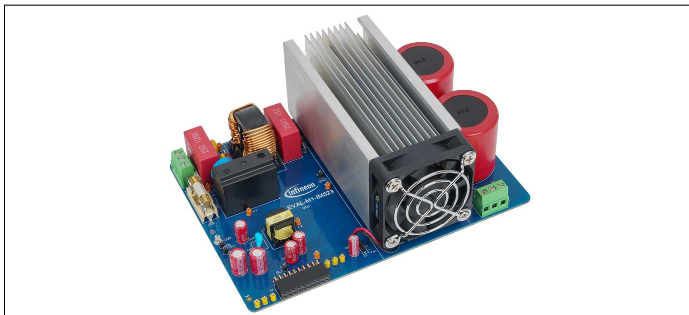
Figure 1 The iMotion™ MADK evaluation board for IM523-X6A CIPOS™ Mini IPM
