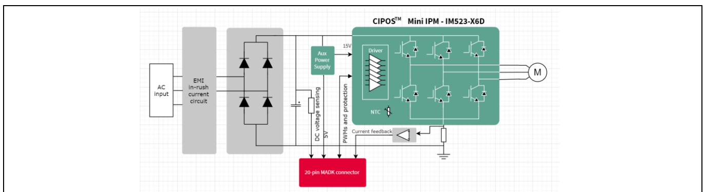
Figure 2 Block diagram of the EVAL-M1-IM523 evaluation board
