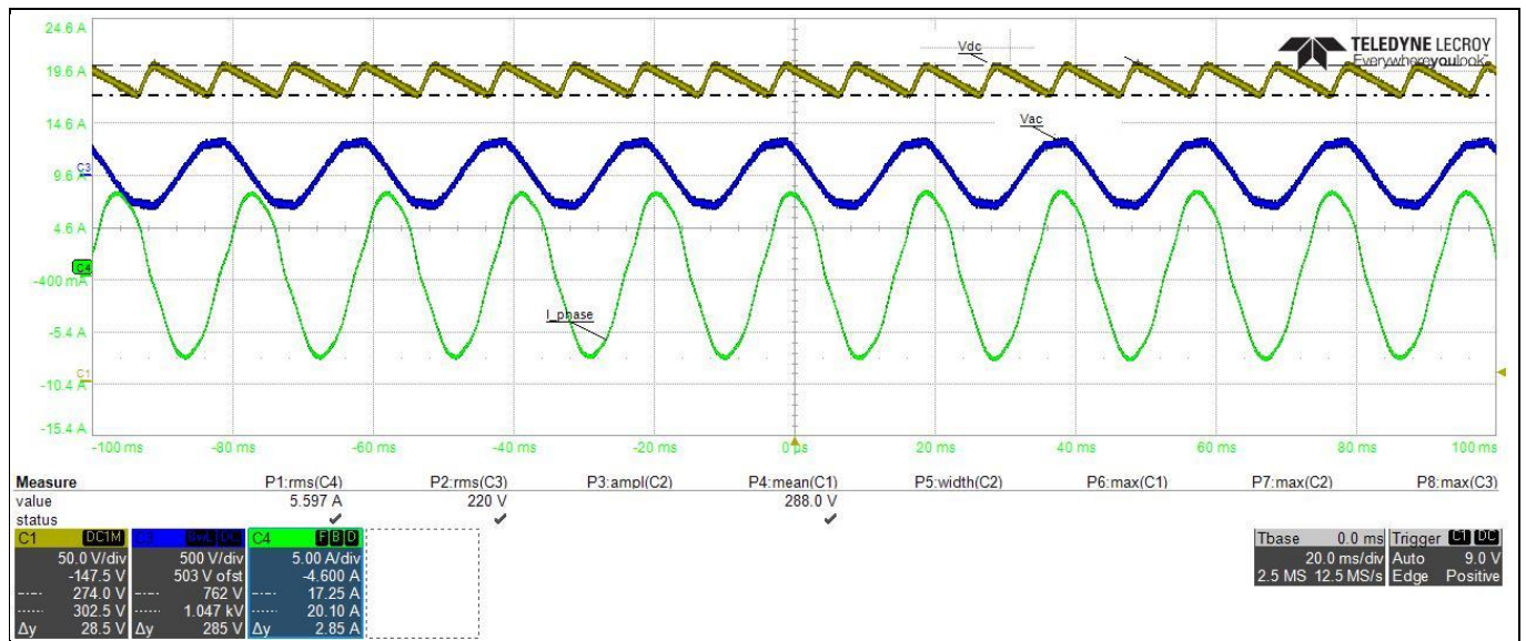
Figure 28 Scope waveform at 220 V AC input, 15 kHz PWM and 900 W output
