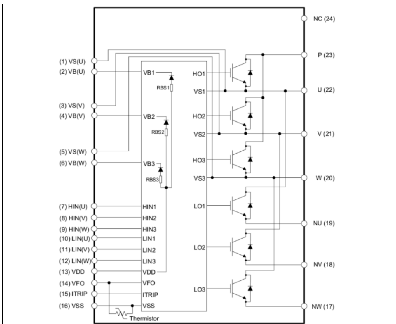
Figure 11 Internal block of the IM523-X6A
