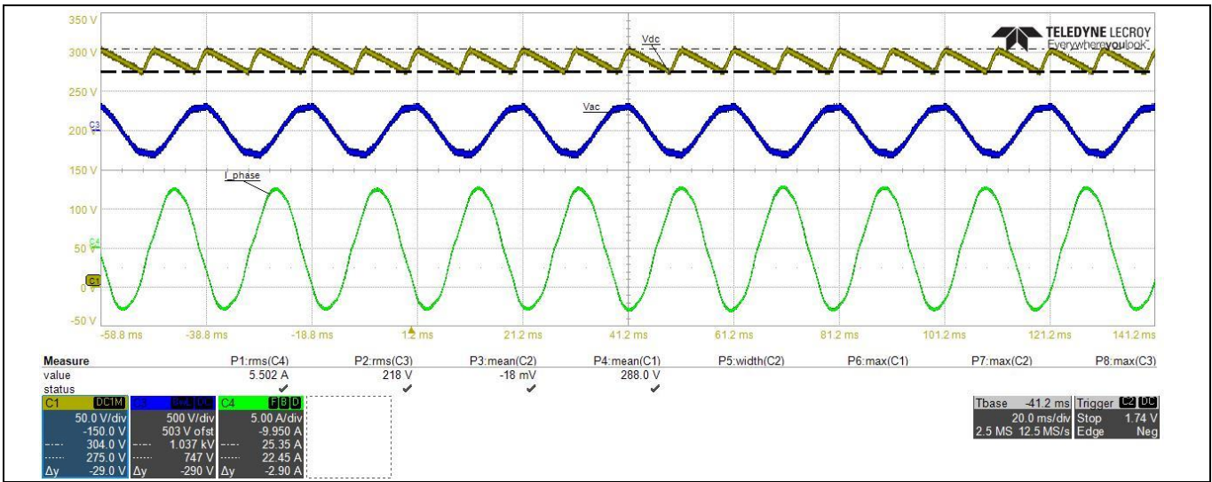
Figure 39 Scope waveforms at 930 W load, 5.5 A rms phase current, 15 kHz PWM, 220 V AC input
