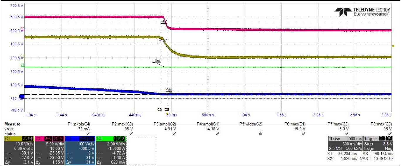
Figure 18 Auxiliary power supply browns out
