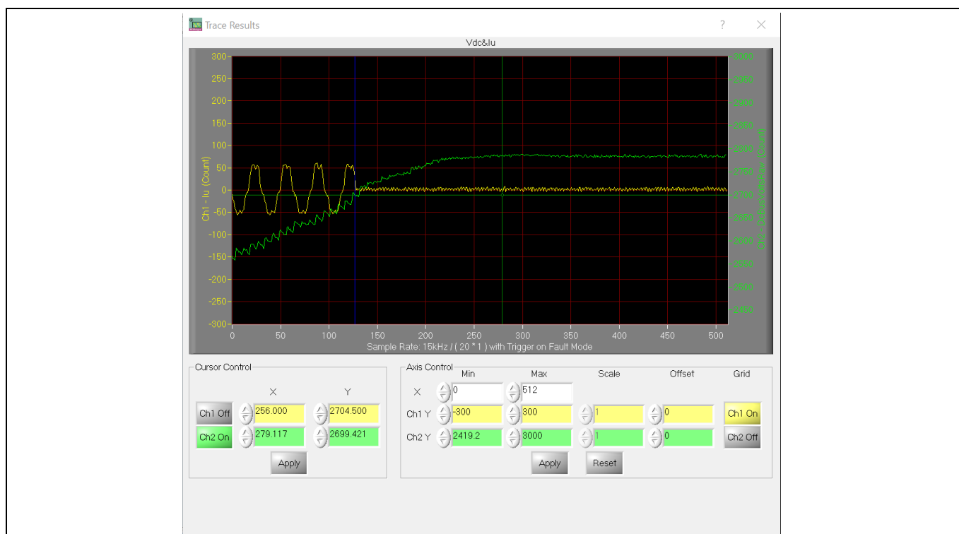
Figure 30 OV protection
