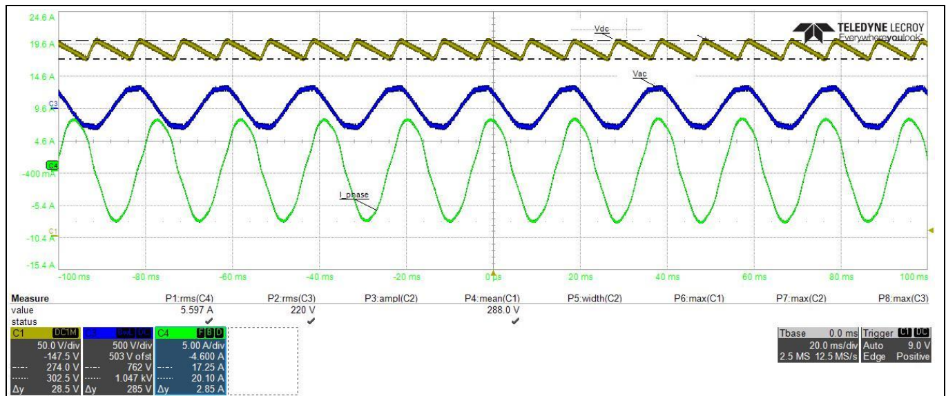
Figure 22 220 V AC input, V DC bus voltage ripple
