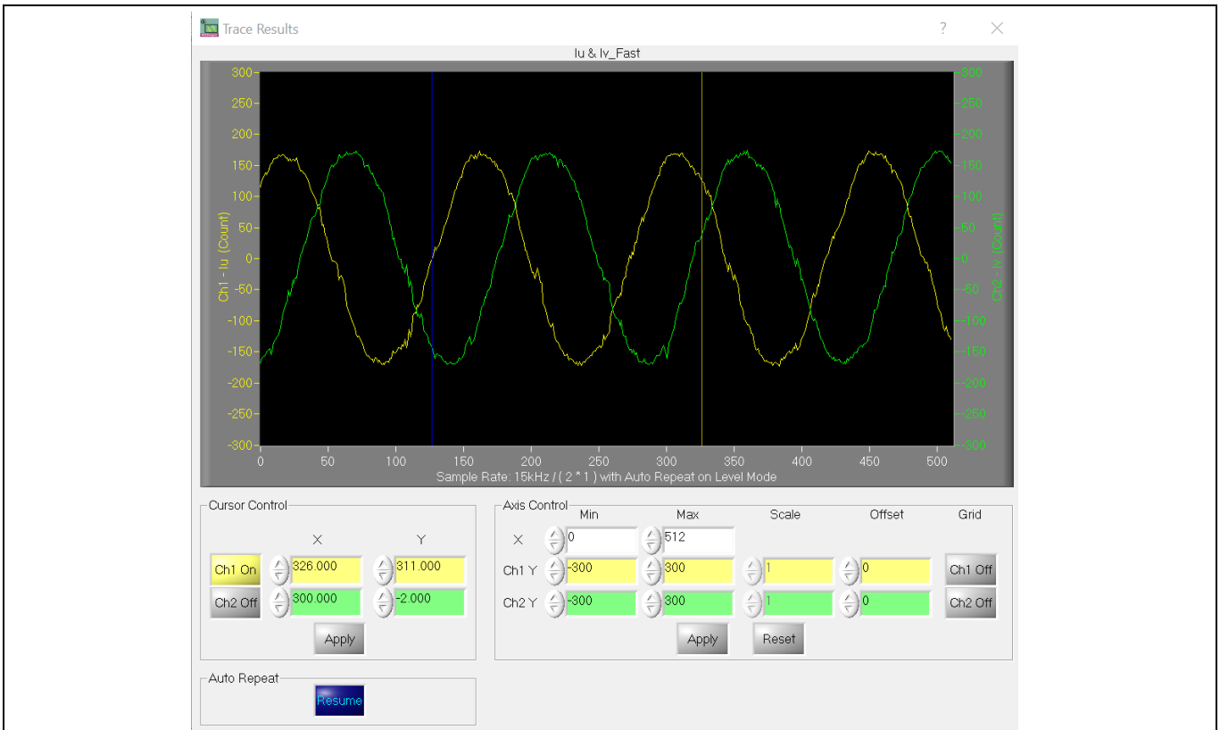
Figure 38 930 W load, 5.5 A rms phase current, 15 kHz PWM, 220 V AC input
