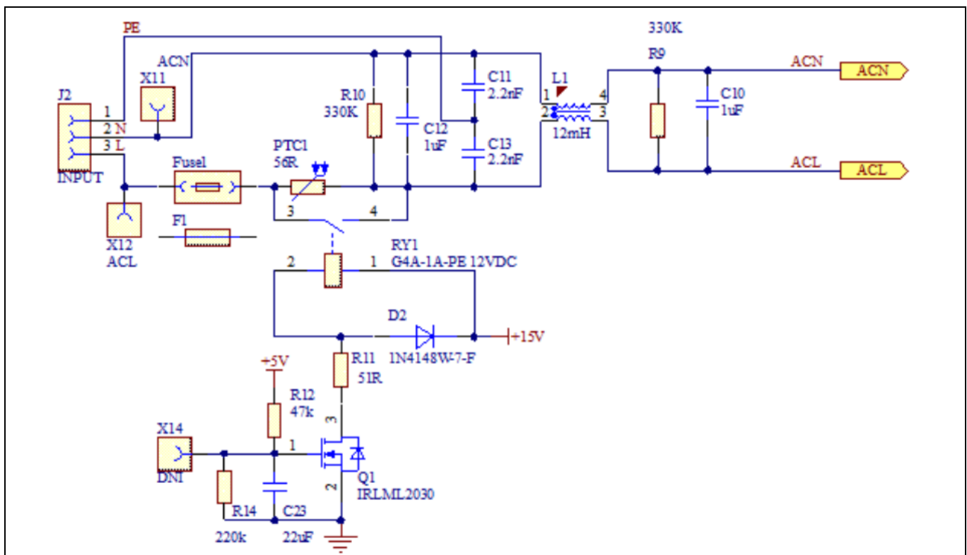
Figure 12 Schematics for EMI filter and a soft power-up circuit
