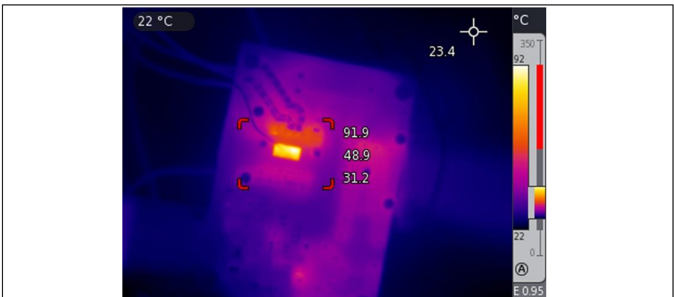
Figure 27 Thermal test at 220 V AC input, 15 kHz PWM and 900 W output
