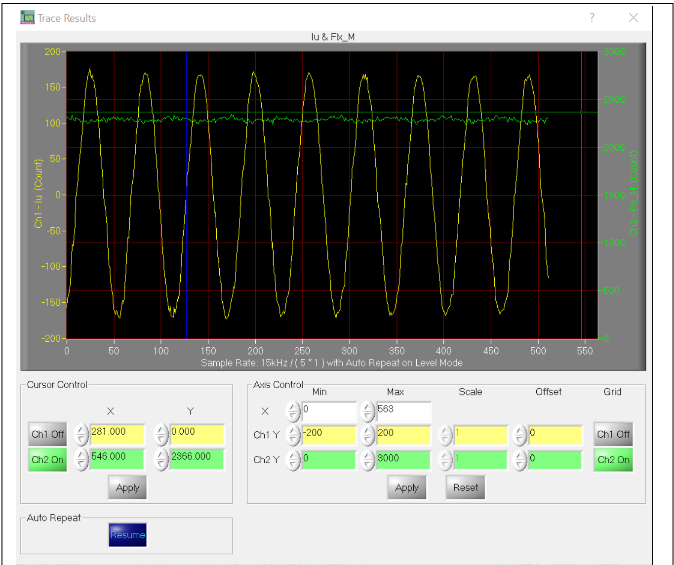
Figure 40 Flx_M & Iu waveform in MCEDesigner
