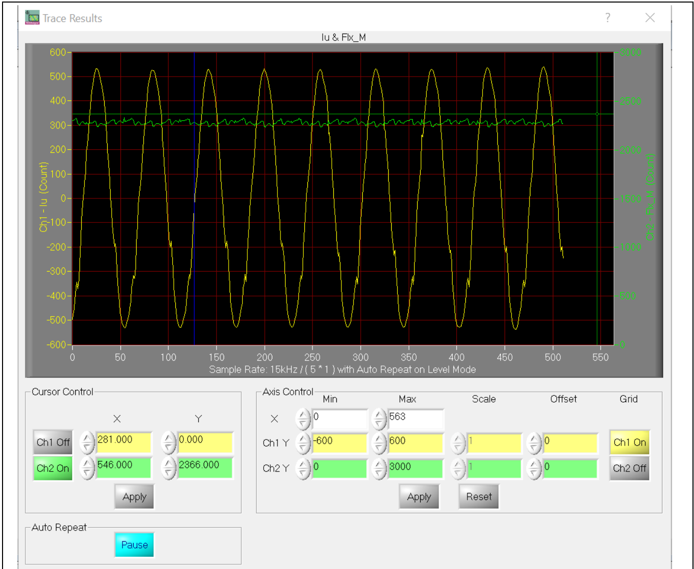
Figure 26 I_u & Flx\_M at 15 kHz PWM, 220 V AC input, 900 W output (5.5 A rms phase current)
