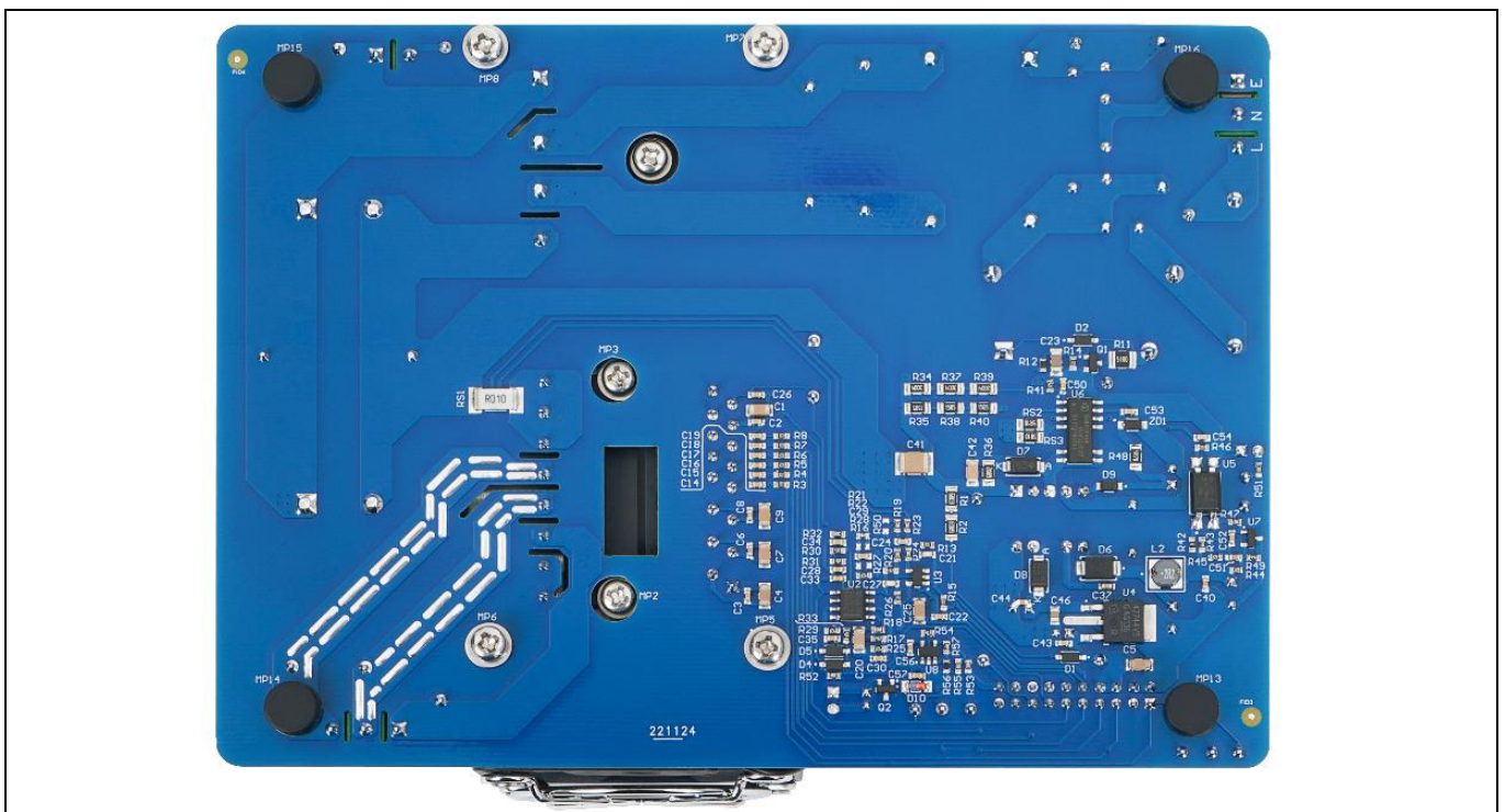
Figure 16 Bottom-assembly PCBA of the EVAL-M1-IM523
