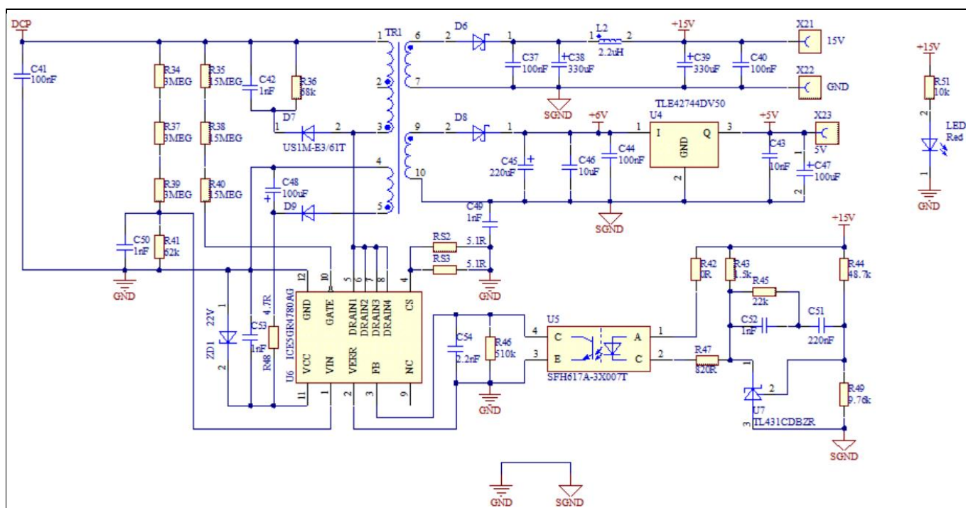
Figure 14 Auxiliary power supply of the EVAL-M1-IM523
