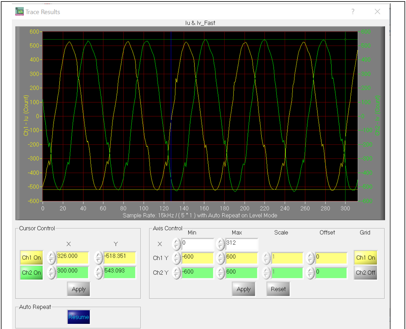
Figure 25 Iu & Flx_M at 15 kHz PWM, 220 V AC input, 900 W output (5.5 A rms phase current)
