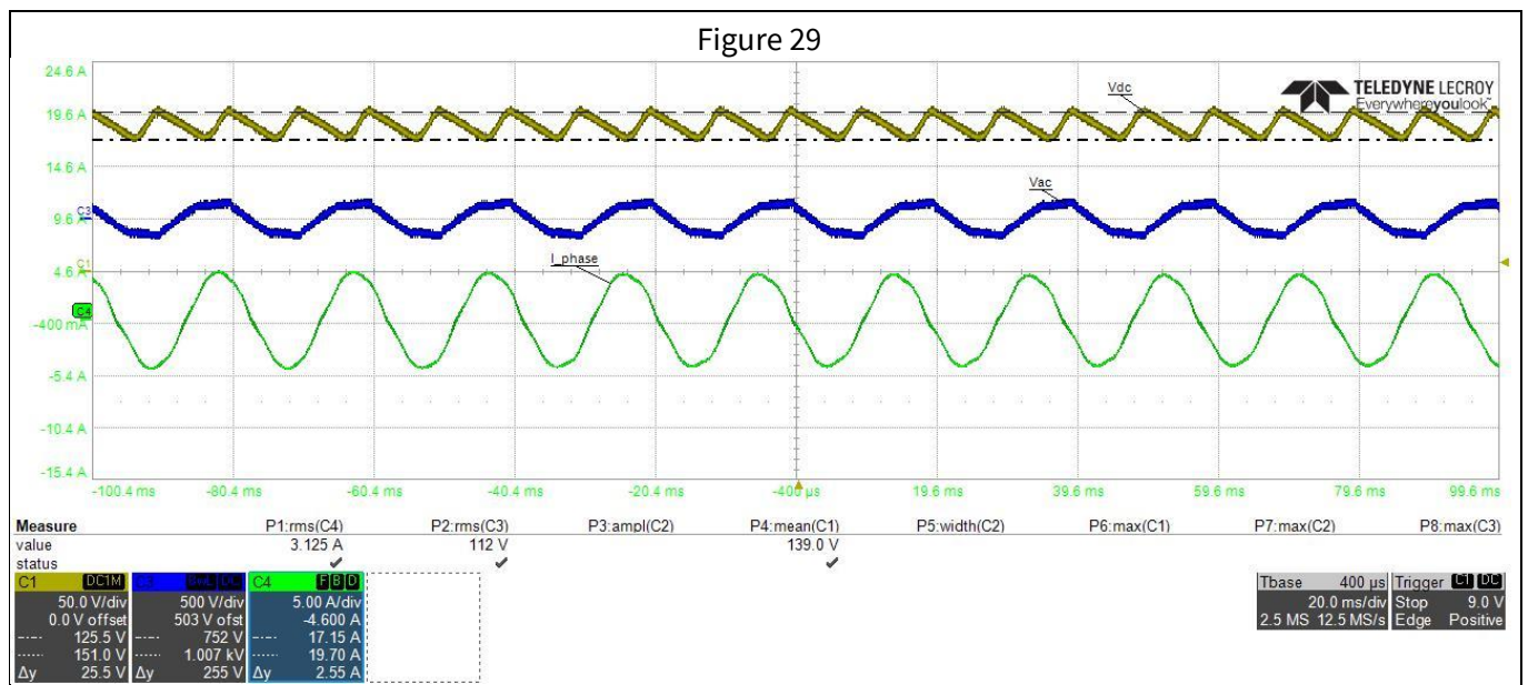
Figure 29 Scope waveform at 110 V AC input, 500 W output power, and 15 kHz PWM
