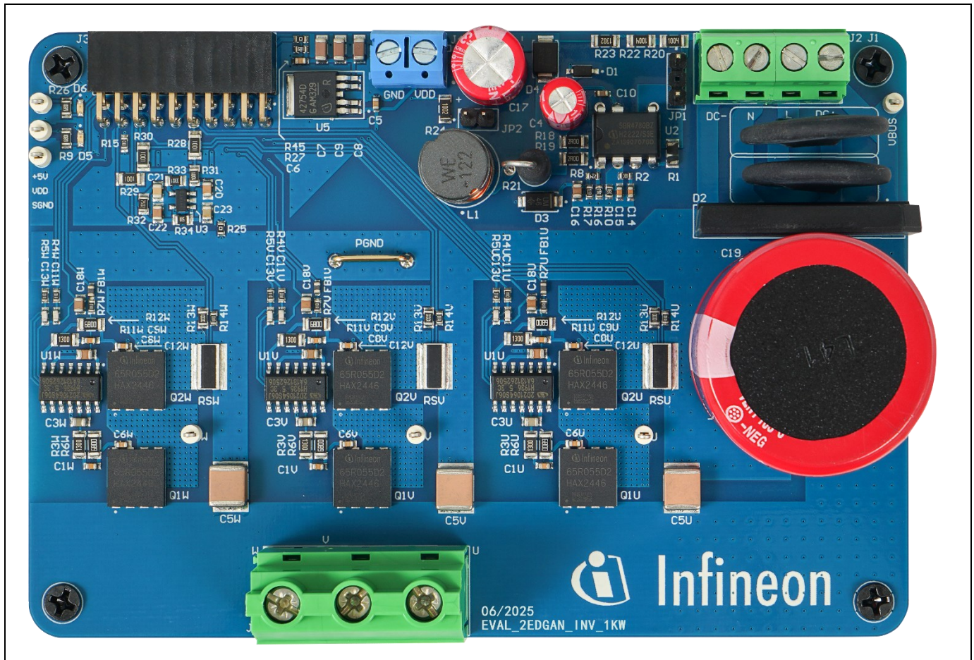
Figure 1 Evaluation Board EVAL-2EDGAN-INV-1KW
