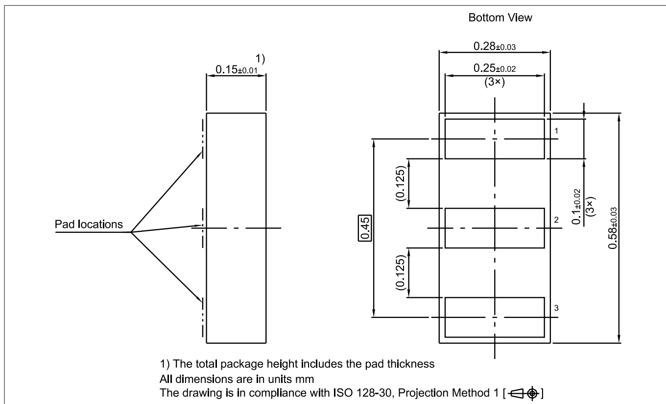
Figure 11 WLL-3-1 package
