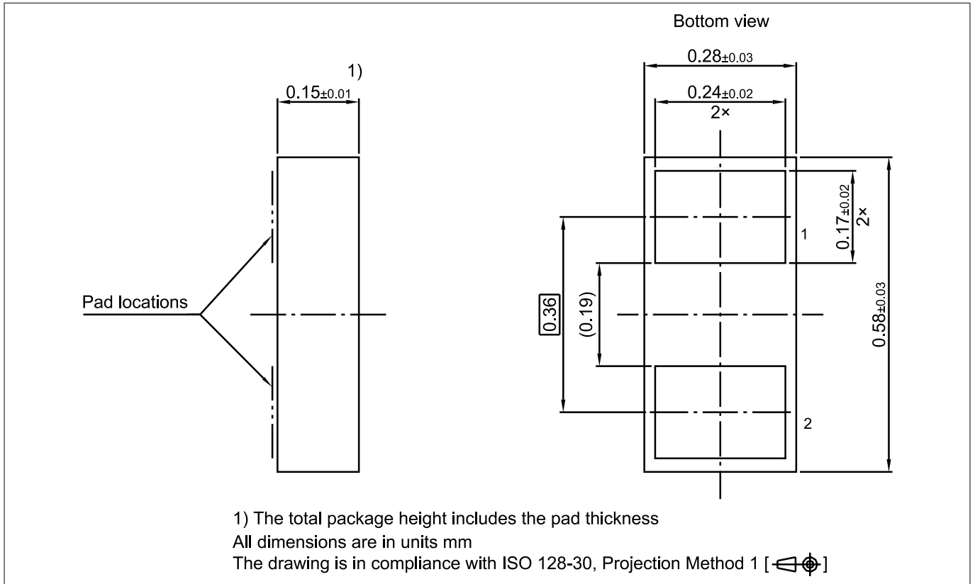
Figure 13 WLL-2-3 package
